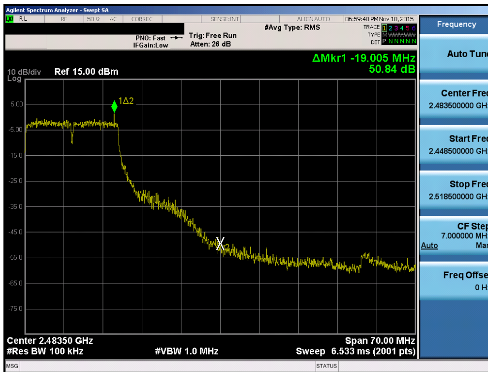
Plot 7-23. Band Edge Plot (802.11g – Ch. 10)
