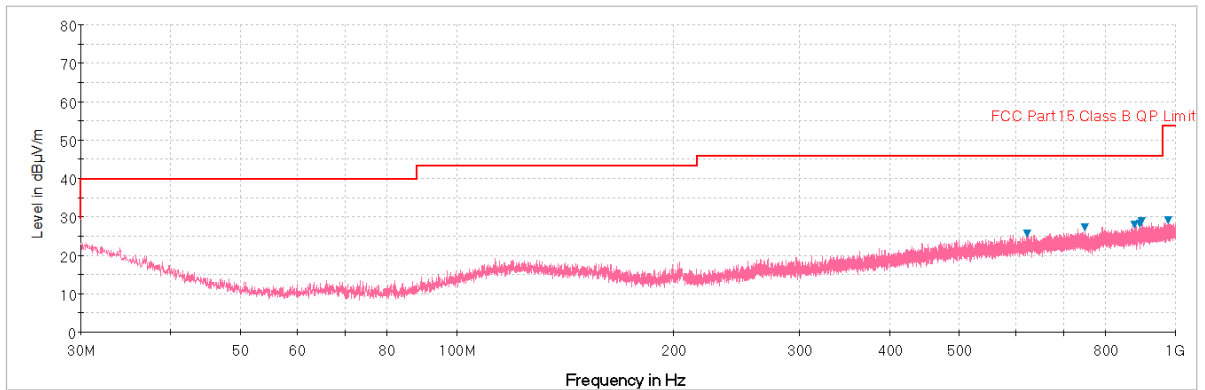
Plot 7-51. Radiated Spurious Plot below 1GHz (Pol. H)
