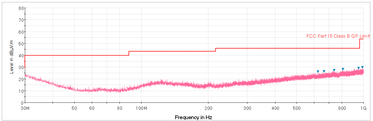
Plot 7-52. Radiated Spurious Plot below 1GHz (Pol. V)
