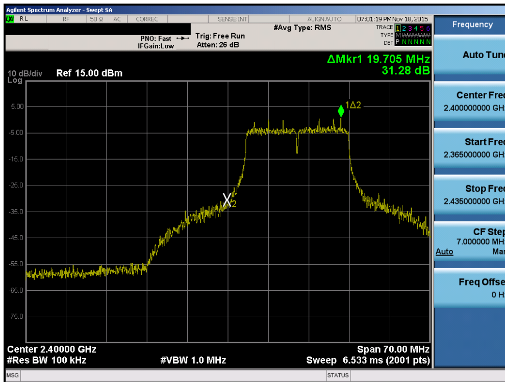
Plot 7-25. Band Edge Plot (802.11n (2.4GHz) – Ch. 1)
