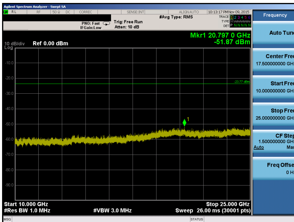
Plot 7-34. Conducted Spurious Plot (802.11b – Ch. 11)
