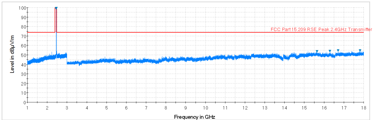
Plot 7-40. Radiated Spurious Plot above 1GHz (802.11b – Ch. 11, Ant. Pol. V)
