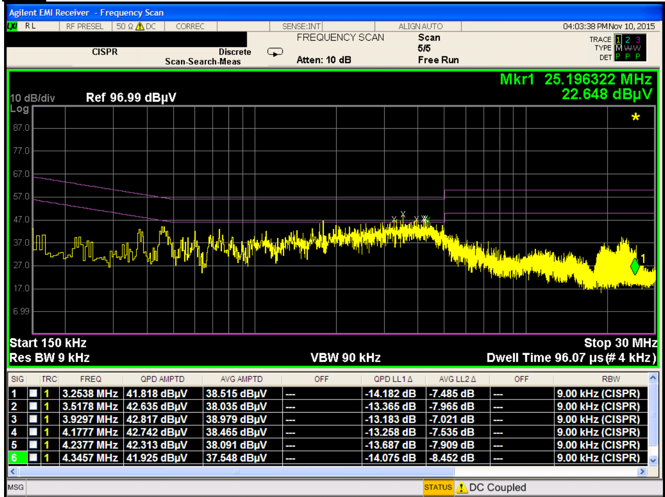
Plot 7-54. Line Conducted Plot with 802.11b (N)
