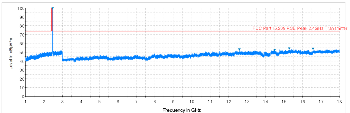
Plot 7-39. Radiated Spurious Plot above 1GHz (802.11b – Ch. 11, Ant. Pol. H)
