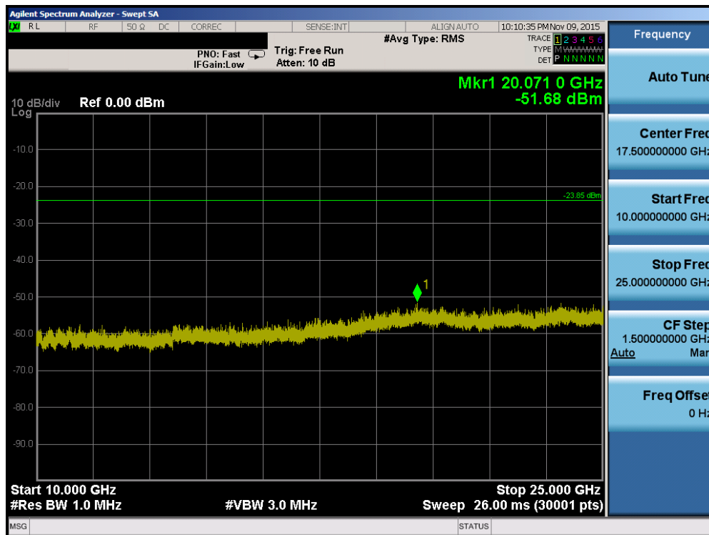
Plot 7-30. Conducted Spurious Plot (802.11b – Ch. 1)
