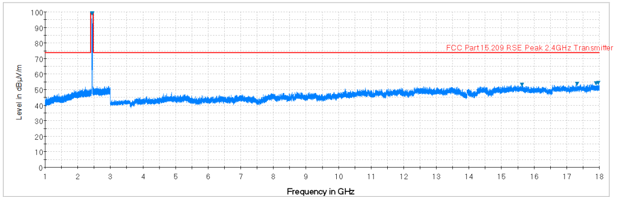
Plot 7-38. Radiated Spurious Plot above 1GHz (802.11b – Ch. 6, Ant. Pol. V)
