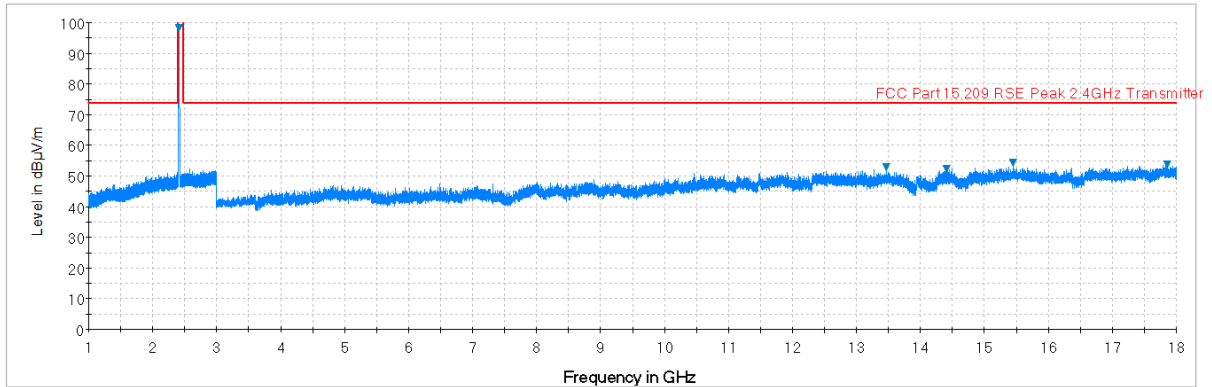
Plot 7-35. Radiated Spurious Plot above 1GHz (802.11b – Ch. 1, Ant. Pol. H)
