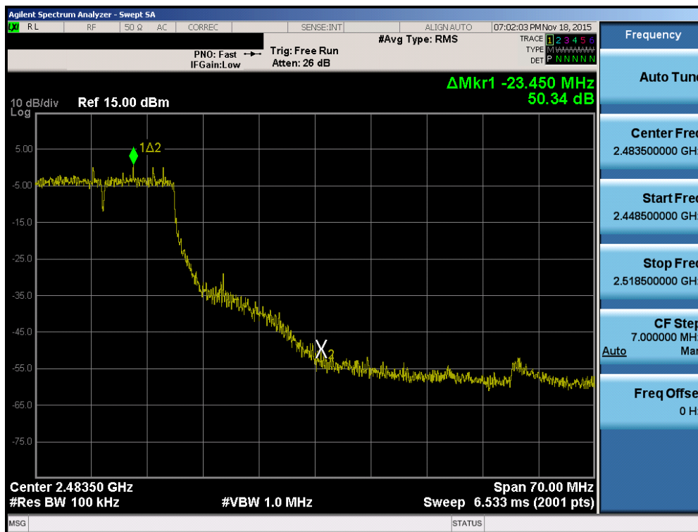
Plot 7-27. Band Edge Plot (802.11n (2.4GHz) – Ch. 10)
