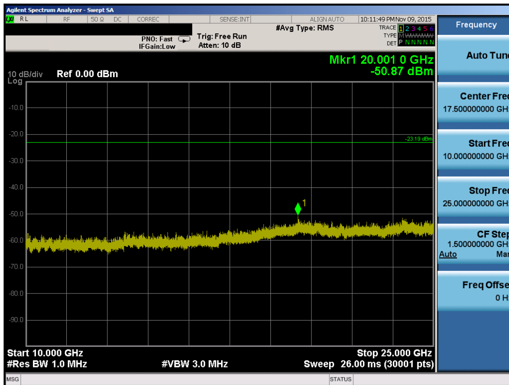
Plot 7-32. Conducted Spurious Plot (802.11b – Ch. 6)
