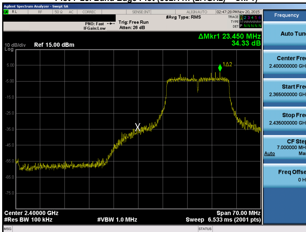
Plot 7-26. Band Edge Plot (802.11n (2.4GHz) – Ch. 2)
