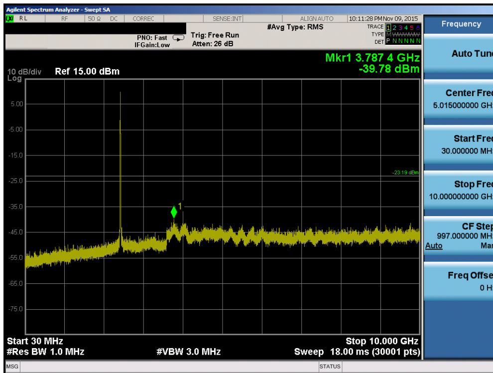
Plot 7-31. Conducted Spurious Plot (802.11b – Ch. 6)
