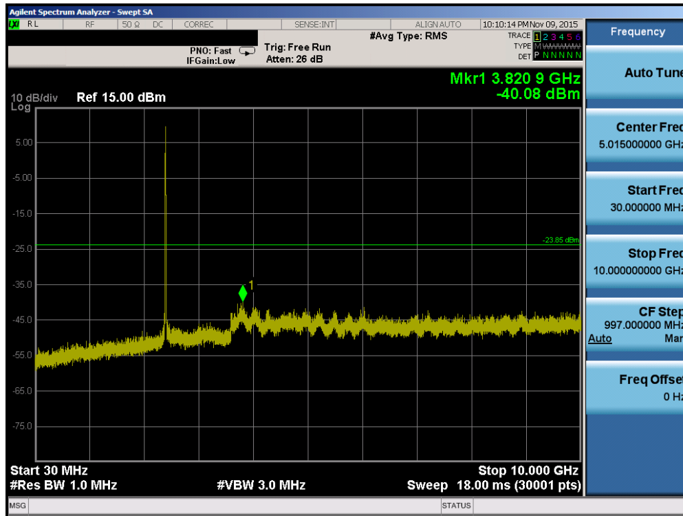
Plot 7-29. Conducted Spurious Plot (802.11b – Ch. 1)
