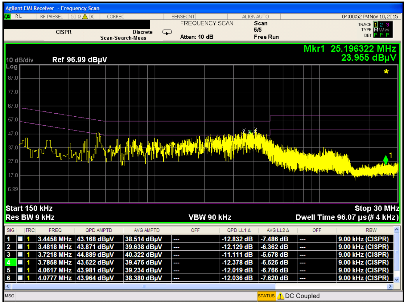
Plot 7-53. Line Conducted Plot with 802.11b (L1)
