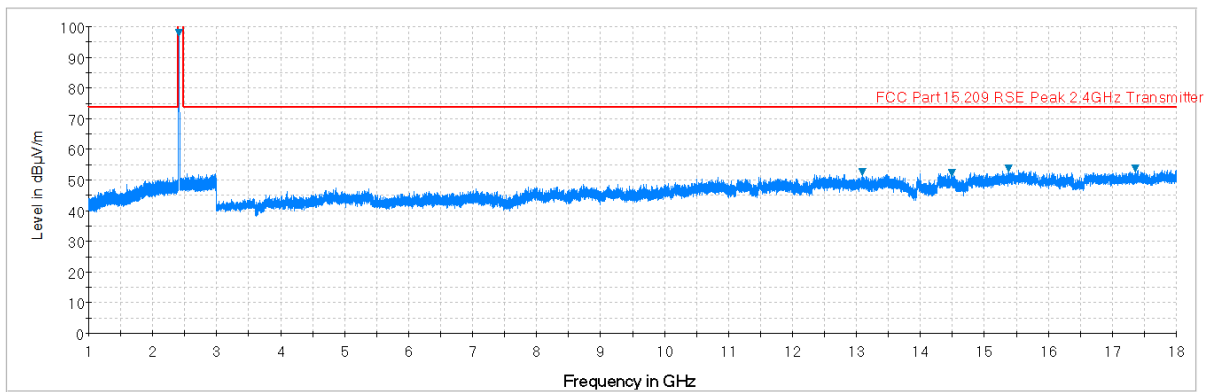
Plot 7-36. Radiated Spurious Plot above 1GHz (802.11b – Ch. 1, Ant. Pol. V)
