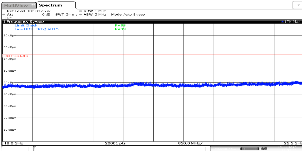
Plot 7-42. Radiated Spurious Plot above 18GHz (Pol. V)
