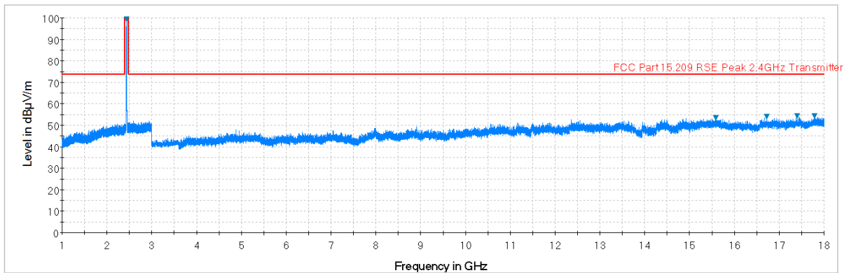
Plot 7-37. Radiated Spurious Plot above 1GHz (802.11b – Ch. 6, Ant. Pol. H)
