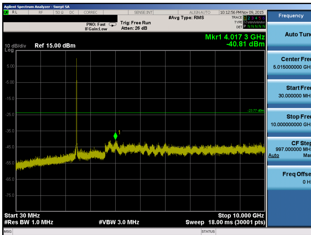
Plot 7-33. Conducted Spurious Plot (802.11b – Ch. 11)
