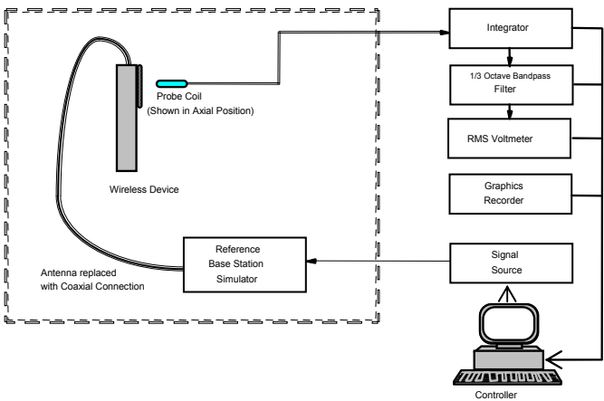
Figure 4-13 Audio Magnetic Field Test Setup
