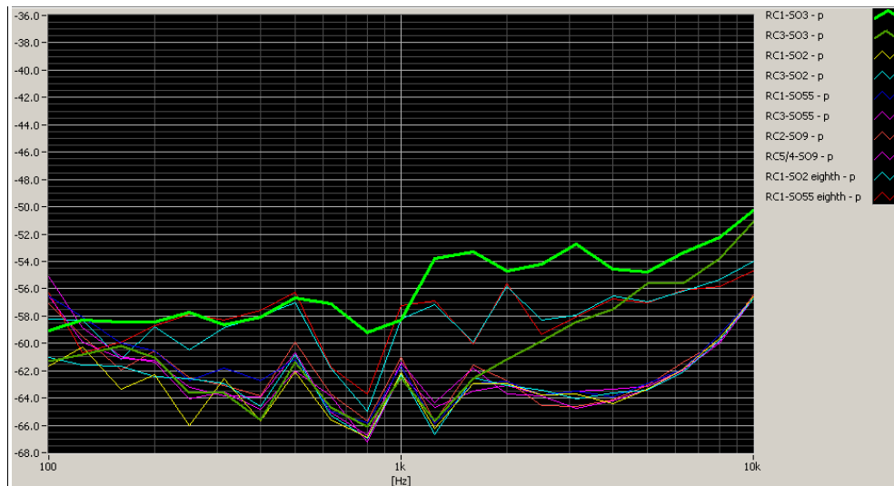
Figure 5-1 CDMA Audio Band Magnetic Noise
