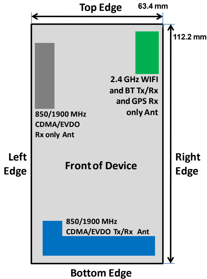
Figure F-3 DUT Antenna Locations
