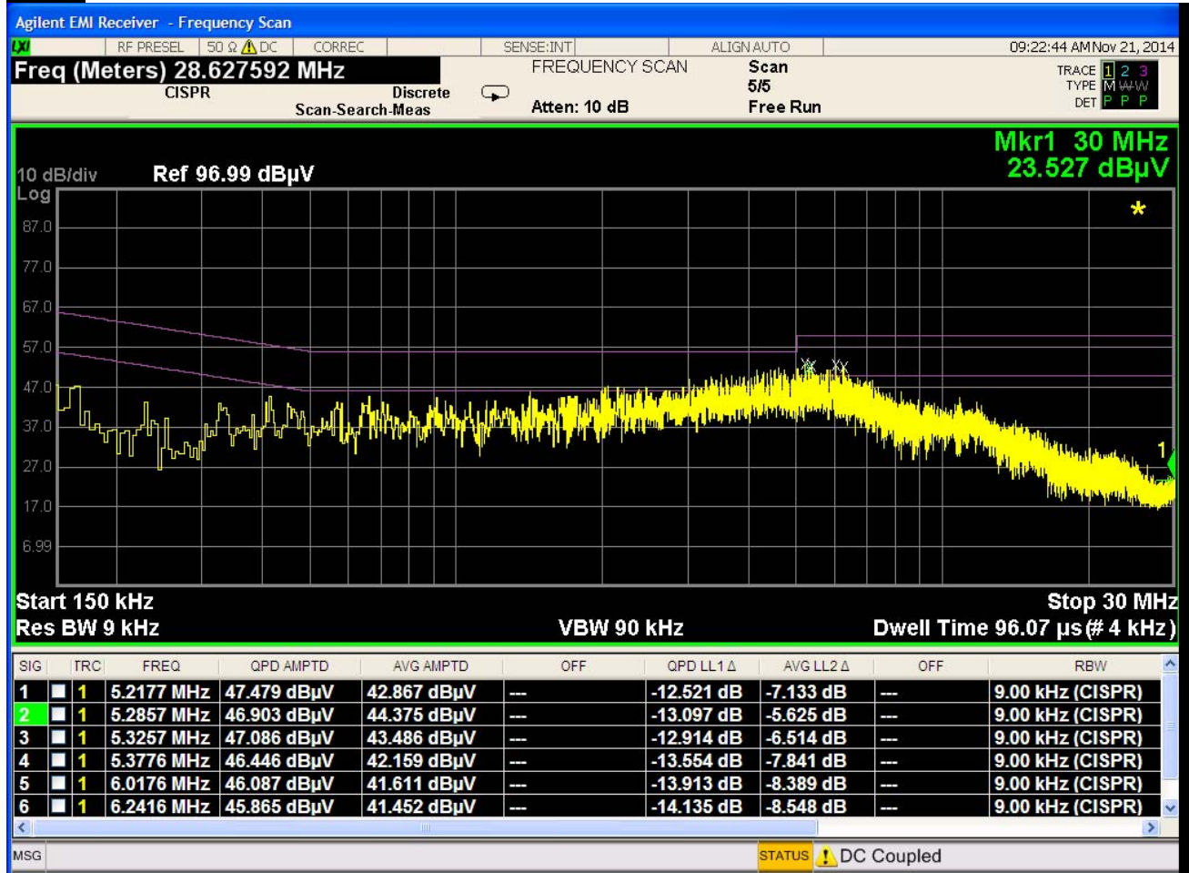
Plot 6-44. Line-Conducted Test Plot (L1)
