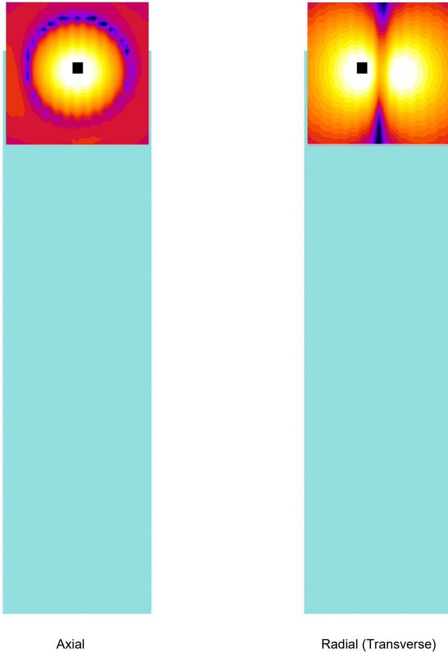
Figure 8-1 T-Coil Scan Overlay Magnetic Field Distributions
