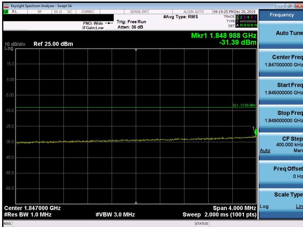
Plot 7-196. Lower Extended Band Edge Plot (Band 25/2 - 20.0MHz QPSK - Full RB Configuration)
