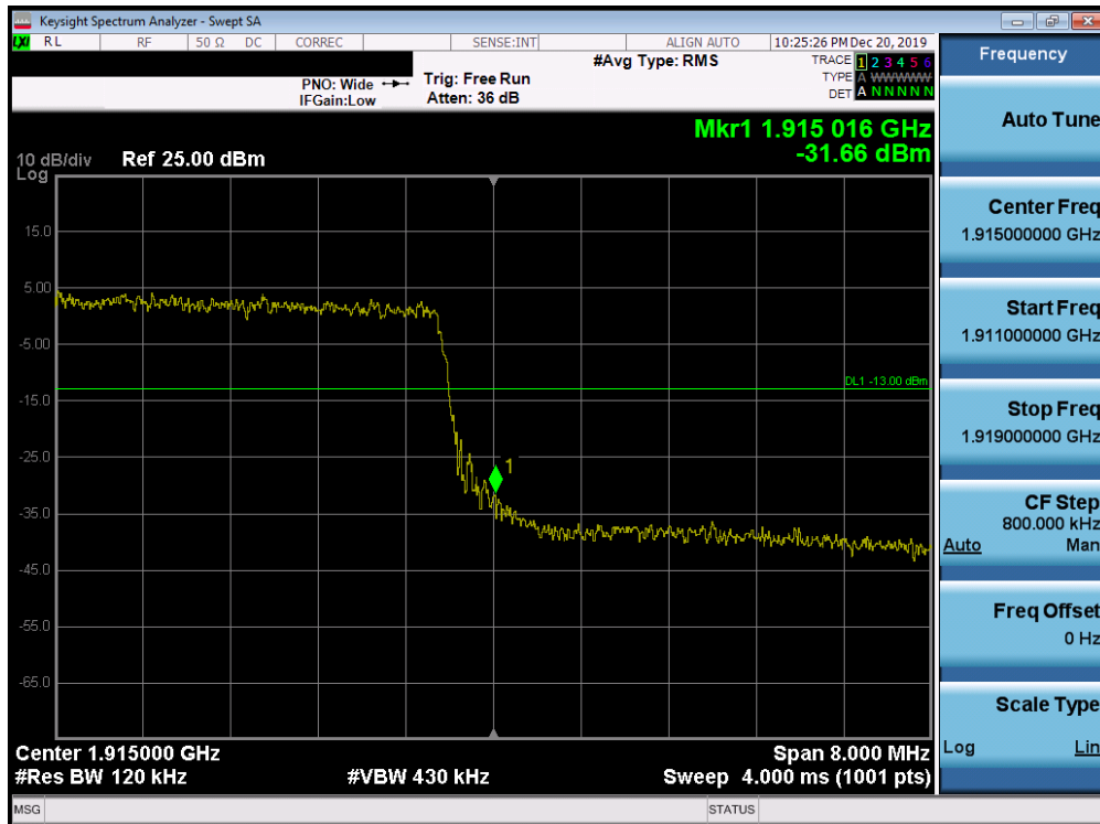
Plot 7-187. Upper Band Edge Plot (Band 25 - 10.0MHz QPSK - Full RB Configuration)
