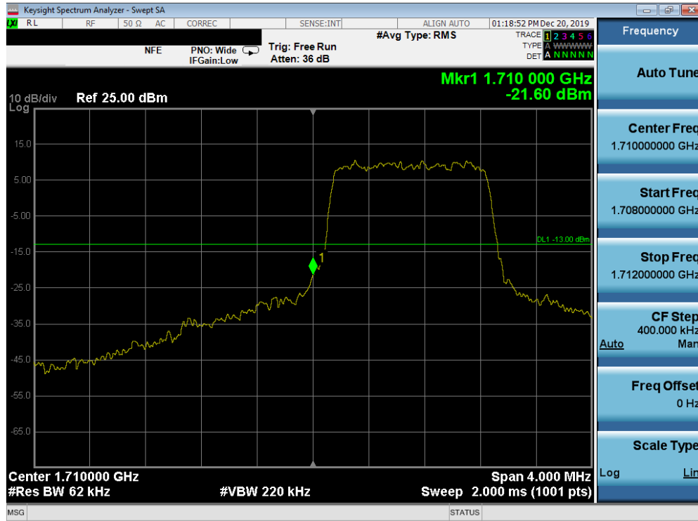
Plot 7-129. Lower Band Edge Plot (Band 66/4 - 1.4MHz QPSK - Full RB Configuration)
