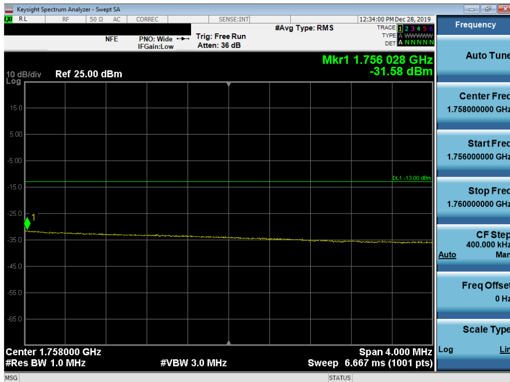
Plot 7-164. Upper Extended Band Edge Plot (Band 4 - 20.0MHz QPSK - Full RB Configuration)
