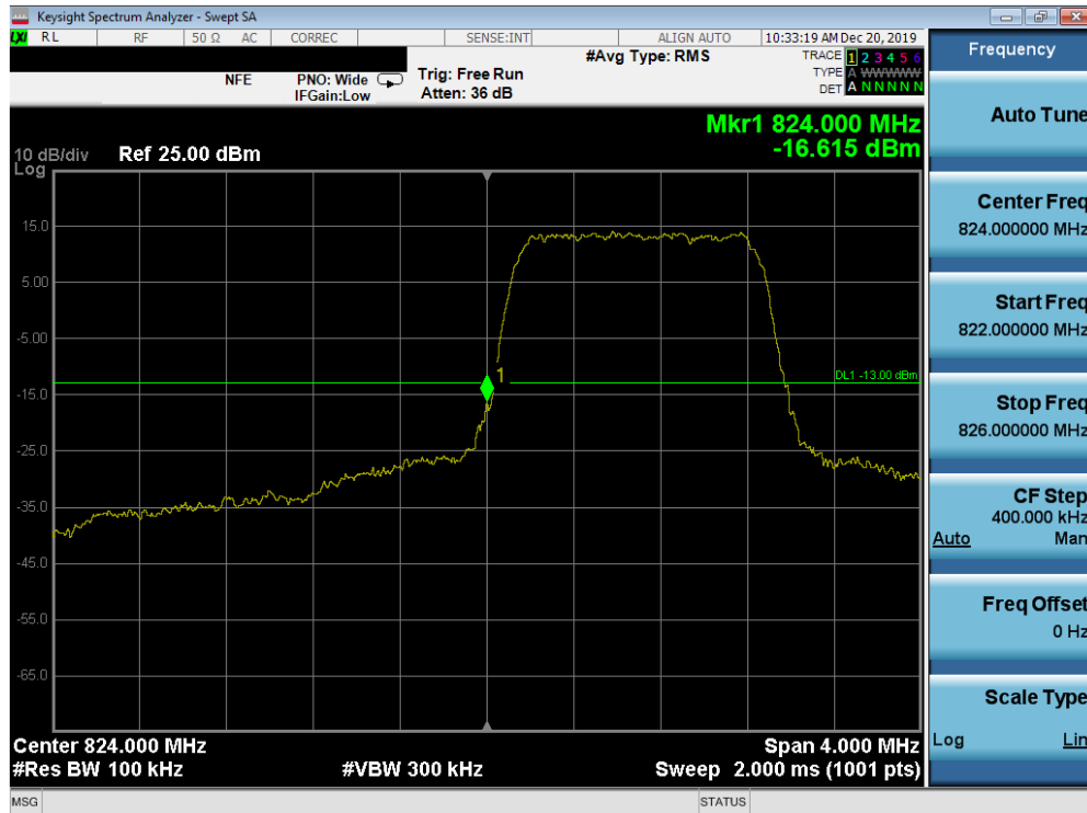
Plot 7-119. Lower Band Edge Plot (Band 26/5 - 1.4MHz QPSK - Full RB Configuration)
