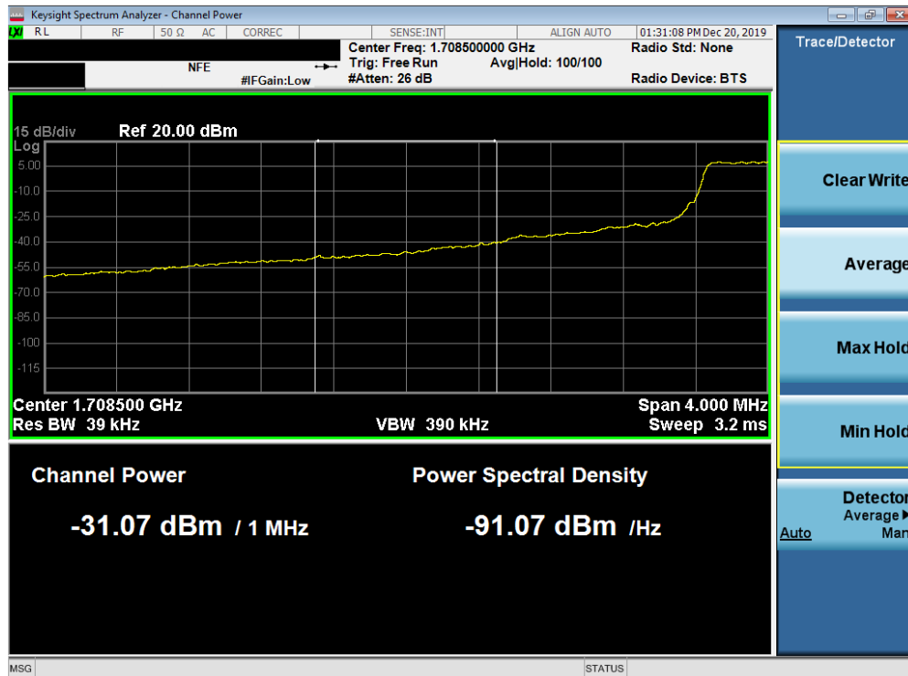
Plot 7-130. Lower Extended Band Edge Plot (Band 66/4 - 1.4MHz QPSK - Full RB Configuration)
