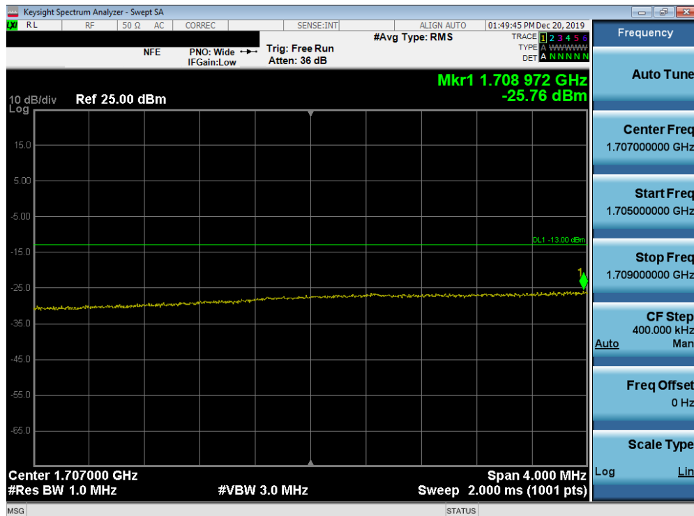
Plot 7-154. Lower Extended Band Edge Plot (Band 66/4 - 15.0MHz QPSK - Full RB Configuration)
