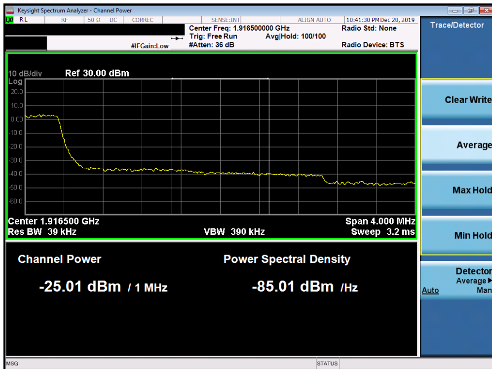
Plot 7-176. Upper Extended Band Edge Plot (Band 25 - 3.0MHz QPSK - Full RB Configuration)
