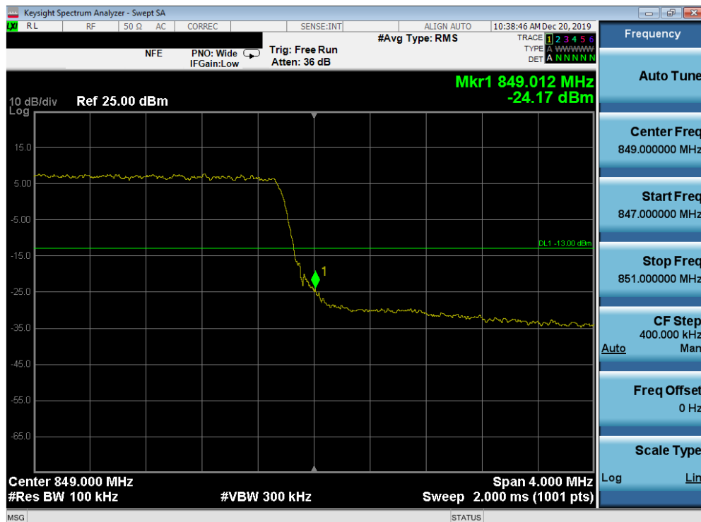
Plot 7-124. Upper Band Edge Plot (Band 26/5 - 5.0MHz QPSK - Full RB Configuration)
