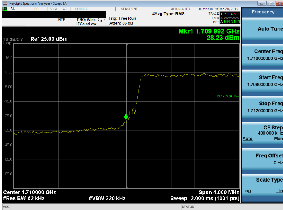
Plot 7-141. Lower Band Edge Plot (Band 66/4 - 5.0MHz QPSK - Full RB Configuration)
