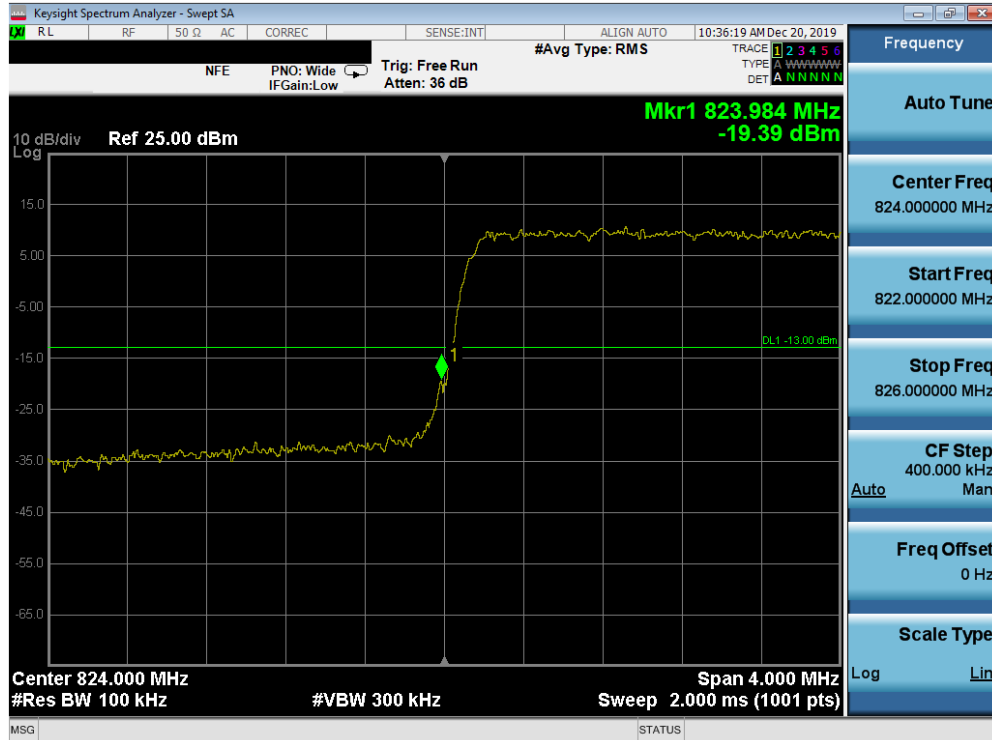
Plot 7-121. Lower Band Edge Plot (Band 26/5 - 3.0MHz QPSK - Full RB Configuration)
