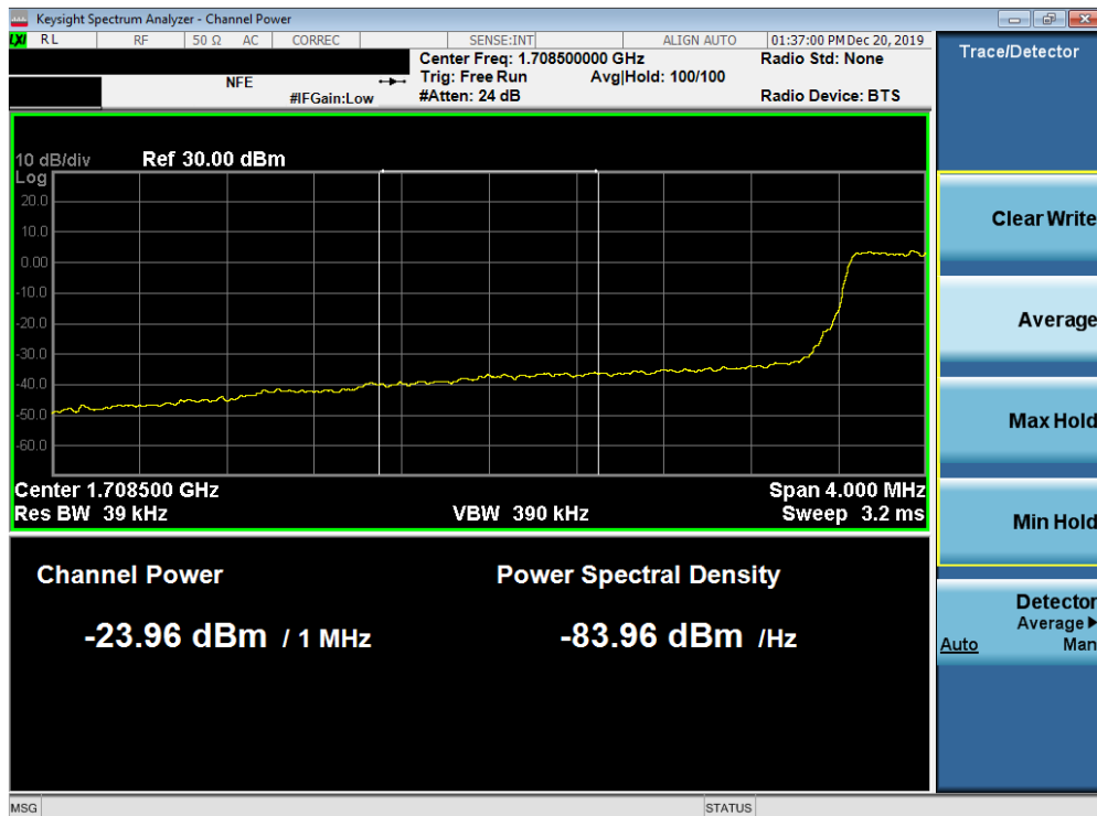
Plot 7-136. Lower Extended Band Edge Plot (Band 66/4 - 3.0MHz QPSK - Full RB Configuration)
