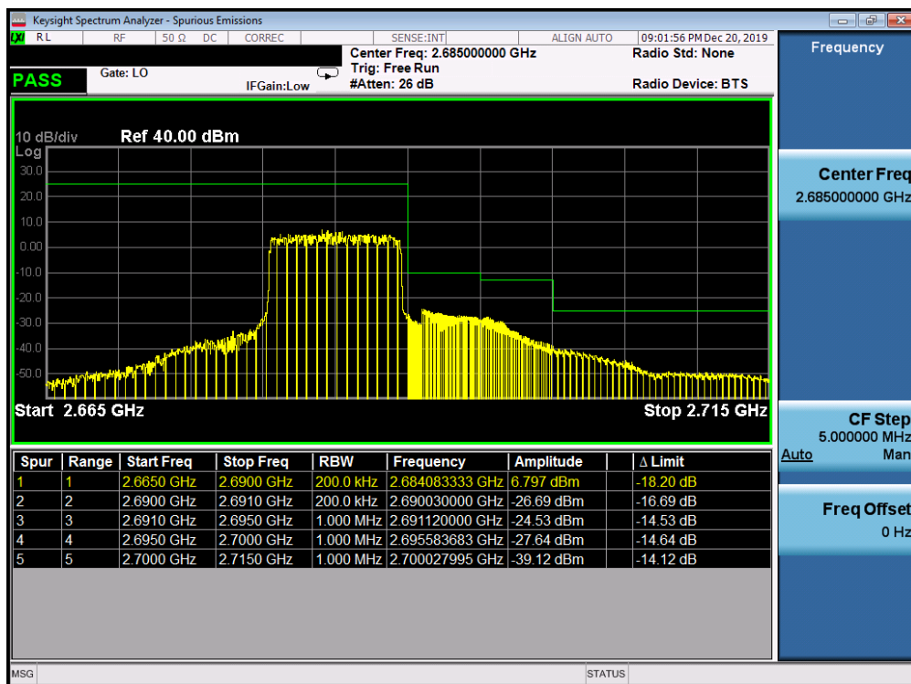
Plot 7-204. Upper ACP Plot (Band 41 PC3 - 10.0MHz QPSK - Full RB Configuration)
