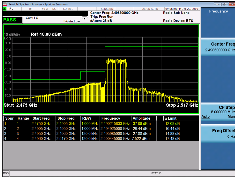
Plot 7-201. Lower ACP Plot at 2496 MHz (Band 41 PC3 - 5.0MHz QPSK - Full RB Configuration)
