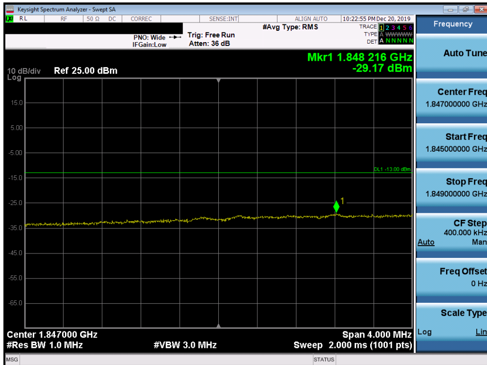
Plot 7-190. Lower Extended Band Edge Plot (Band 25/2 - 15.0MHz QPSK - Full RB Configuration)
