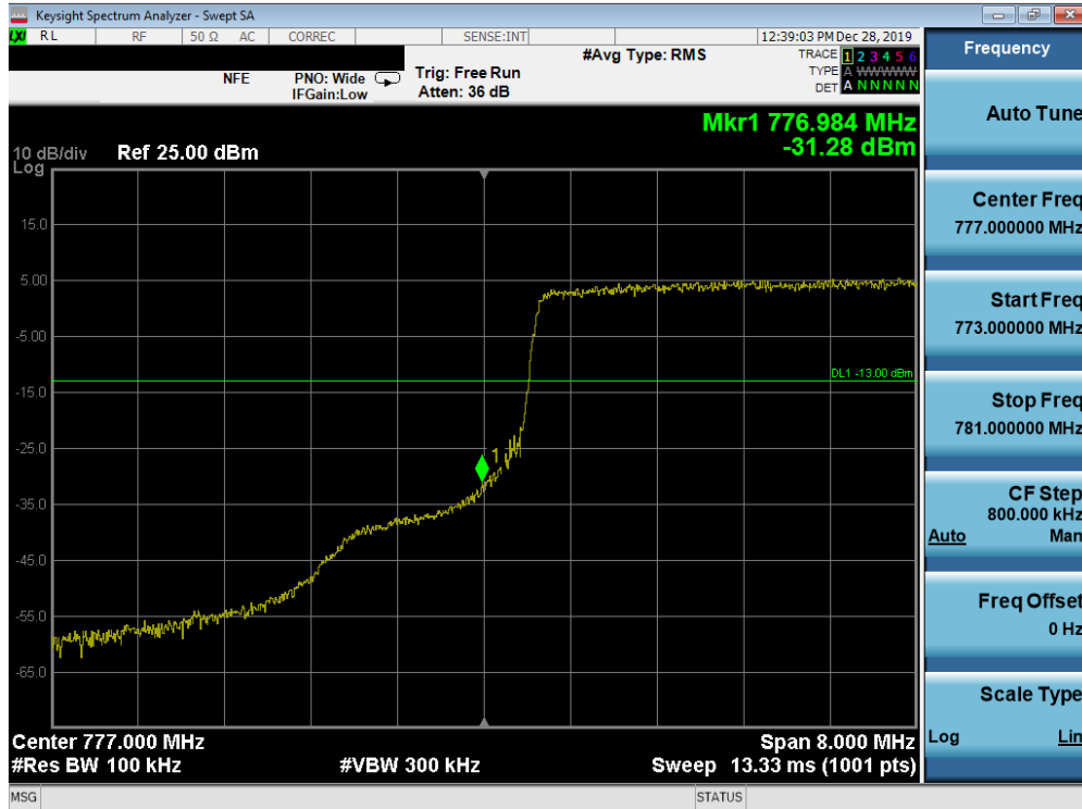
Plot 7-115. Lower Band Edge Plot (Band 13 - 10MHz QPSK - Full RB Configuration)
