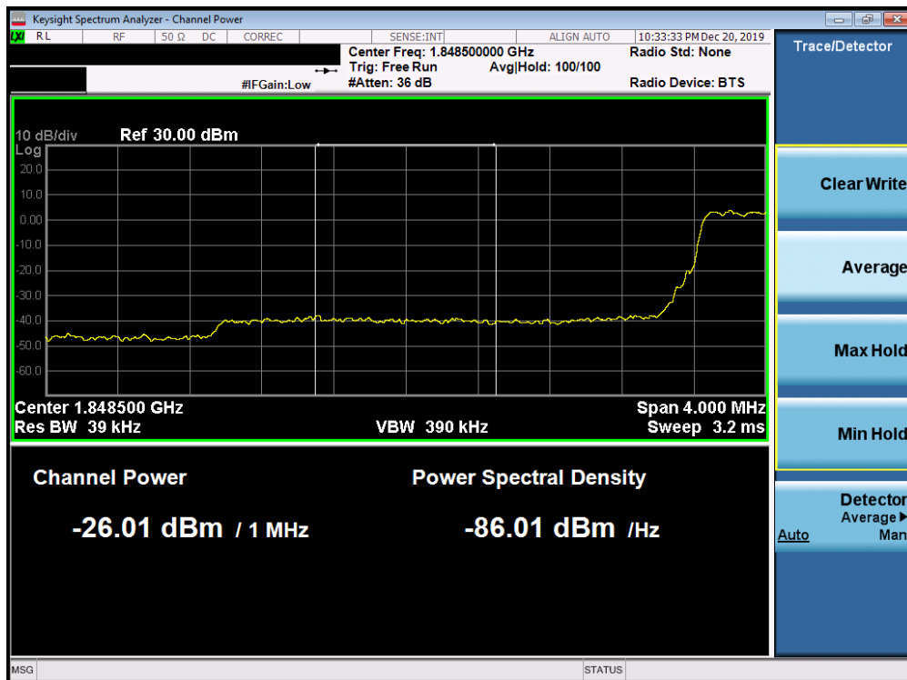
Plot 7-172. Lower Extended Band Edge Plot (Band 25/2 - 3.0MHz QPSK - Full RB Configuration)
