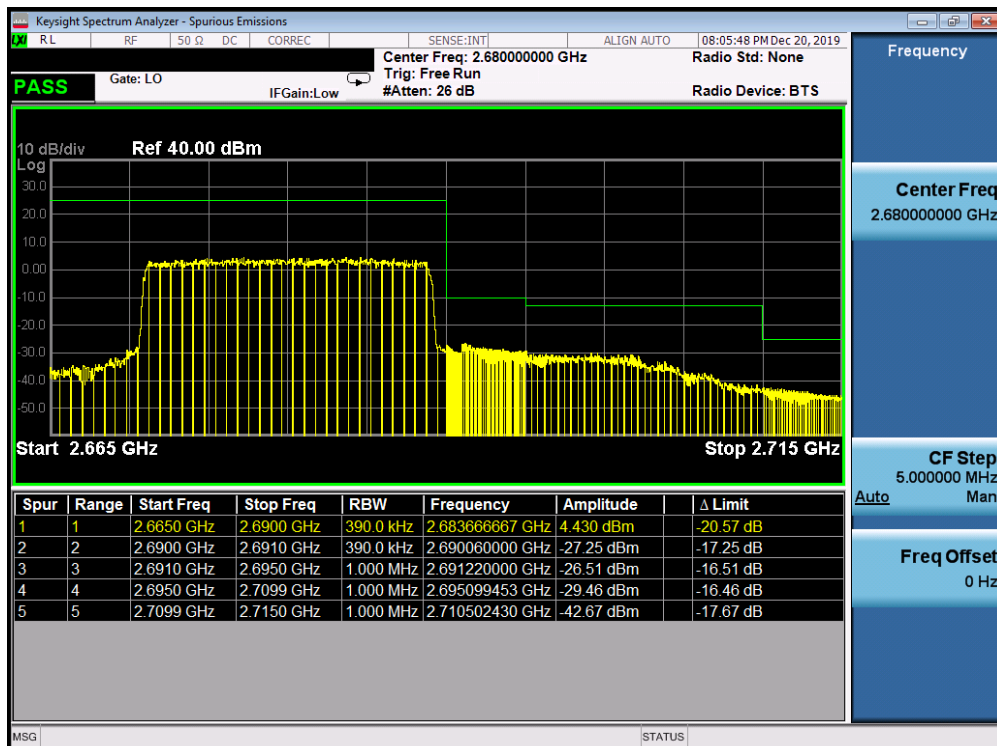
Plot 7-208. Upper ACP Plot (Band 41 PC3 - 20.0MHz QPSK - Full RB Configuration)
