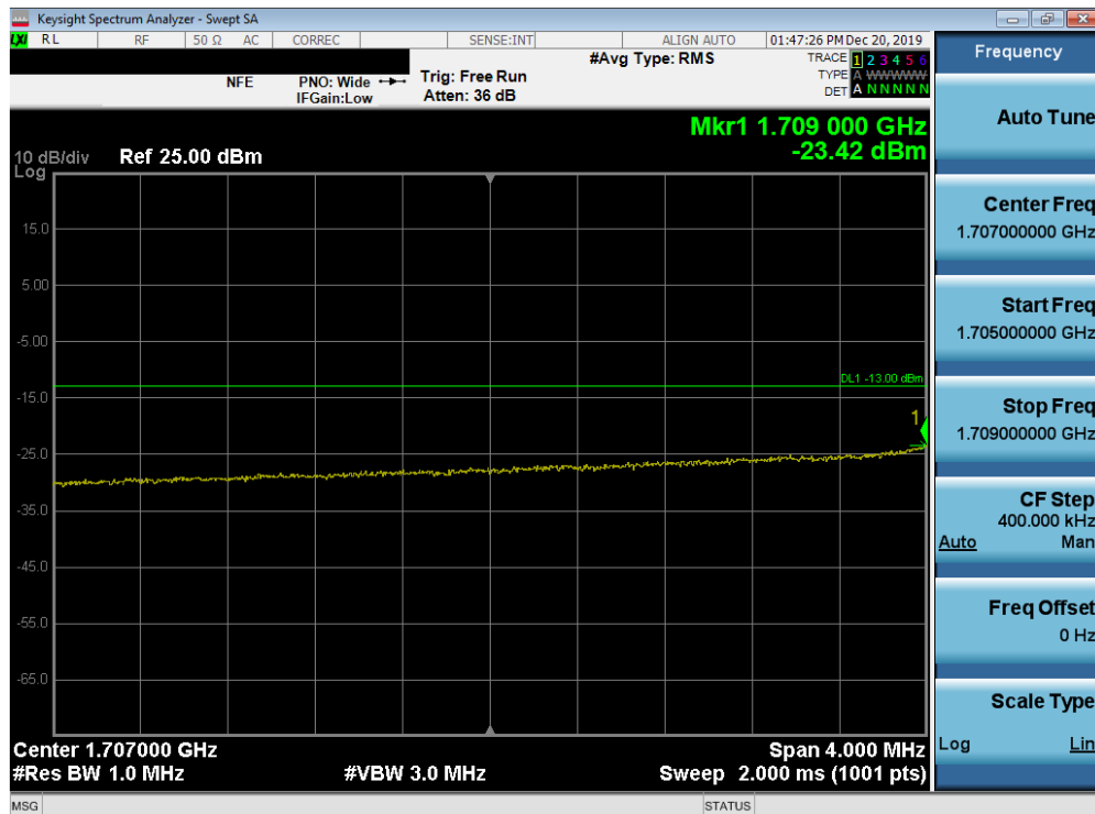
Plot 7-148. Lower Extended Band Edge Plot (Band 66/4 - 10.0MHz QPSK - Full RB Configuration)
