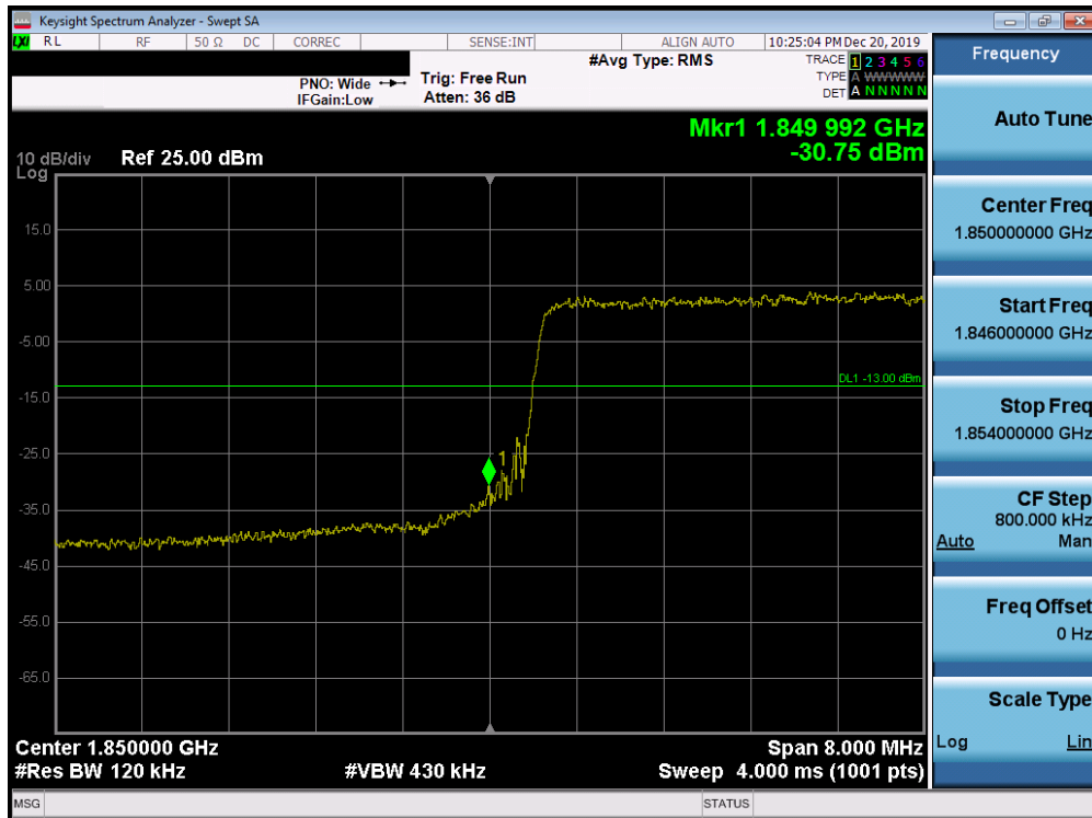
Plot 7-183. Lower Band Edge Plot (Band 25/2 - 10.0MHz QPSK - Full RB Configuration)
