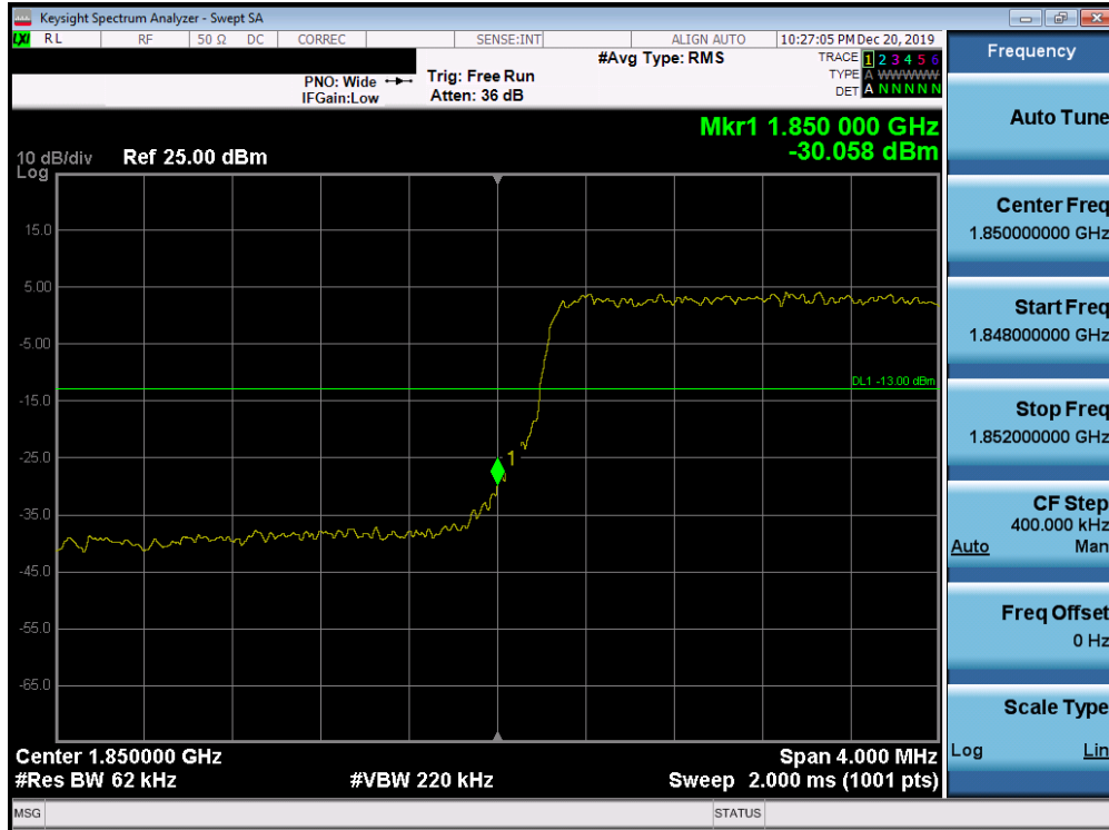
Plot 7-177. Lower Band Edge Plot (Band 25/2 - 5.0MHz QPSK - Full RB Configuration)
