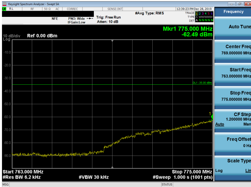
Plot 7-116. Lower Emission Mask Plot (Band 13 - 10MHz QPSK - Full RB Configuration)
