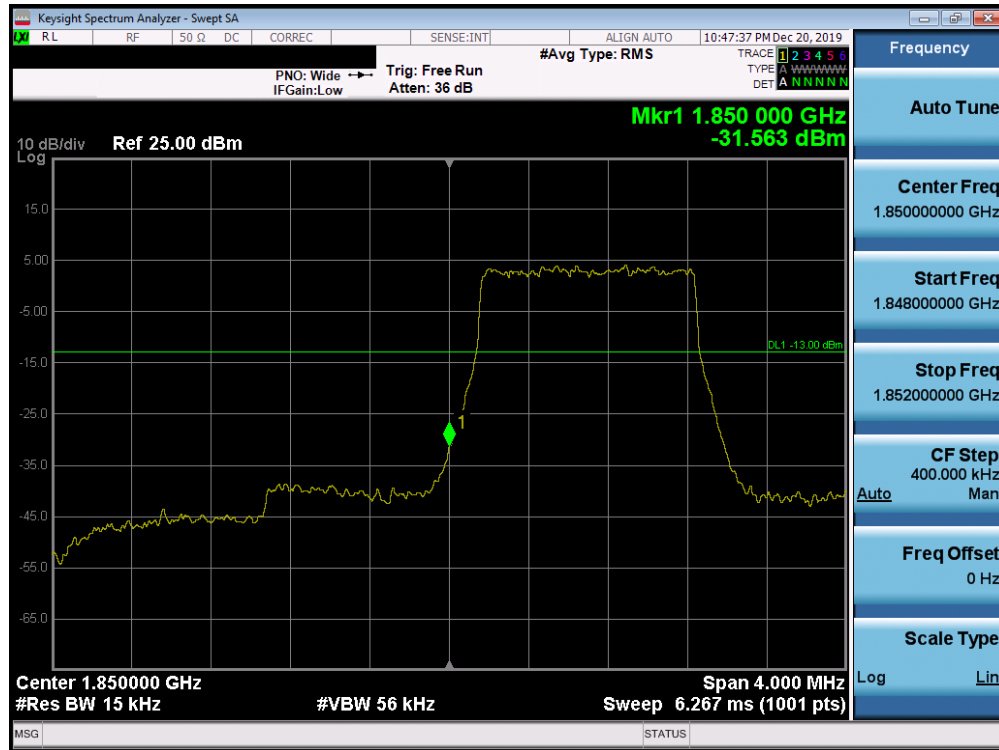
Plot 7-165. Lower Band Edge Plot (Band 25/2 - 1.4MHz QPSK - Full RB Configuration)
