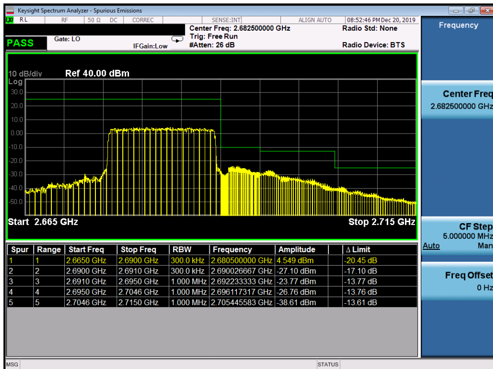
Plot 7-206. Upper ACP Plot (Band 41 PC3 - 15.0MHz QPSK - Full RB Configuration)
