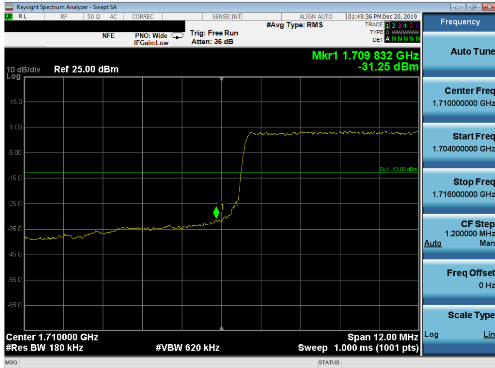
Plot 7-153. Lower Band Edge Plot (Band 66/4 - 15.0MHz QPSK - Full RB Configuration)
