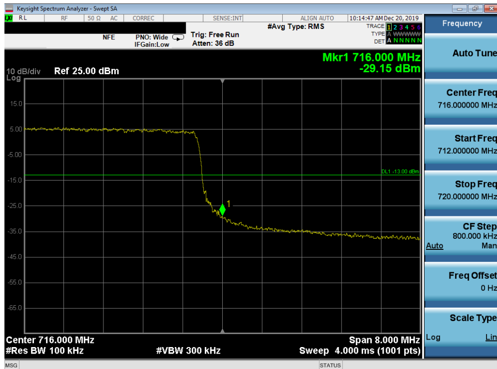
Plot 7-110. Upper Band Edge Plot (Band 12 - 10.0MHz QPSK - Full RB Configuration)
