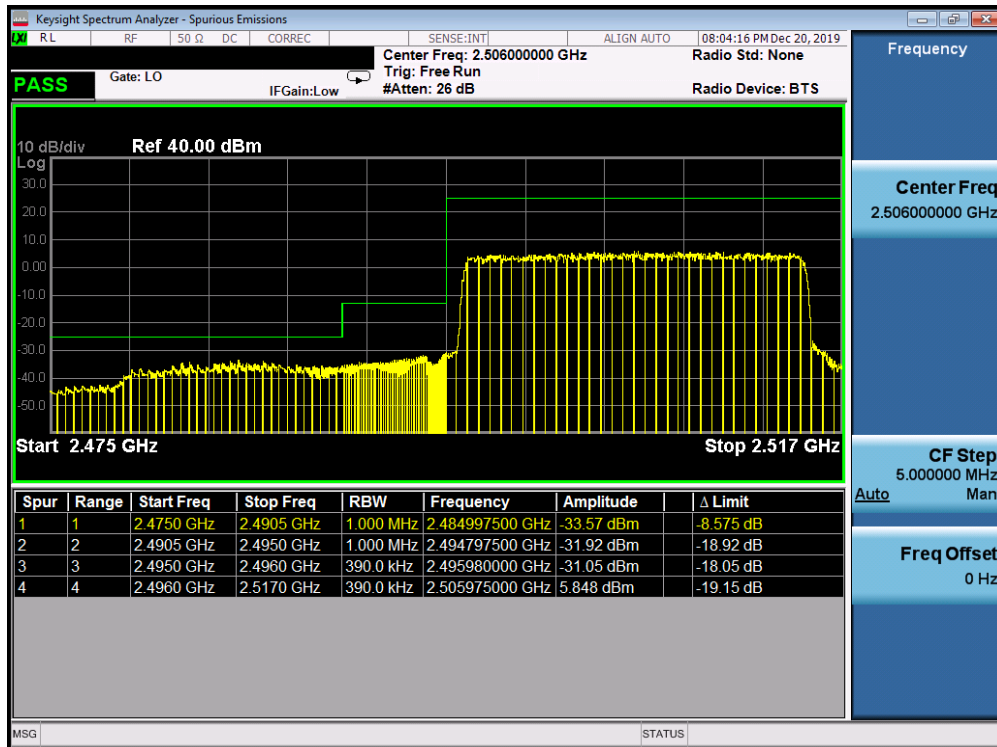
Plot 7-207. Lower ACP Plot at 2496 MHz (Band 41 PC3 - 20.0MHz QPSK - Full RB Configuration)
