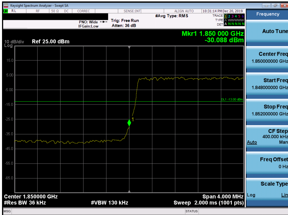
Plot 7-171. Lower Band Edge Plot (Band 25/2 - 3.0MHz QPSK - Full RB Configuration)
