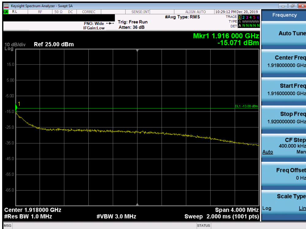
Plot 7-182. Upper Extended Band Edge Plot (Band 25 - 5.0MHz QPSK - Full RB Configuration)
