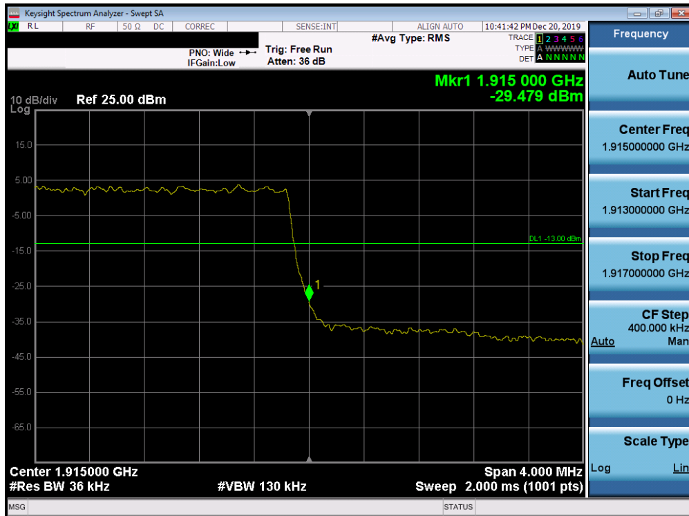
Plot 7-175. Upper Band Edge Plot (Band 25 - 3.0MHz QPSK - Full RB Configuration)
