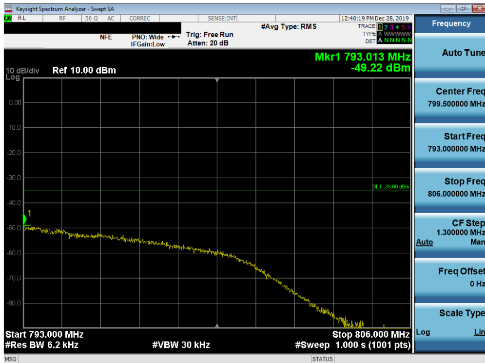
Plot 7-118. Upper Emission Mask Plot (Band 13 - 10MHz QPSK - Full RB Configuration)
