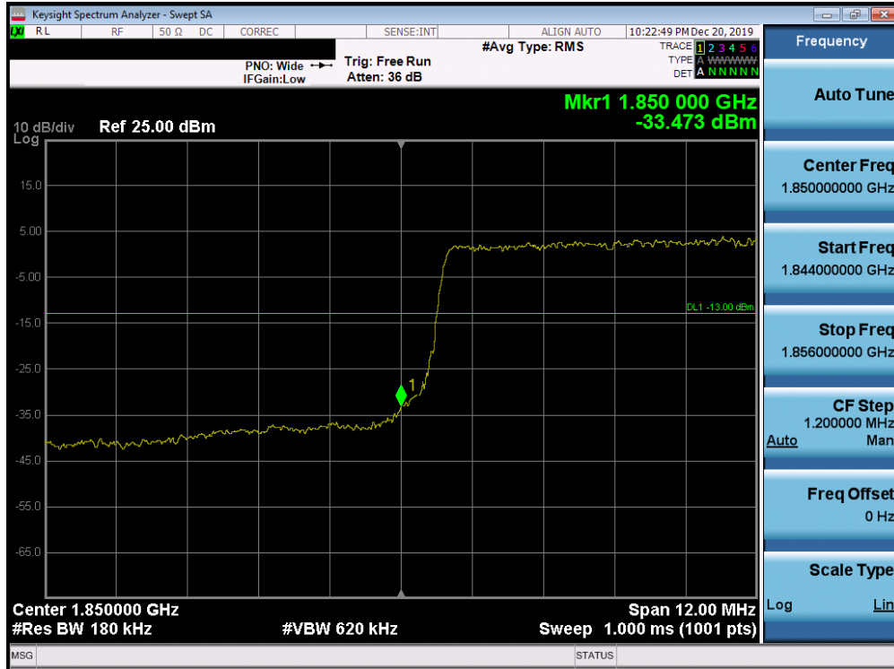
Plot 7-189. Lower Band Edge Plot (Band 25/2 - 15.0MHz QPSK - Full RB Configuration)
