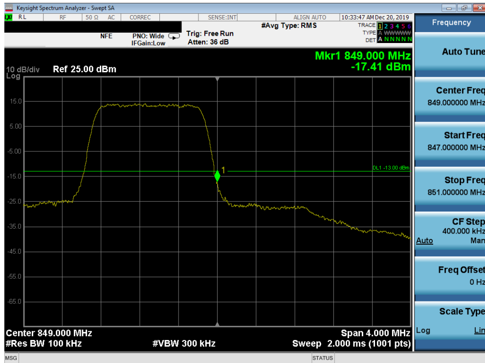
Plot 7-120. Upper Band Edge Plot (Band 26/5 - 1.4MHz QPSK - Full RB Configuration)
