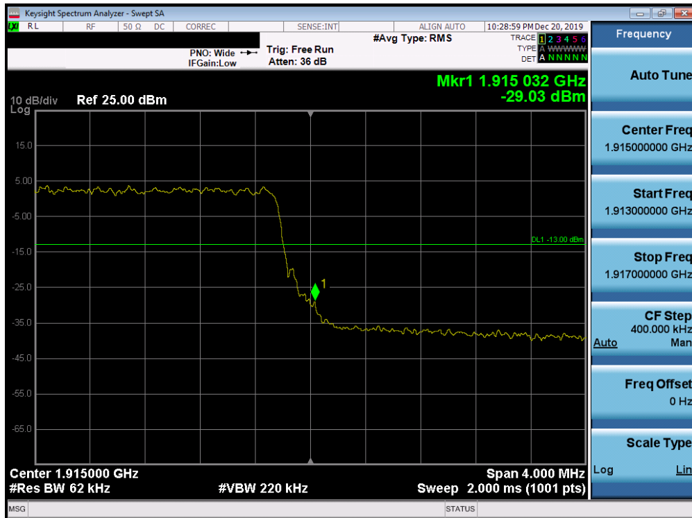
Plot 7-181. Upper Band Edge Plot (Band 25 - 5.0MHz QPSK - Full RB Configuration)
