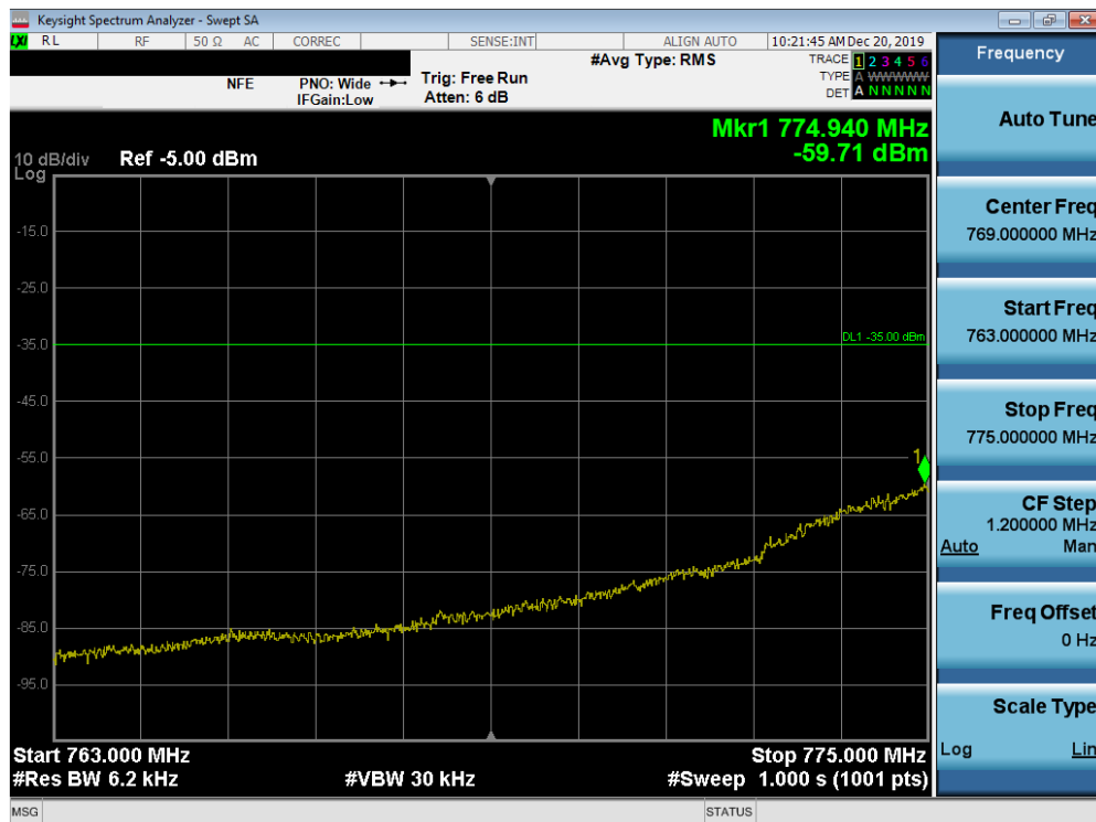
Plot 7-112. Lower Emission Mask Plot (Band 13 - 5.0MHz QPSK - Full RB Configuration)
