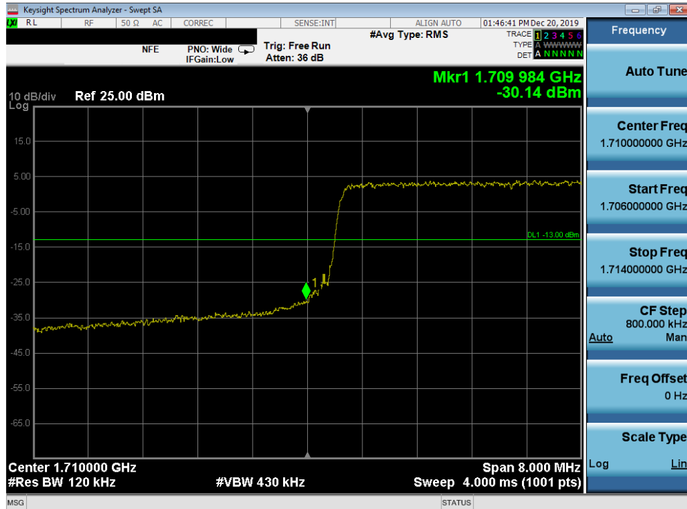
Plot 7-147. Lower Band Edge Plot (Band 66/4 - 10.0MHz QPSK - Full RB Configuration)
