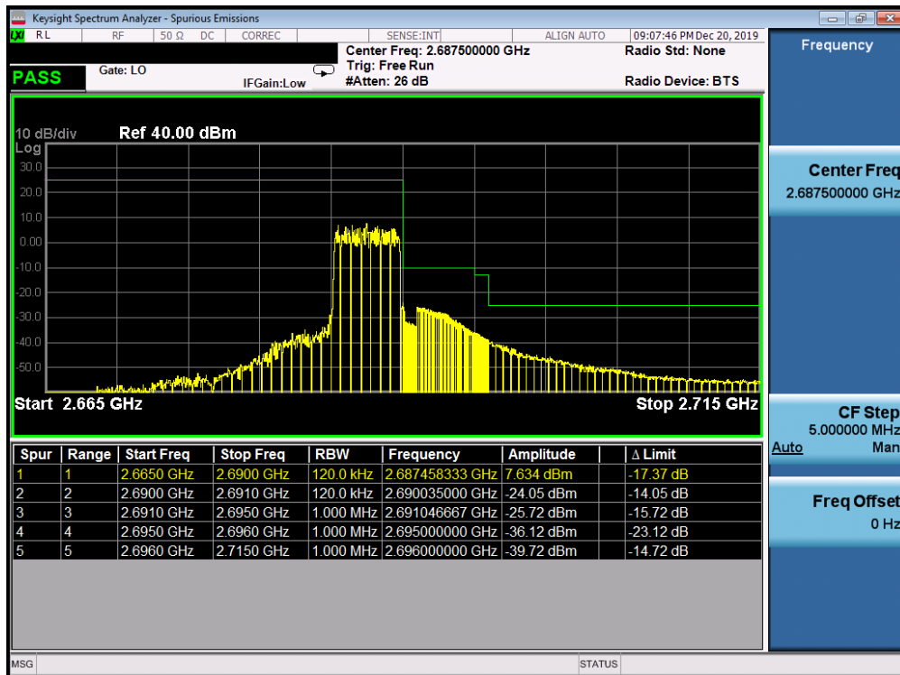
Plot 7-202. Upper ACP Plot (Band 41 PC3 - 5.0MHz QPSK - Full RB Configuration)
