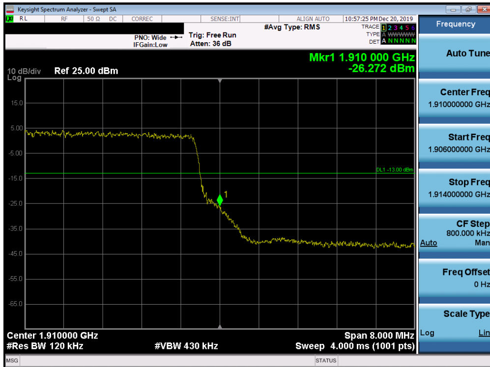
Plot 7-185. Upper Band Edge Plot (Band 2 - 10.0MHz QPSK - Full RB Configuration)
