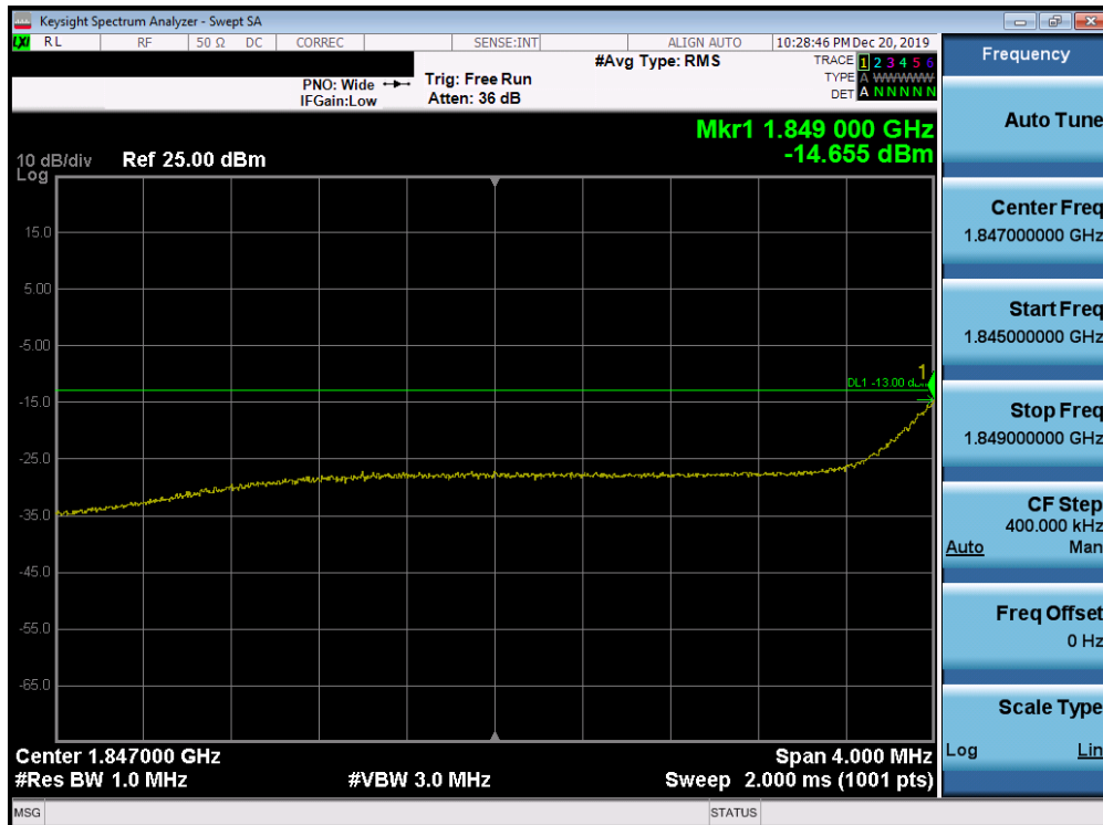
Plot 7-178. Lower Extended Band Edge Plot (Band 25/2 - 5.0MHz QPSK - Full RB Configuration)
