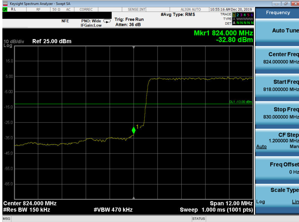
Plot 7-127. Lower Band Edge Plot (Band 26 - 15.0MHz QPSK - Full RB Configuration)
