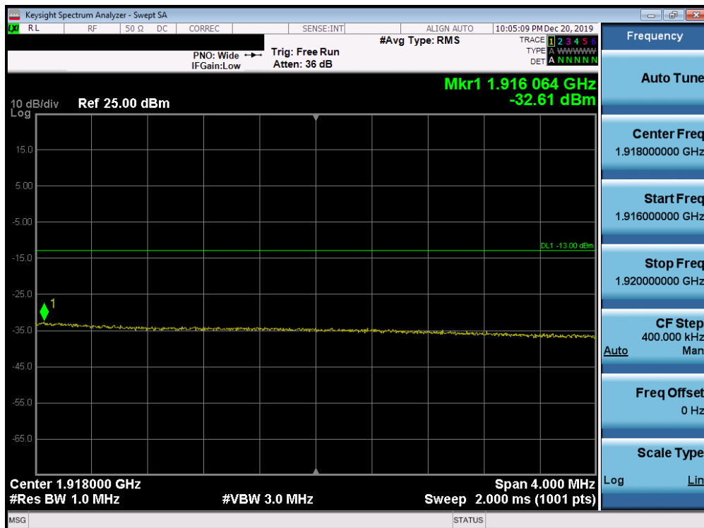
Plot 7-200. Upper Extended Band Edge Plot (Band 25 - 20.0MHz QPSK - Full RB Configuration)
