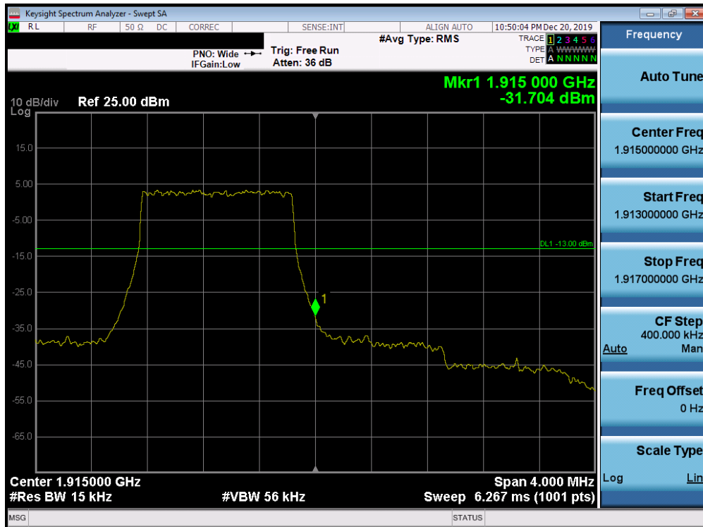
Plot 7-169. Upper Band Edge Plot (Band 25 - 1.4MHz QPSK - Full RB Configuration)
