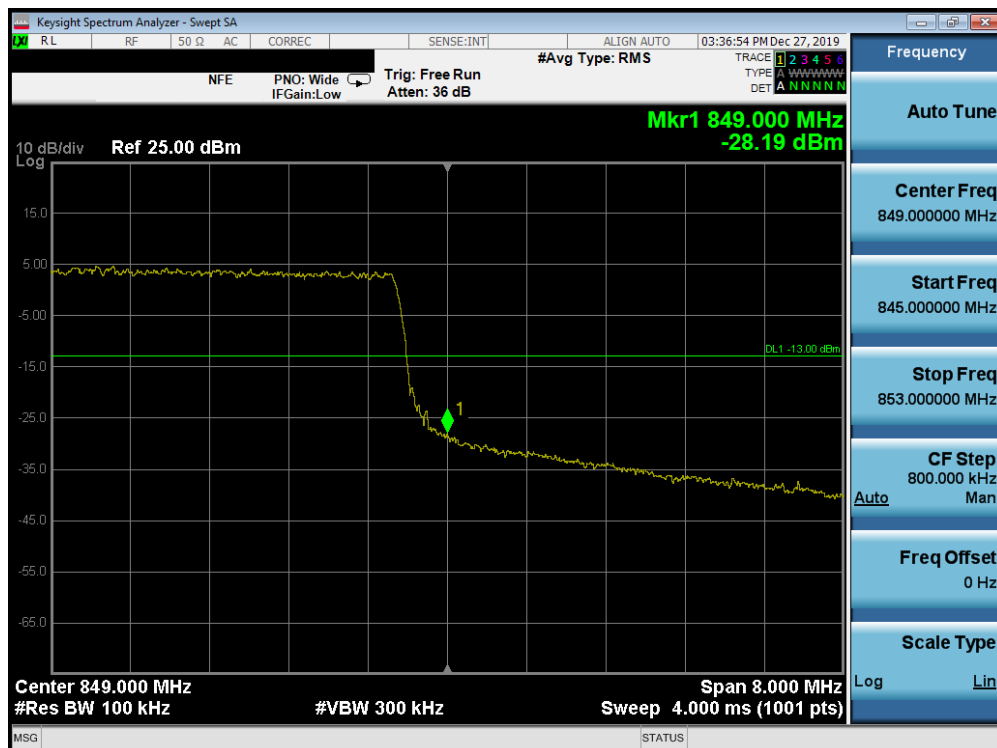
Plot 7-126. Upper Band Edge Plot (Band 26/5 - 10.0MHz QPSK - Full RB Configuration)
