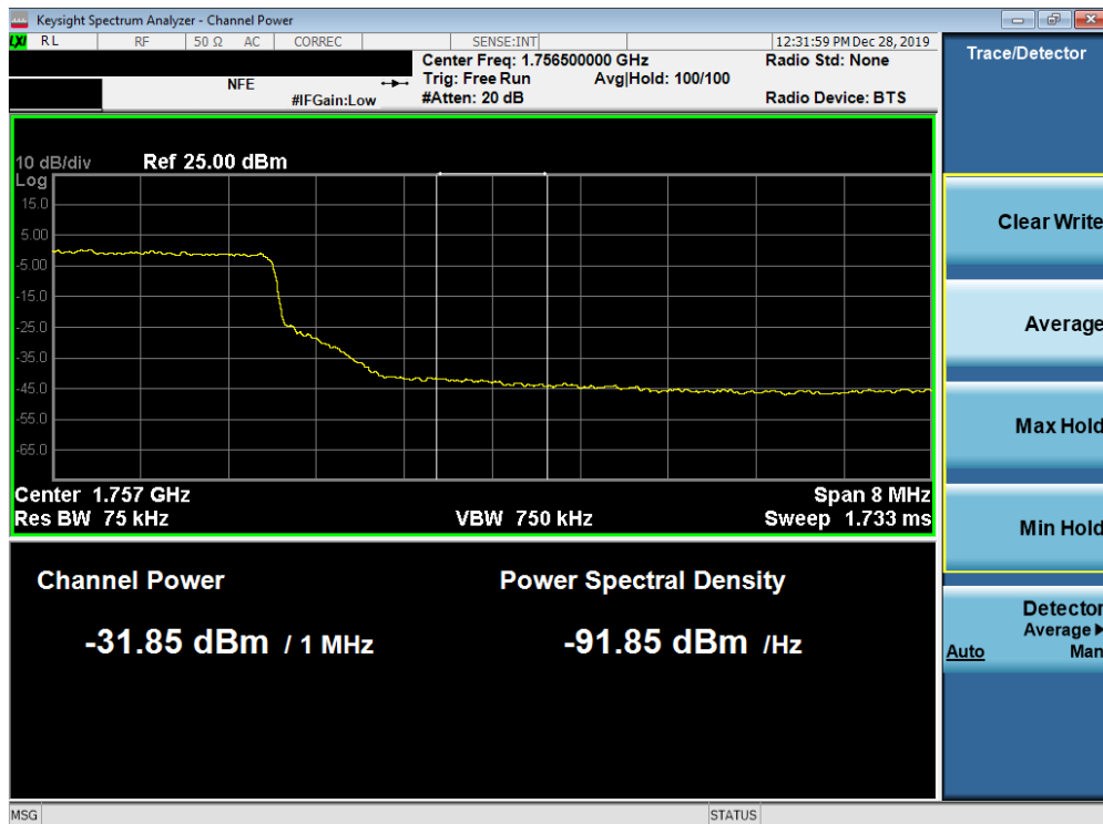
Plot 7-152. Upper Extended Band Edge Plot (Band 4 - 10.0MHz QPSK - Full RB Configuration)
