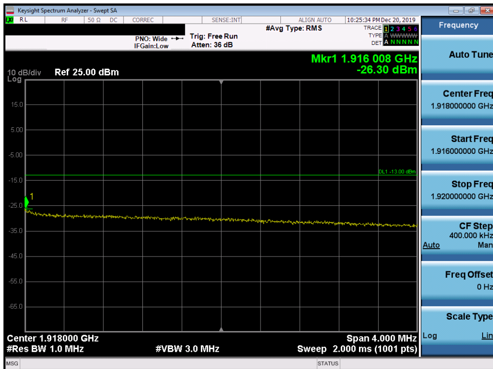
Plot 7-188. Upper Extended Band Edge Plot (Band 25 - 10.0MHz QPSK - Full RB Configuration)
