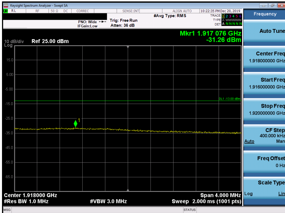
Plot 7-194. Upper Extended Band Edge Plot (Band 25 - 15.0MHz QPSK - Full RB Configuration)
