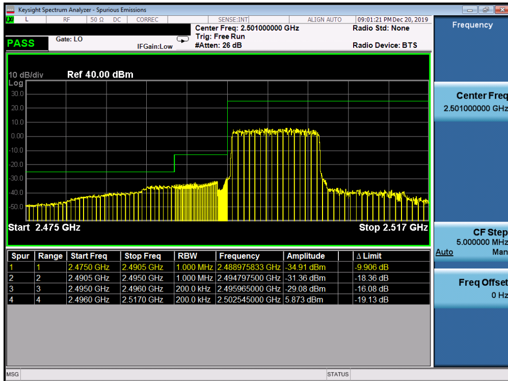
Plot 7-203. Lower ACP Plot at 2496 MHz (Band 41 PC3 - 10.0MHz QPSK - Full RB Configuration)
