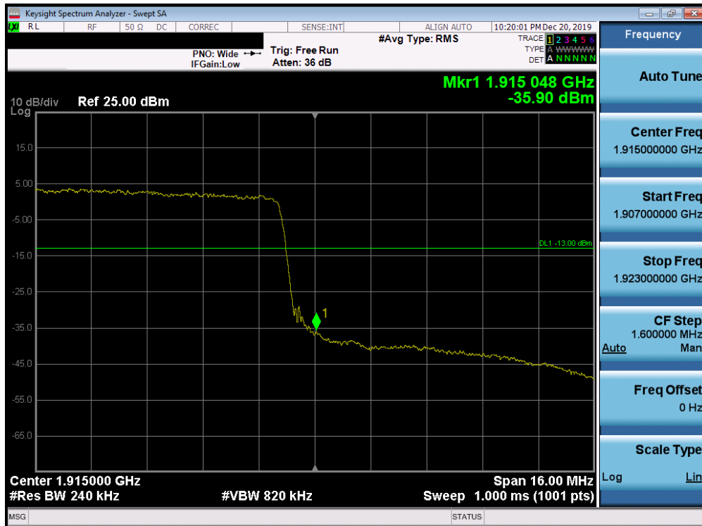
Plot 7-199. Upper Band Edge Plot (Band 25 - 20.0MHz QPSK - Full RB Configuration)
