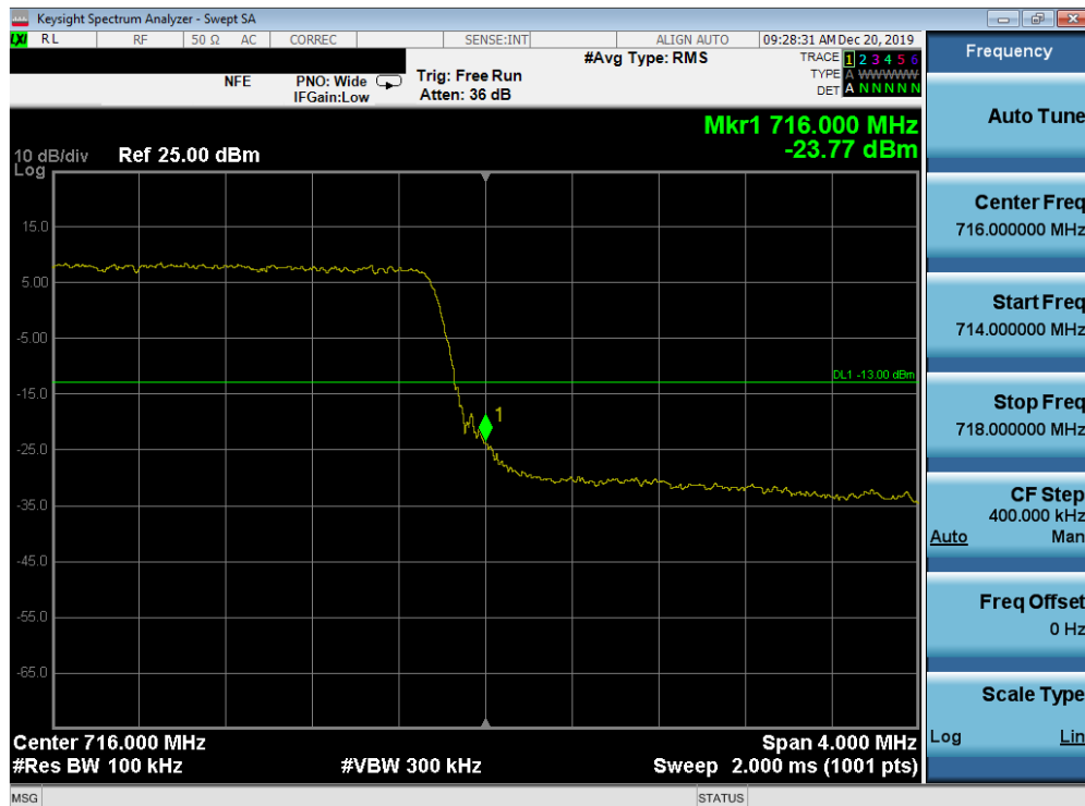
Plot 7-108. Upper Band Edge Plot (Band 12 - 5.0MHz QPSK - Full RB Configuration)
