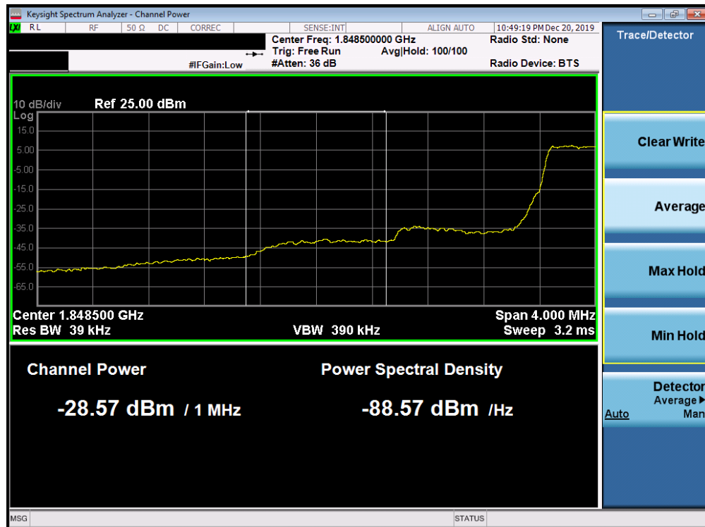
Plot 7-166. Lower Extended Band Edge Plot (Band 25/2 - 1.4MHz QPSK - Full RB Configuration)
