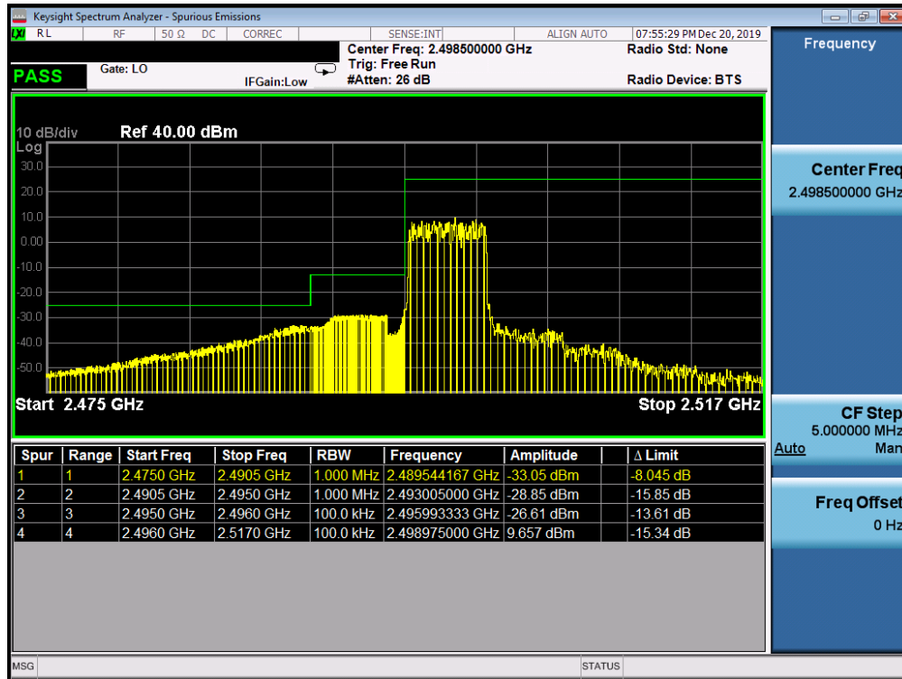
Plot 7-209. Lower ACP Plot at 2496 MHz (Band 41 PC2 - 5.0MHz QPSK - Full RB Configuration)
