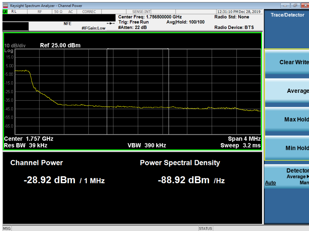
Plot 7-146. Upper Extended Band Edge Plot (Band 4 - 5.0MHz QPSK - Full RB Configuration)
