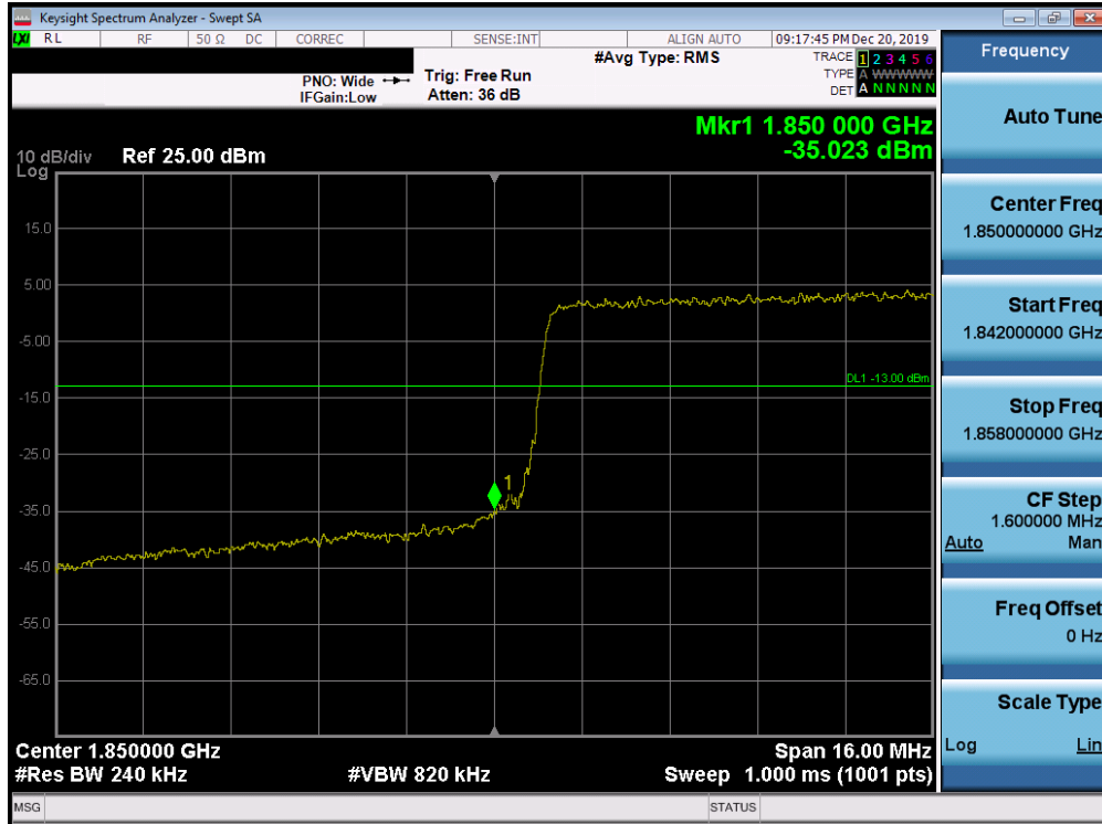
Plot 7-195. Lower Band Edge Plot (Band 25/2 - 20.0MHz QPSK - Full RB Configuration)
