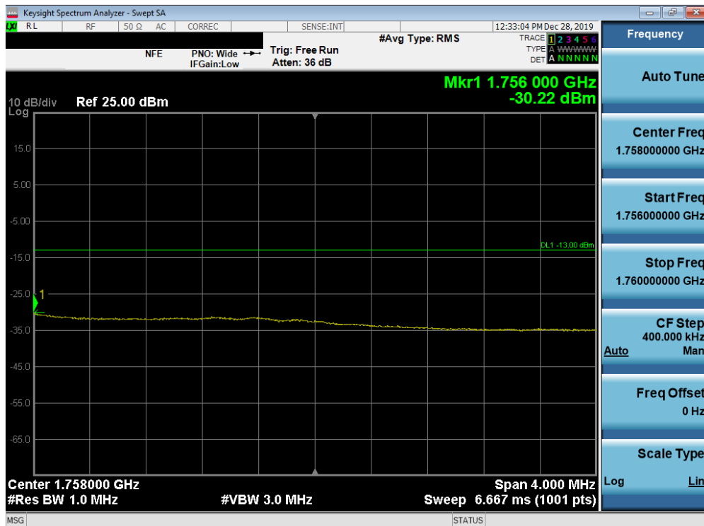
Plot 7-158. Upper Extended Band Edge Plot (Band 4 - 15.0MHz QPSK - Full RB Configuration)
