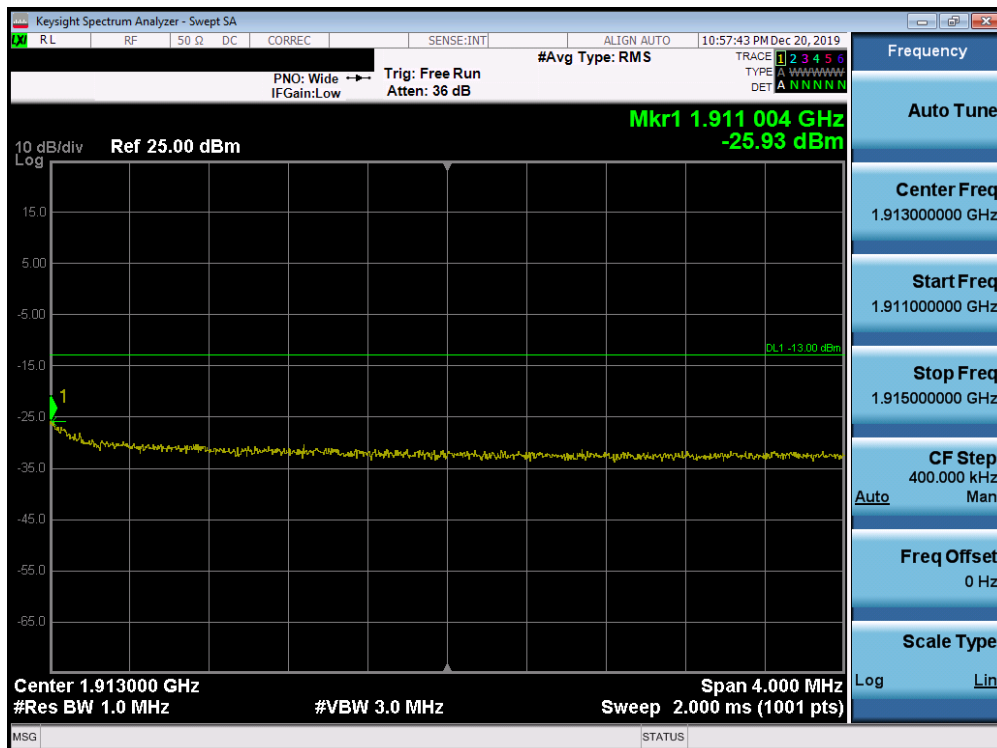
Plot 7-186. Upper Extended Band Edge Plot (Band 2 - 10.0MHz QPSK - Full RB Configuration)
