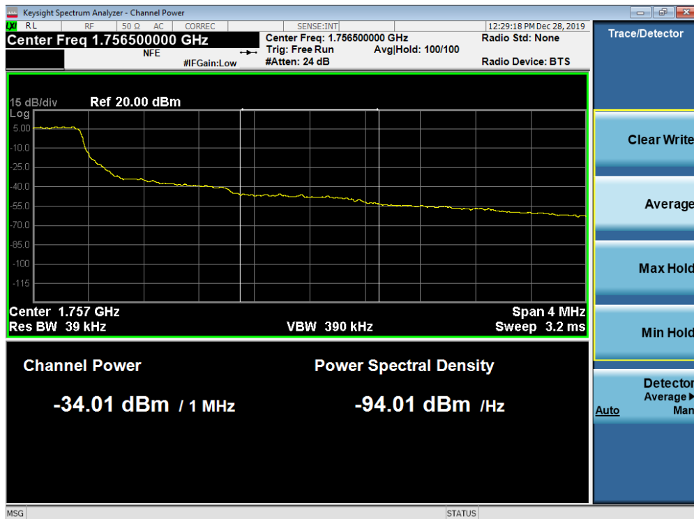
Plot 7-134. Upper Extended Band Edge Plot (Band 4 - 1.4MHz QPSK - Full RB Configuration)
