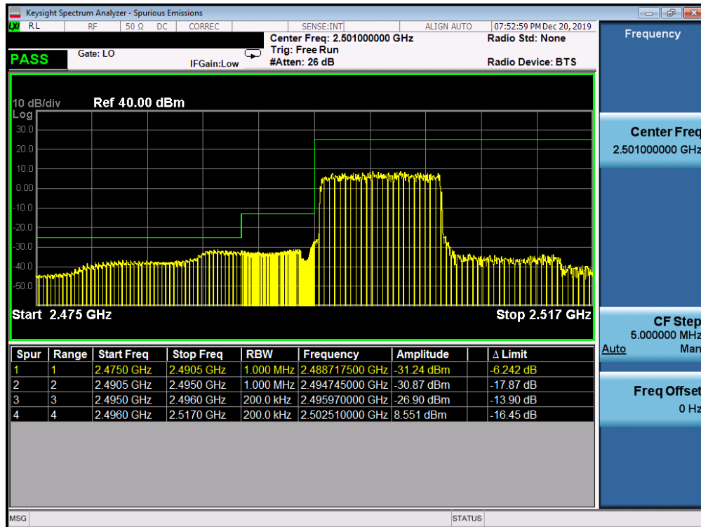
Plot 7-211. Lower ACP Plot at 2496 MHz (Band 41 PC2 - 10.0MHz QPSK - Full RB Configuration)
