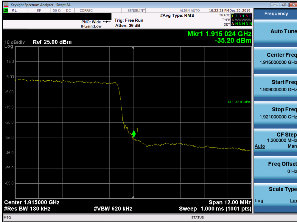
Plot 7-193. Upper Band Edge Plot (Band 25 - 15.0MHz QPSK - Full RB Configuration)
