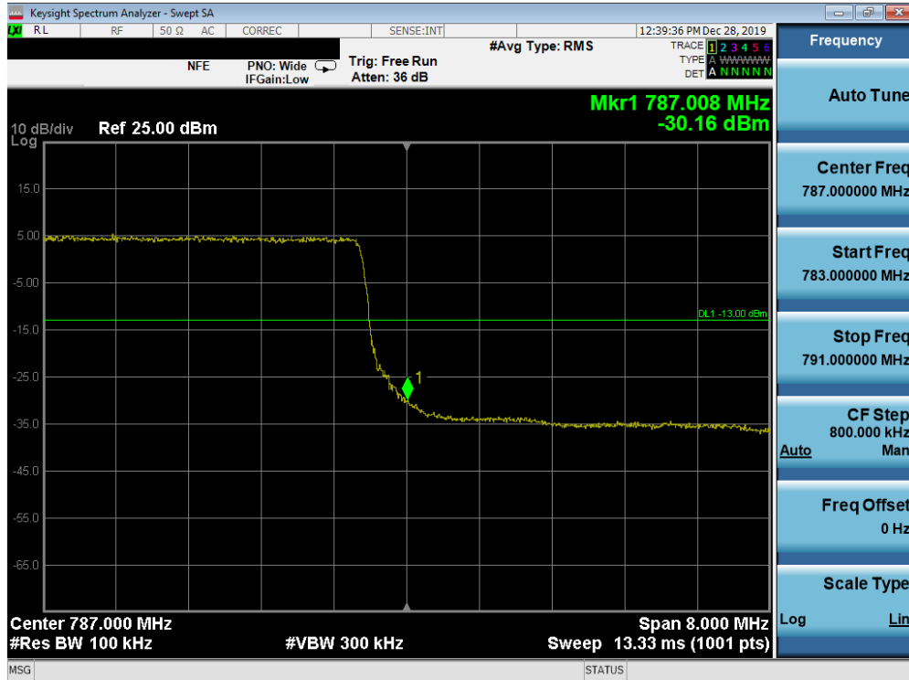
Plot 7-117. Upper Band Edge Plot (Band 13 - 10MHz QPSK - Full RB Configuration)
