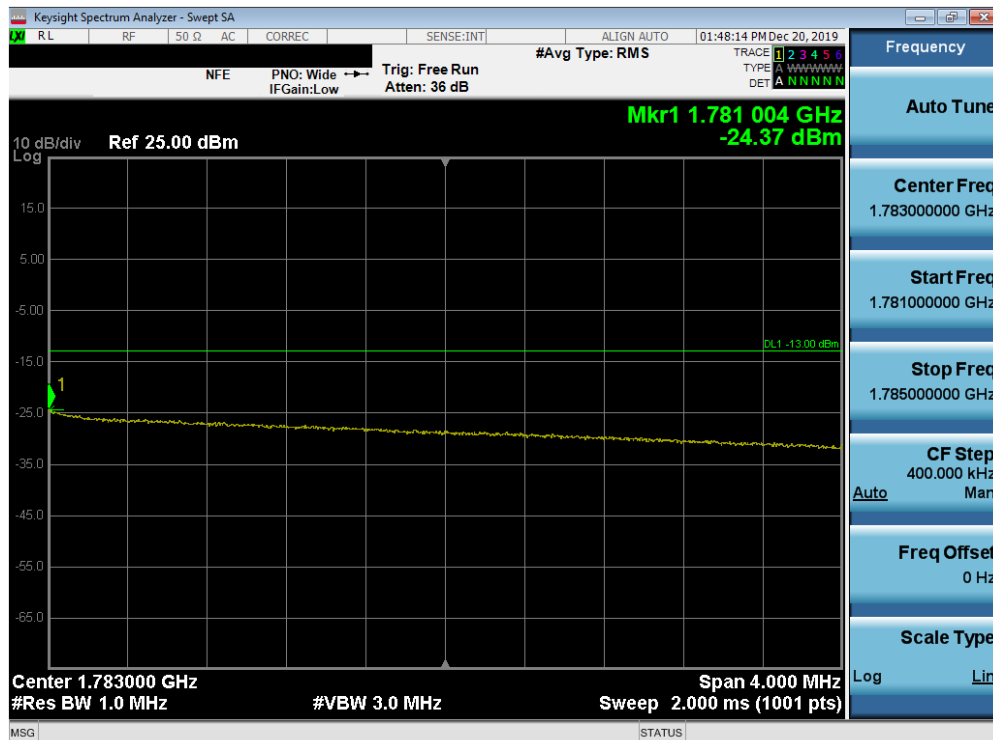
Plot 7-150. Upper Extended Band Edge Plot (Band 66 - 10.0MHz QPSK - Full RB Configuration)
