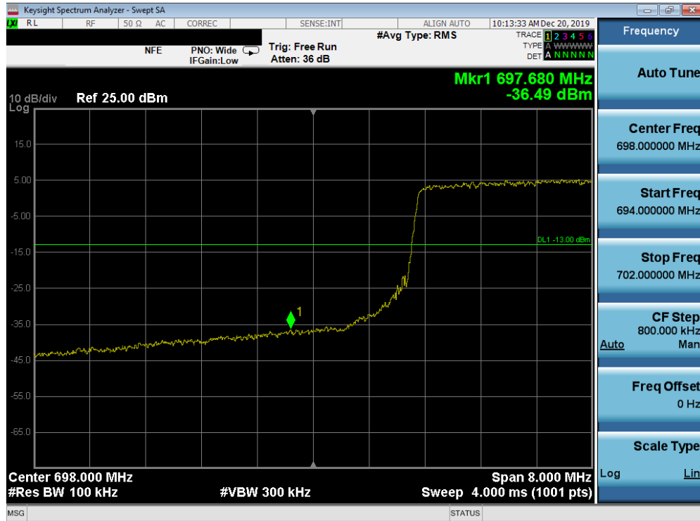
Plot 7-109. Lower Band Edge Plot (Band 12 - 10.0MHz QPSK - Full RB Configuration)
