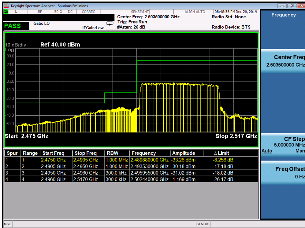
Plot 7-205. Lower ACP Plot at 2496 MHz (Band 41 PC3 - 15.0MHz QPSK - Full RB Configuration)
