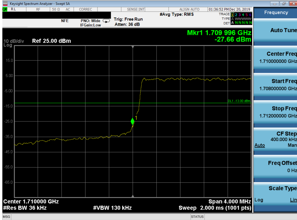
Plot 7-135. Lower Band Edge Plot (Band 66/4 - 3.0MHz QPSK - Full RB Configuration)
