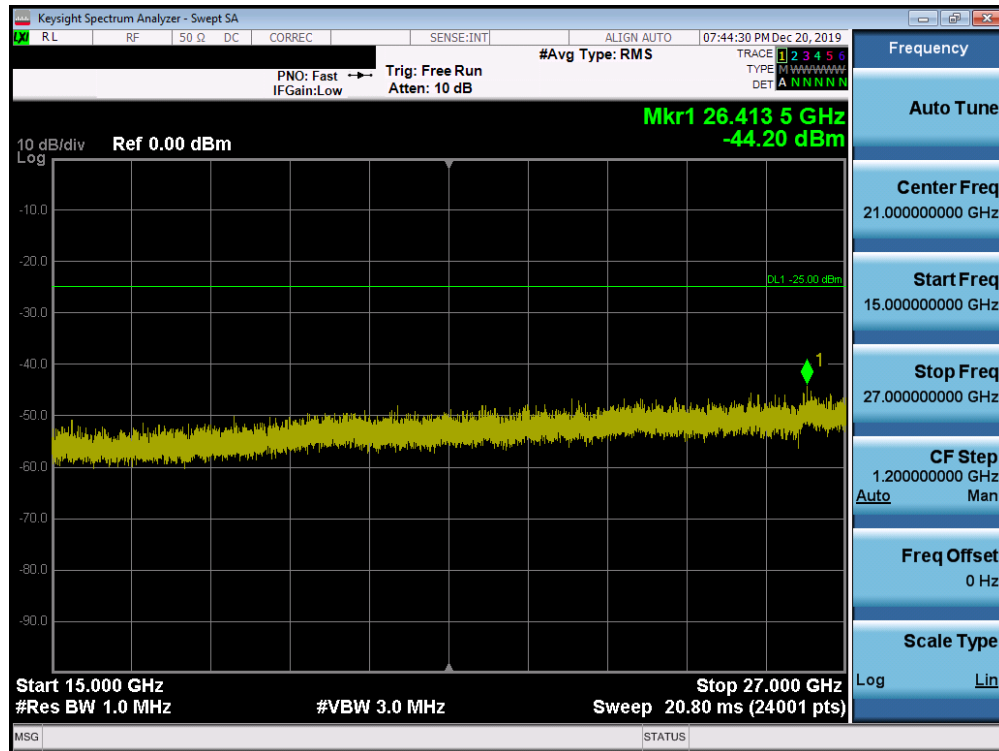
Plot 7-102. Conducted Spurious Plot (Band 41 PC2 - 20.0MHz QPSK - RB Size 1, RB Offset 0 - High Channel)
