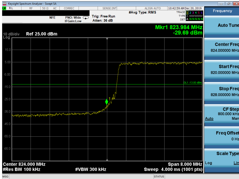
Plot 7-125. Lower Band Edge Plot (Band 26/5 - 10.0MHz QPSK - Full RB Configuration)
