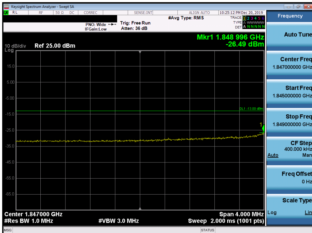
Plot 7-184. Lower Extended Band Edge Plot (Band 25/2 - 10.0MHz QPSK - Full RB Configuration)
