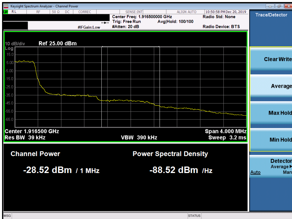
Plot 7-170. Upper Extended Band Edge Plot (Band 25 - 1.4MHz QPSK - Full RB Configuration)
