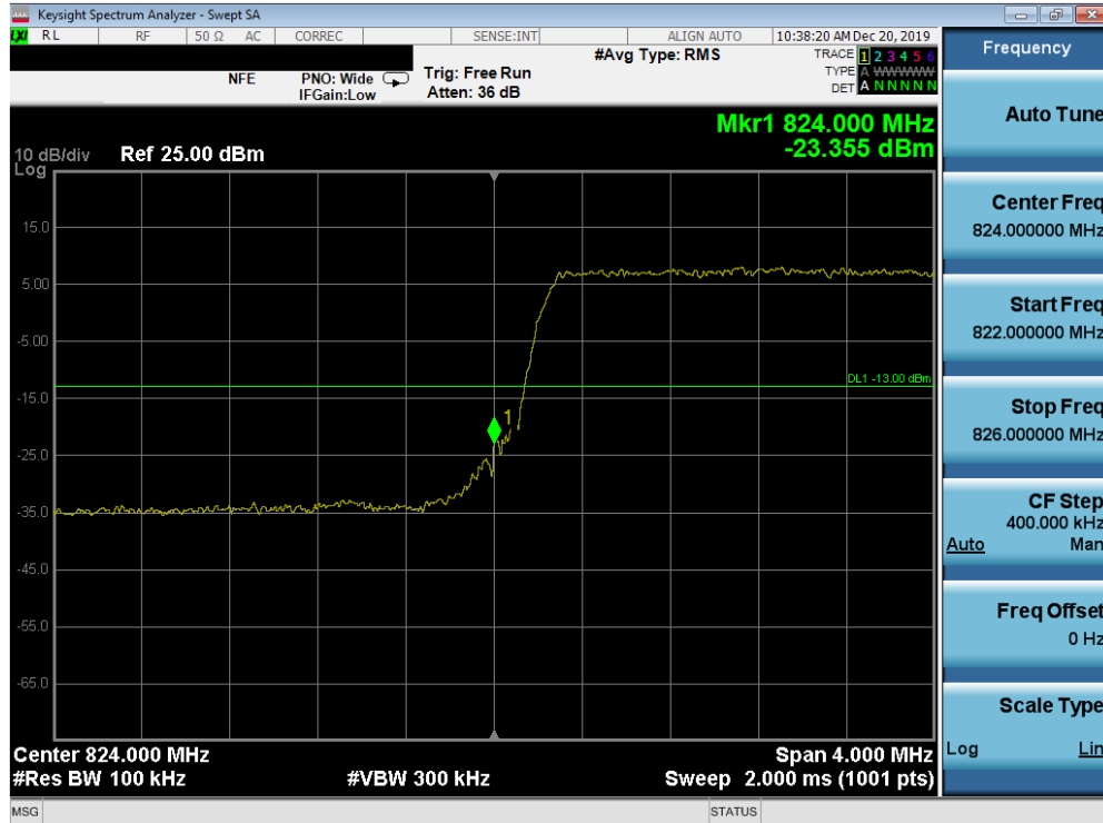
Plot 7-123. Lower Band Edge Plot (Band 26/5 - 5.0MHz QPSK - Full RB Configuration)
