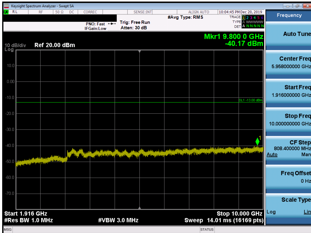
Plot 7-92. Conducted Spurious Plot (Band 25/2 - 20.0MHz QPSK - RB Size 1, RB Offset 0 - High Channel)
