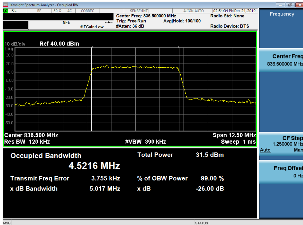
Plot 7-18. Occupied Bandwidth Plot (Band 26/5 - 5MHz 16-QAM - Full RB Configuration)
