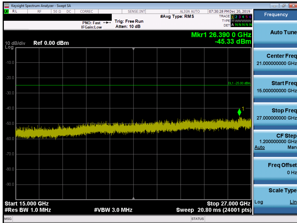
Plot 7-96. Conducted Spurious Plot (Band 41 PC2 - 20.0MHz QPSK - RB Size 1, RB Offset 0 - Low Channel)
