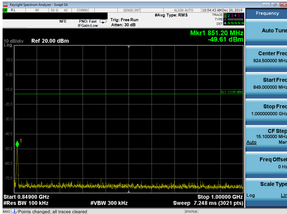
Plot 7-68. Conducted Spurious Plot (Band 26 - 15.0MHz QPSK - RB Size 1, RB Offset 0 - Low Channel)
