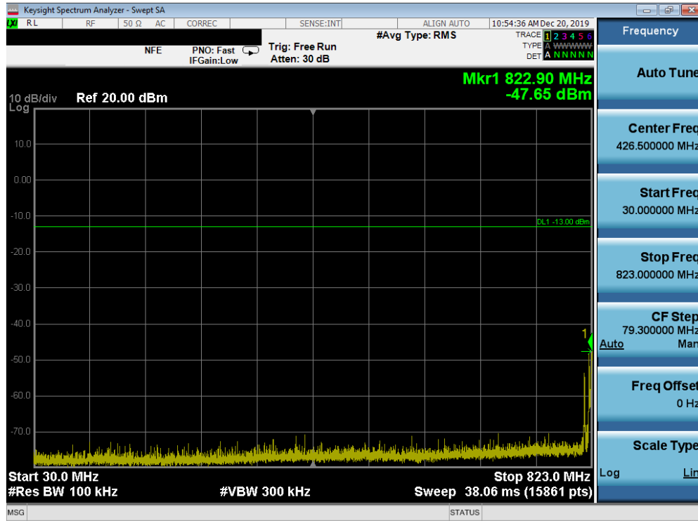
Plot 7-67. Conducted Spurious Plot (Band 26 - 15.0MHz QPSK - RB Size 1, RB Offset 0 - Low Channel)
