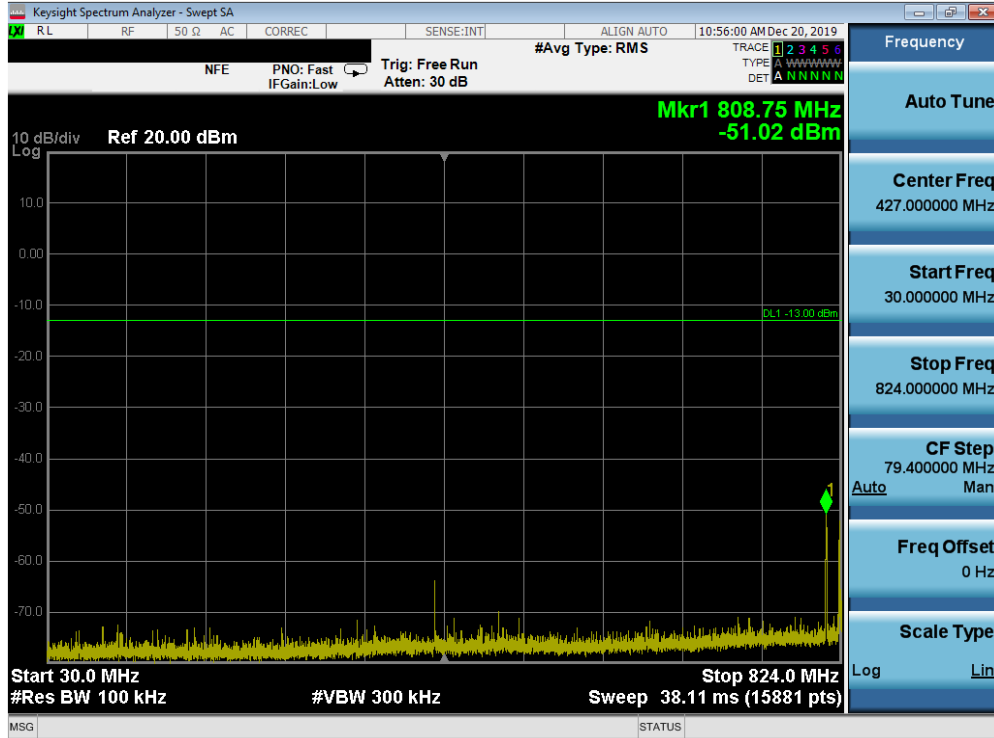
Plot 7-73. Conducted Spurious Plot (Band 26 - 15.0MHz QPSK - RB Size 1, RB Offset 0 - High Channel)
