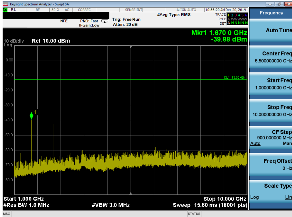
Plot 7-75. Conducted Spurious Plot (Band 26 - 15.0MHz QPSK - RB Size 1, RB Offset 0 - High Channel)
