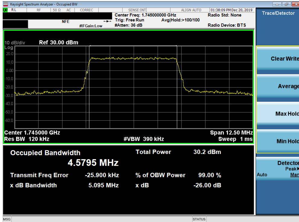
Plot 7-27. Occupied Bandwidth Plot (Band 66/4 - 5.0MHz QPSK - Full RB Configuration)
