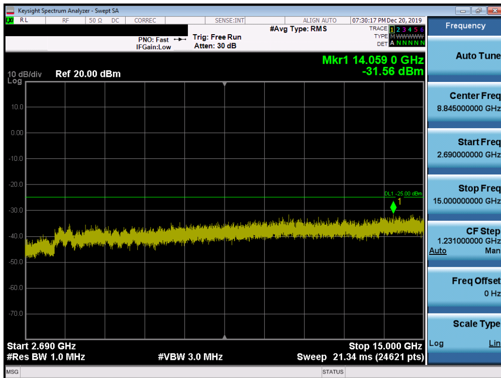
Plot 7-95. Conducted Spurious Plot (Band 41 PC2 - 20.0MHz QPSK - RB Size 1, RB Offset 0 - Low Channel)
