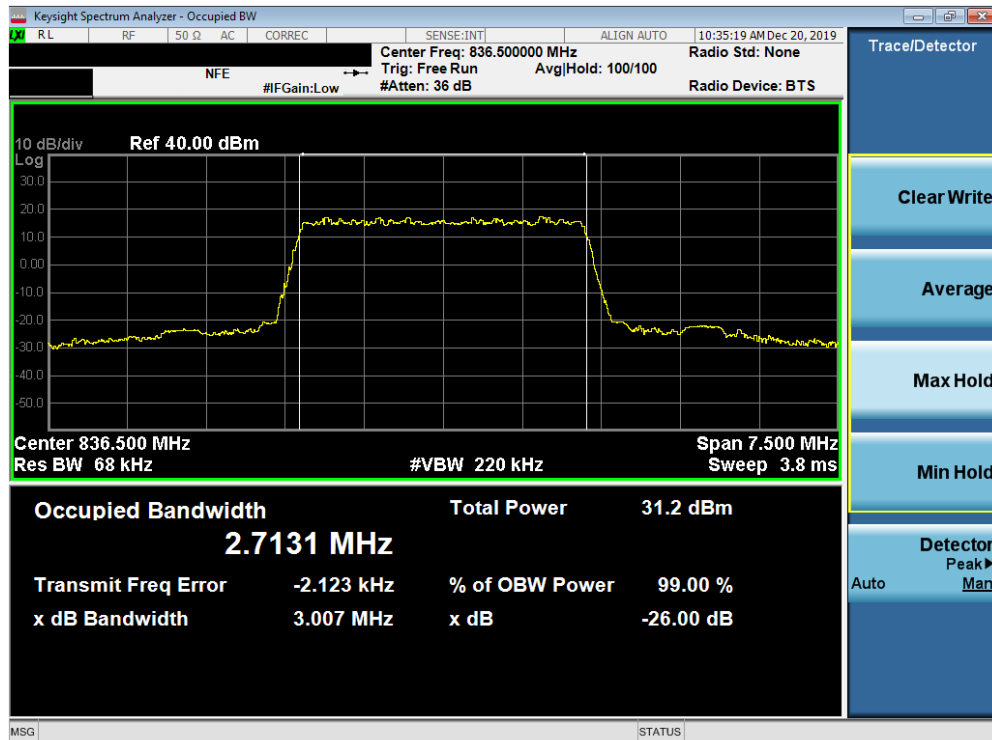
Plot 7-16. Occupied Bandwidth Plot (Band 26/5 - 3MHz 16-QAM - Full RB Configuration)
