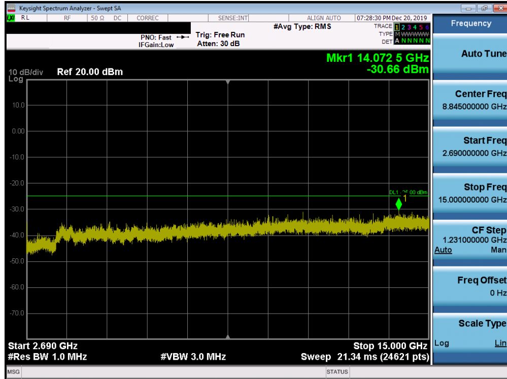
Plot 7-98. Conducted Spurious Plot (Band 41 PC2 - 20.0MHz QPSK - RB Size 1, RB Offset 0 - Mid Channel)
