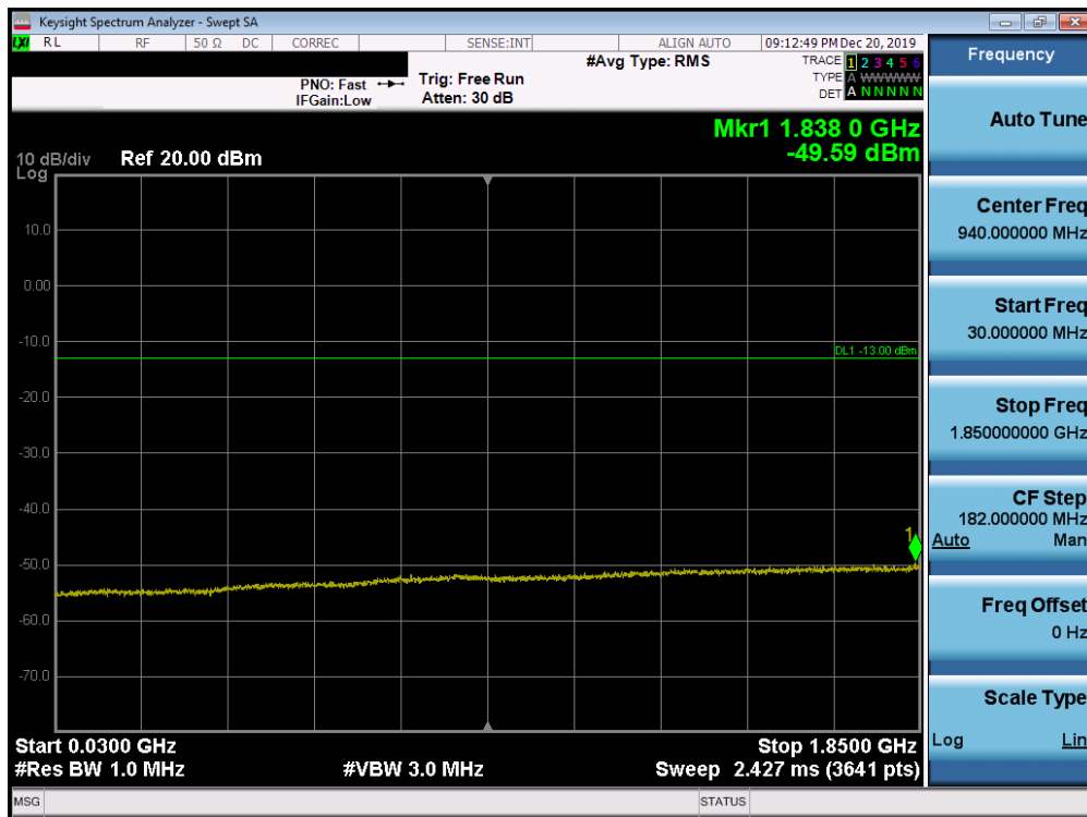
Plot 7-88. Conducted Spurious Plot (Band 25/2 - 20.0MHz QPSK - RB Size 1, RB Offset 0 - Mid Channel)
