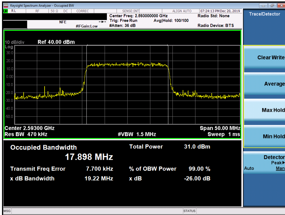
Plot 7-53. Occupied Bandwidth Plot (Band 41 PC2 - 20.0MHz QPSK - Full RB Configuration)
