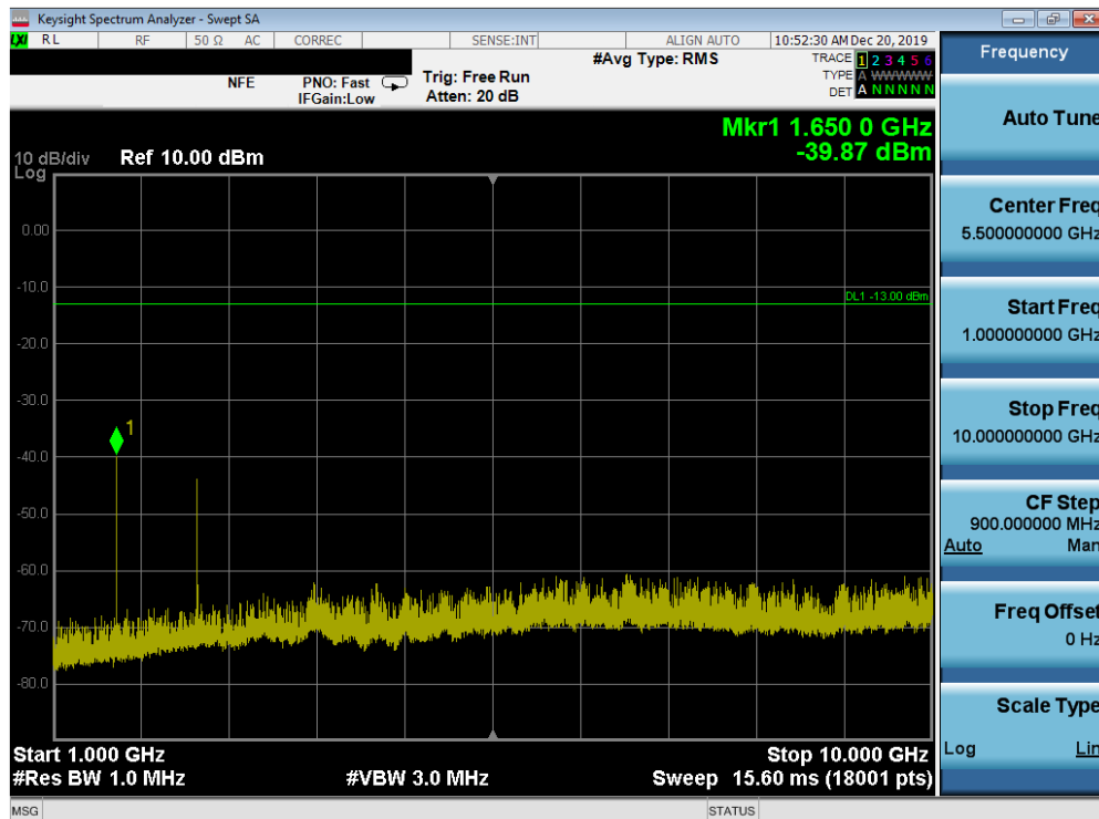
Plot 7-72. Conducted Spurious Plot (Band 26 - 15.0MHz QPSK - RB Size 1, RB Offset 0 - Mid Channel)
