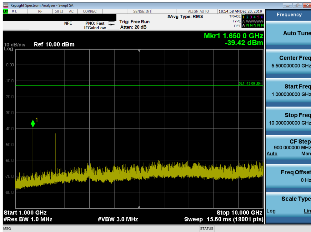
Plot 7-69. Conducted Spurious Plot (Band 26 - 15.0MHz QPSK - RB Size 1, RB Offset 0 - Low Channel)
