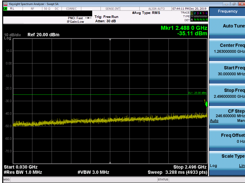
Plot 7-100. Conducted Spurious Plot (Band 41 PC2 - 20.0MHz QPSK - RB Size 1, RB Offset 0 - High Channel)
