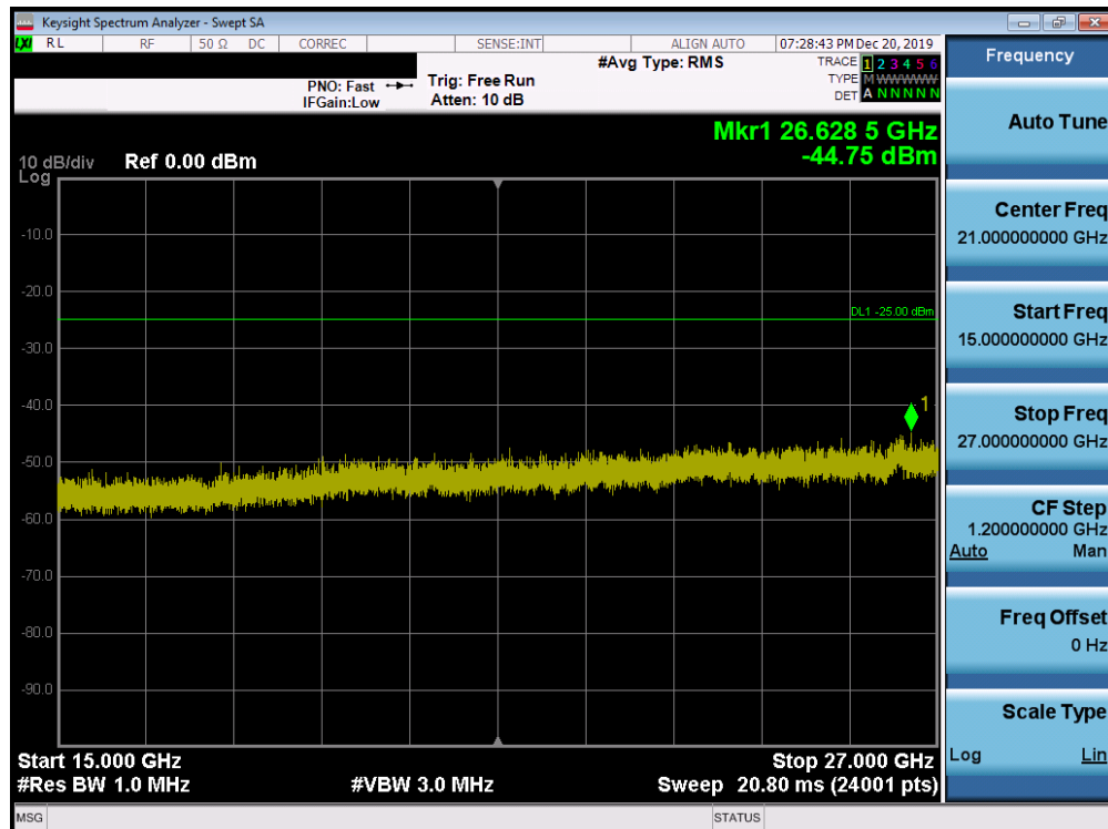
Plot 7-99. Conducted Spurious Plot (Band 41 PC2 - 20.0MHz QPSK - RB Size 1, RB Offset 0 - Mid Channel)
