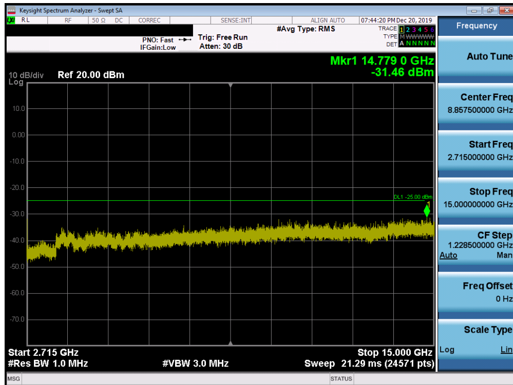
Plot 7-101. Conducted Spurious Plot (Band 41 PC2 - 20.0MHz QPSK - RB Size 1, RB Offset 0 - High Channel)
