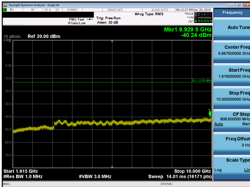
Plot 7-86. Conducted Spurious Plot (Band 25/2 - 20.0MHz QPSK - RB Size 1, RB Offset 0 - Low Channel)
