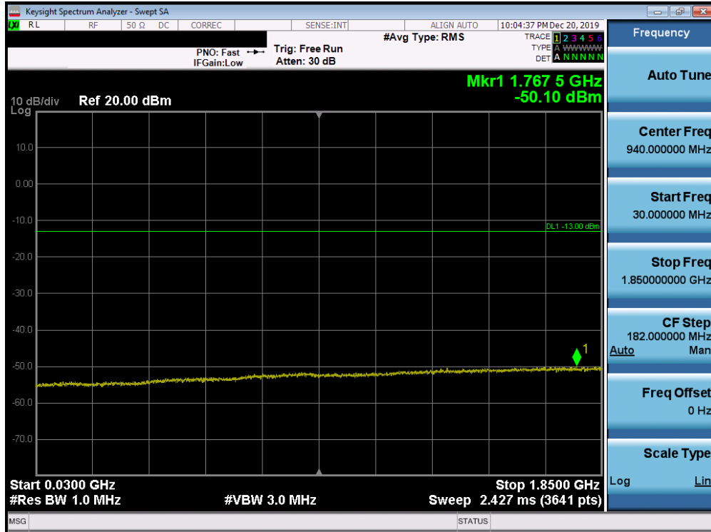
Plot 7-91. Conducted Spurious Plot (Band 25/2 - 20.0MHz QPSK - RB Size 1, RB Offset 0 - High Channel)
