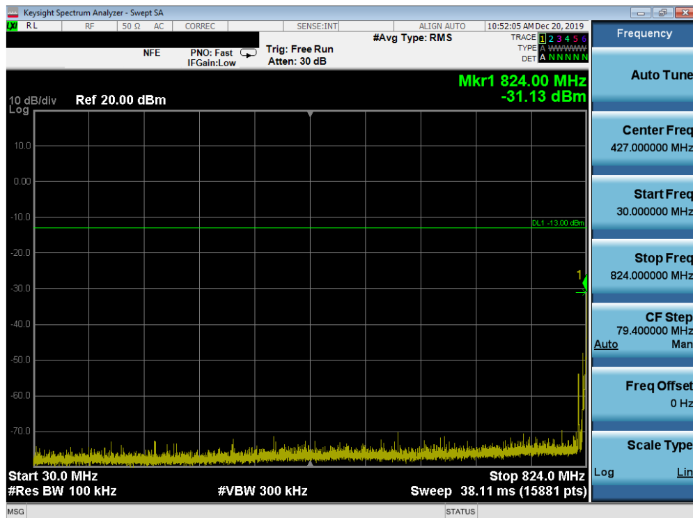
Plot 7-70. Conducted Spurious Plot (Band 26 - 15.0MHz QPSK - RB Size 1, RB Offset 0 - Mid Channel)
