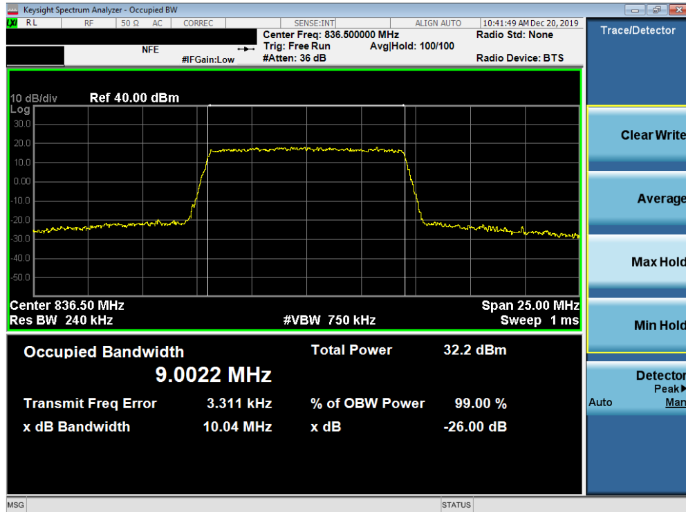
Plot 7-19. Occupied Bandwidth Plot (Band 26/5 - 10MHz QPSK - Full RB Configuration)
