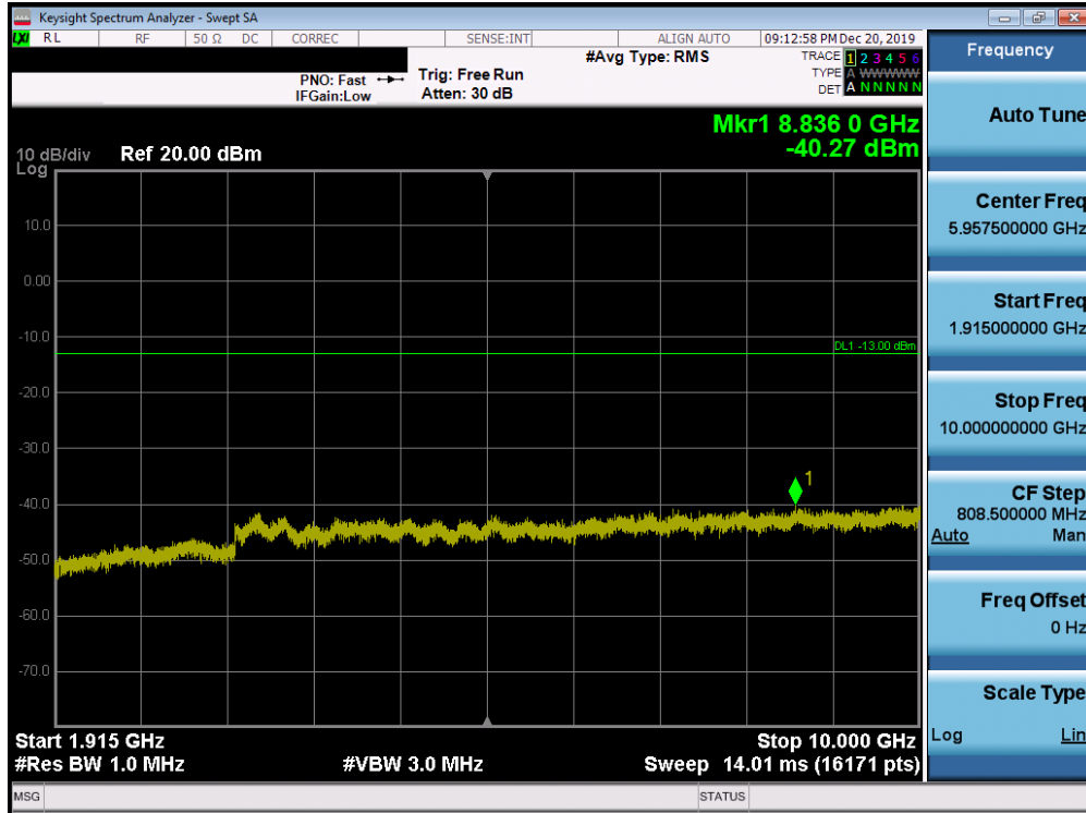
Plot 7-89. Conducted Spurious Plot (Band 25/2 - 20.0MHz QPSK - RB Size 1, RB Offset 0 - Mid Channel)
