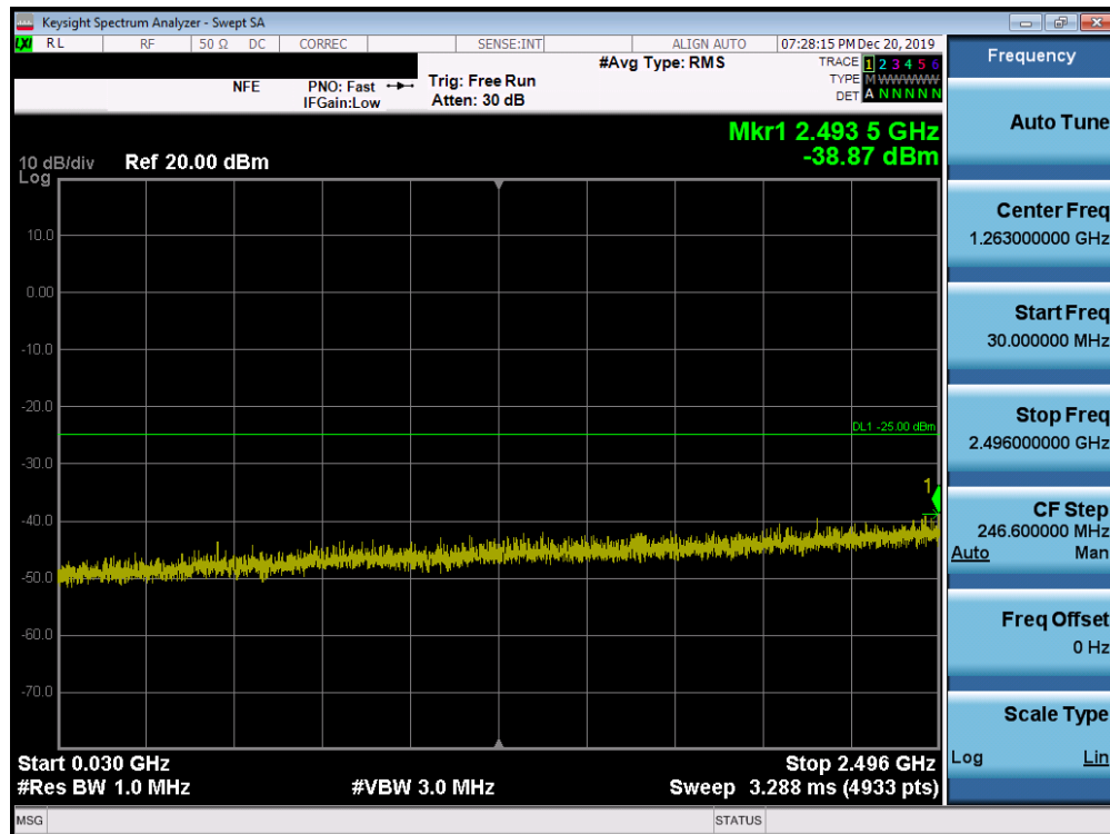
Plot 7-97. Conducted Spurious Plot (Band 41 PC2 - 20.0MHz QPSK - RB Size 1, RB Offset 0 - Mid Channel)
