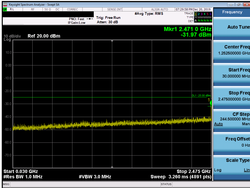
Plot 7-94. Conducted Spurious Plot (Band 41 PC2 - 20.0MHz QPSK - RB Size 1, RB Offset 0 - Low Channel)
