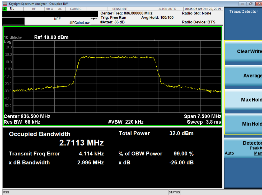
Plot 7-15. Occupied Bandwidth Plot (Band 26/5 - 3MHz QPSK - Full RB Configuration)
