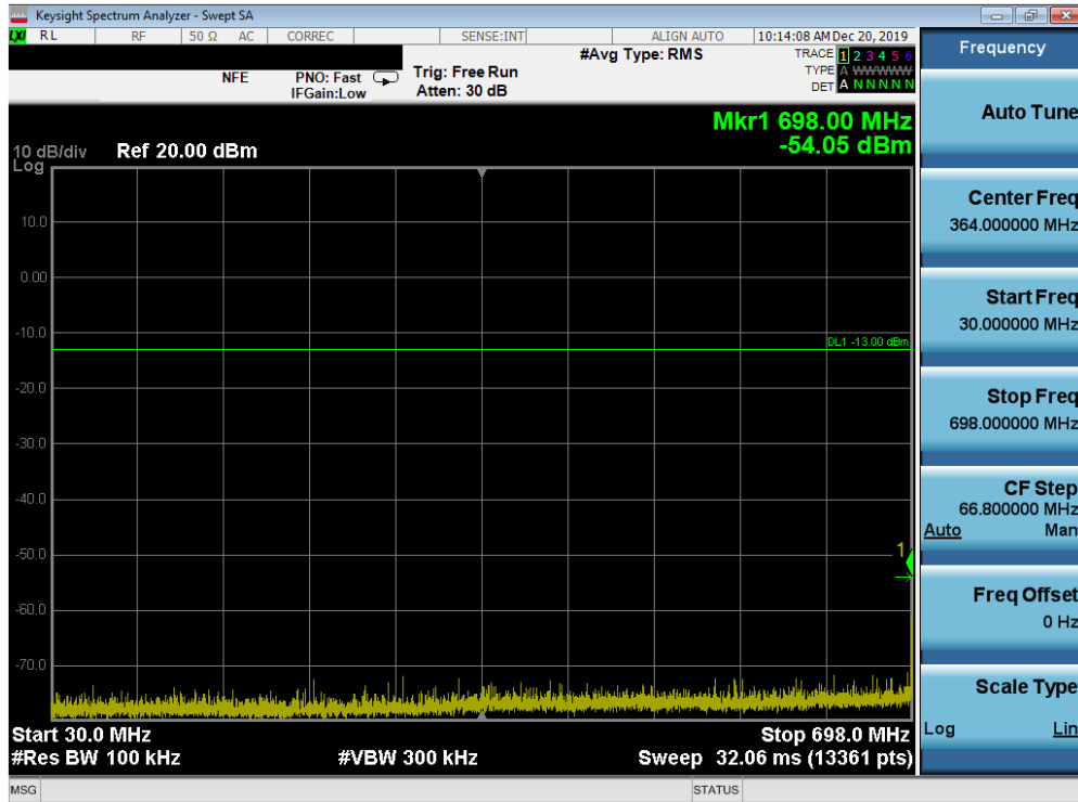
Plot 7-61. Conducted Spurious Plot (Band 12 - 10.0MHz QPSK - RB Size 1, RB Offset 0 - High Channel)
