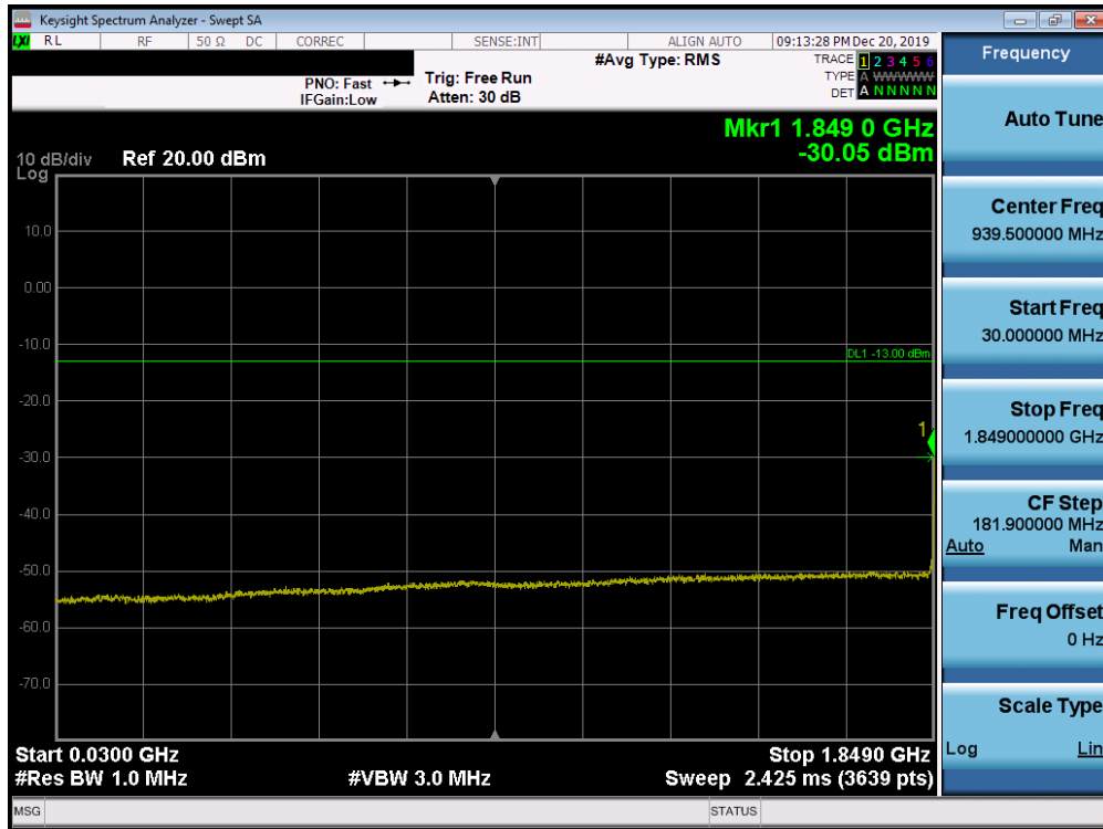
Plot 7-85. Conducted Spurious Plot (Band 25/2 - 20.0MHz QPSK - RB Size 1, RB Offset 0 - Low Channel)
