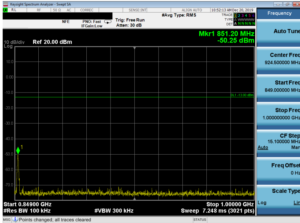
Plot 7-71. Conducted Spurious Plot (Band 26 - 15.0MHz QPSK - RB Size 1, RB Offset 0 - Mid Channel)
