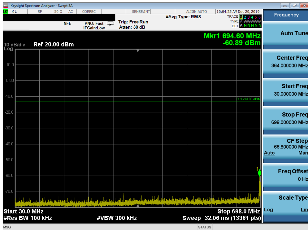
Plot 7-58. Conducted Spurious Plot (Band 12 - 10.0MHz QPSK - RB Size 1, RB Offset 0 - Mid Channel)
