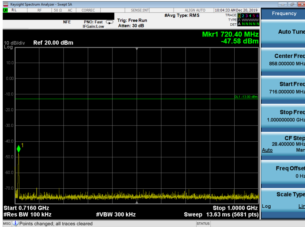
Plot 7-59. Conducted Spurious Plot (Band 12 - 10.0MHz QPSK - RB Size 1, RB Offset 0 - Mid Channel)
