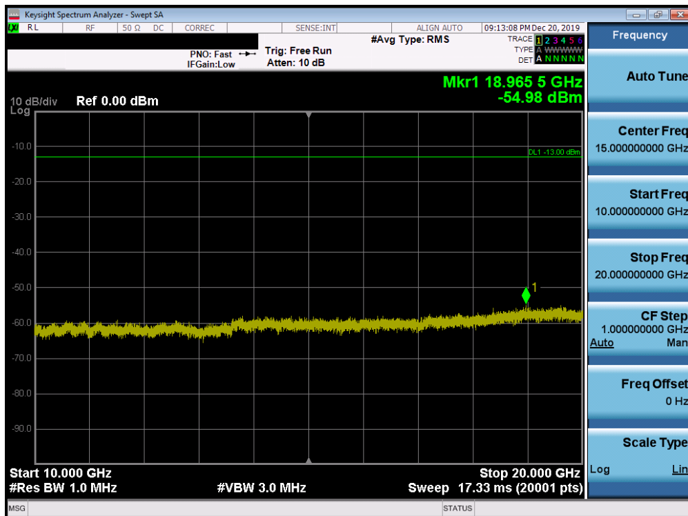
Plot 7-90. Conducted Spurious Plot (Band 25/2 - 20.0MHz QPSK - RB Size 1, RB Offset 0 - Mid Channel)
