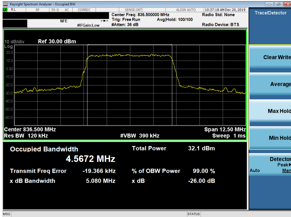
Plot 7-17. Occupied Bandwidth Plot (Band 26/5 - 5MHz QPSK - Full RB Configuration)
