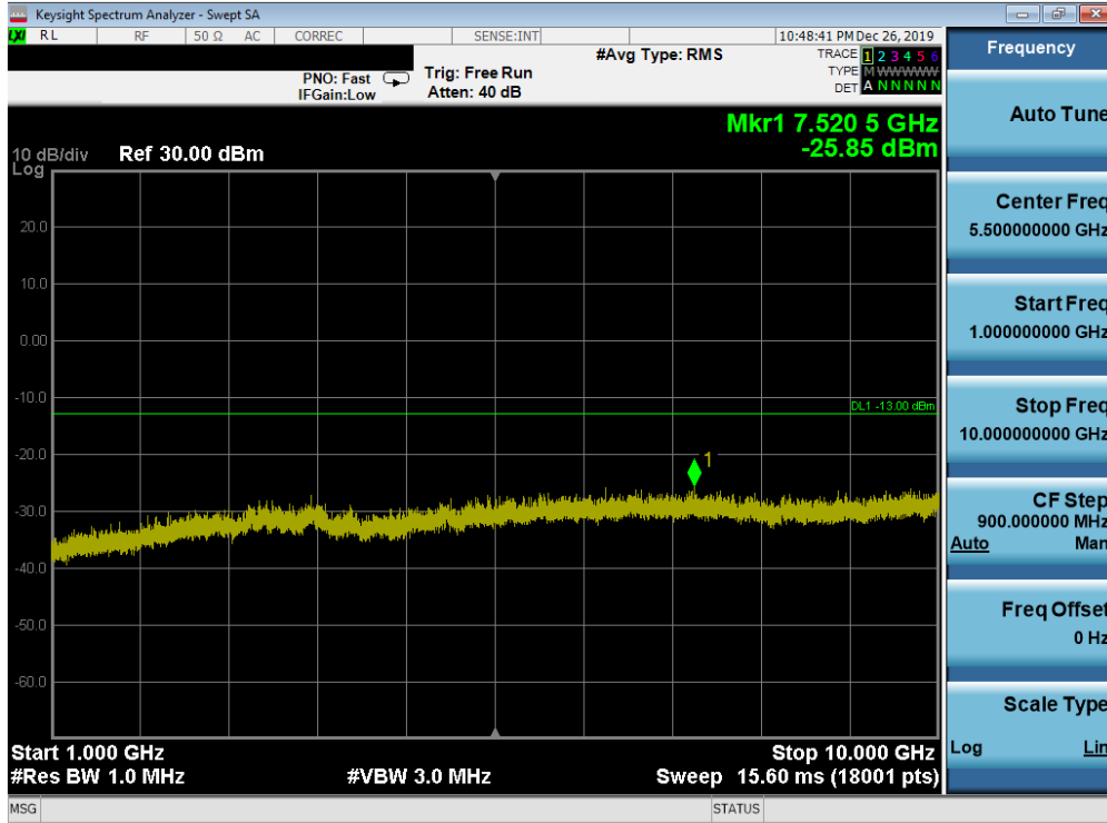
Plot 7-18. Conducted Spurious Plot (Cellular GSM Mode - High Channel)
