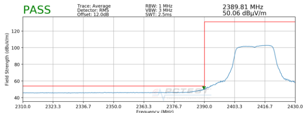
Plot 7-43. Radiated Restricted Lower Band Edge Measurement (Average)
