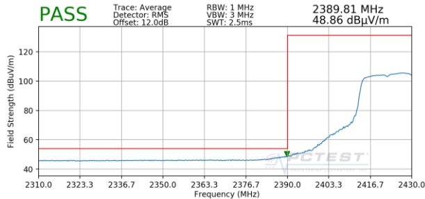
Plot 7-47. Radiated Restricted Lower Band Edge Measurement (Average)
