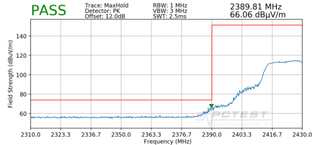
Plot 7-48. Radiated Restricted Lower Band Edge Measurement (Peak)
