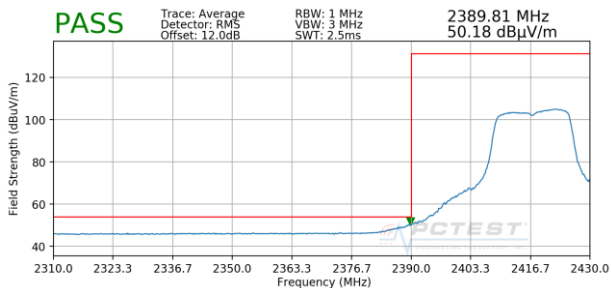
Plot 7-45. Radiated Restricted Lower Band Edge Measurement (Average)
