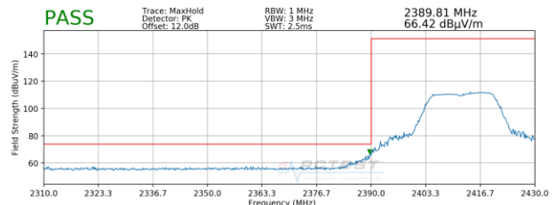
Plot 7-44. Radiated Restricted Lower Band Edge Measurement (Peak)
