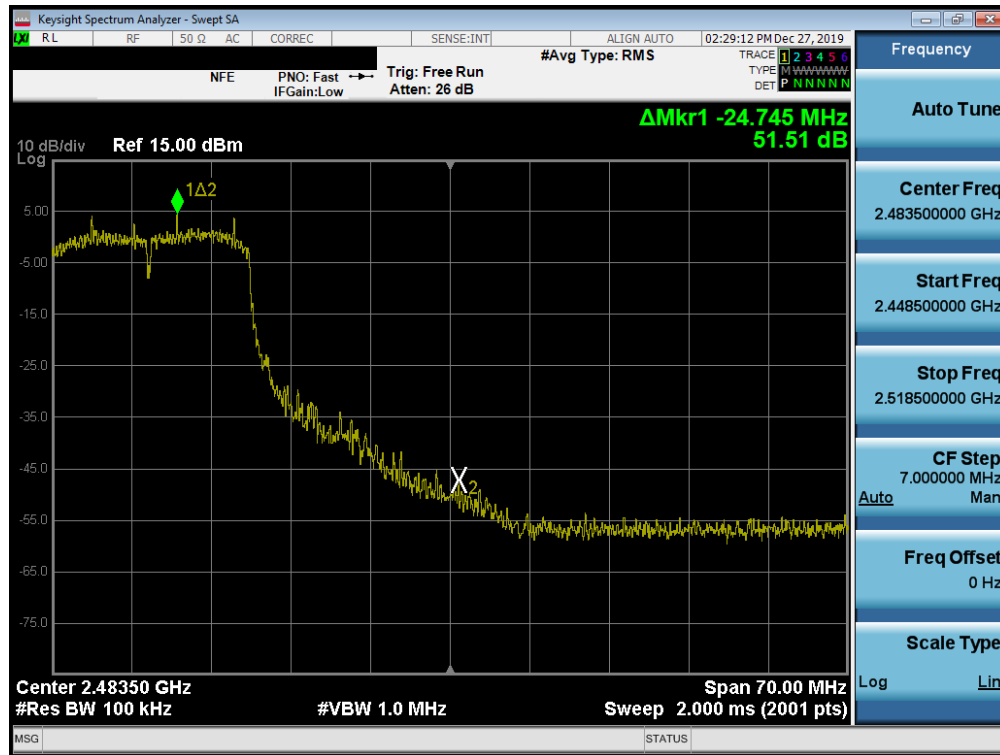
Plot 7-31. Band Edge Plot (802.11n (2.4GHz) – Ch. 10)
