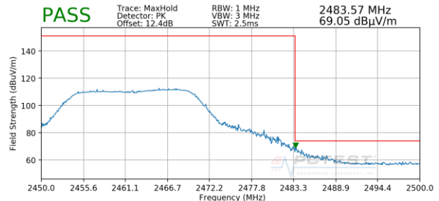
Plot 7-54. Radiated Restricted Upper Band Edge Measurement (Peak)
