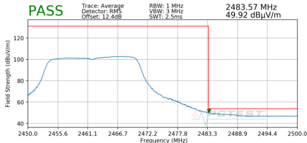
Plot 7-53. Radiated Restricted Upper Band Edge Measurement (Average)
