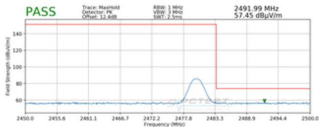
Plot 7-21. Radiated Restricted Upper Band Edge Measurement (Peak - Closed)
