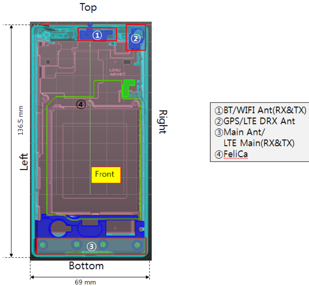
Figure 13.2 Identification of Sides for SAR Testing (Front Side View)
