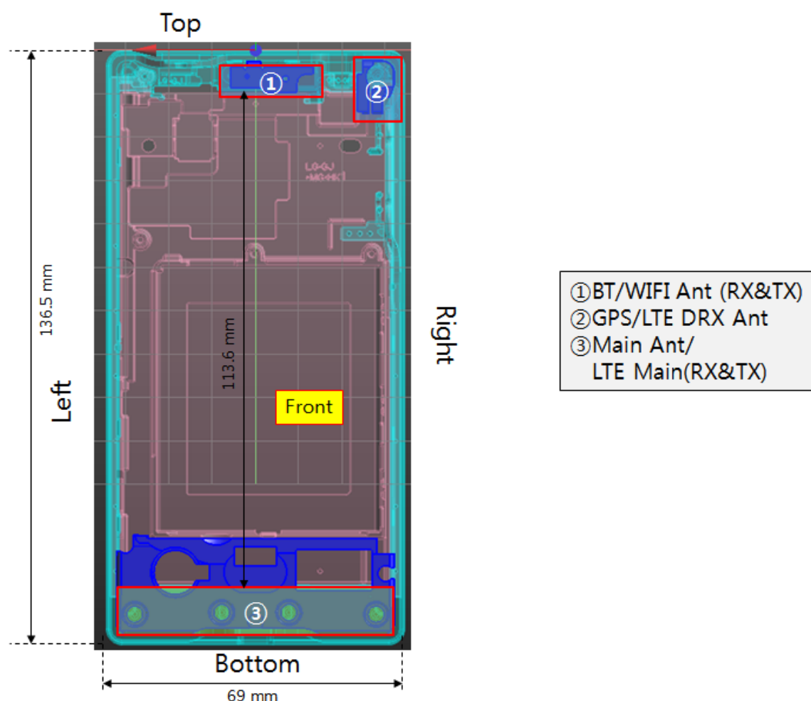
Figure 13.1 Identification of Sides for SAR Testing (Front Side View)
