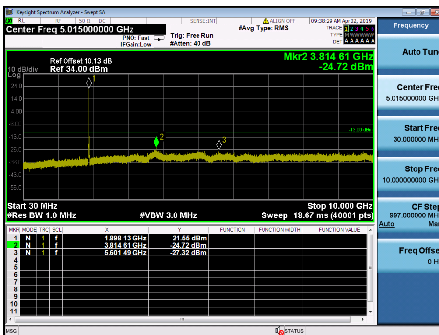
LTE Band 2 / 15MHz / 64QAM - RB Size/Offset (36/0) – High Channel
