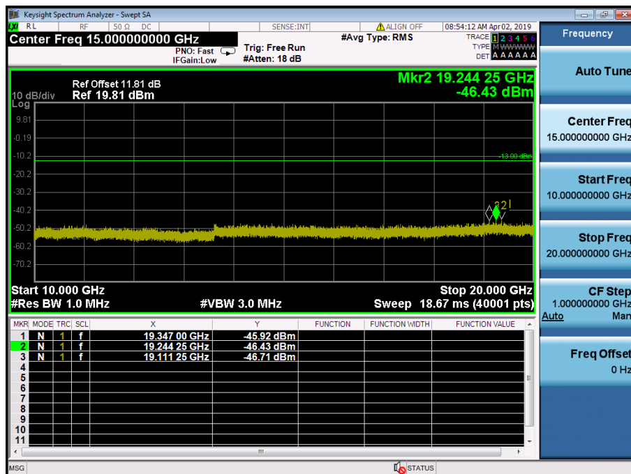
LTE Band 2 / 10MHz / 64QAM - RB Size/Offset (1/49) – High Channel
