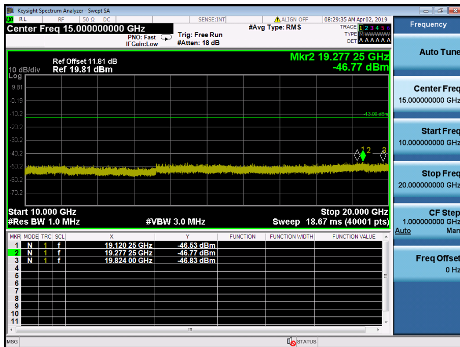
LTE Band 2 / 10MHz / 64QAM - RB Size/Offset (1/49) – Low Channel
