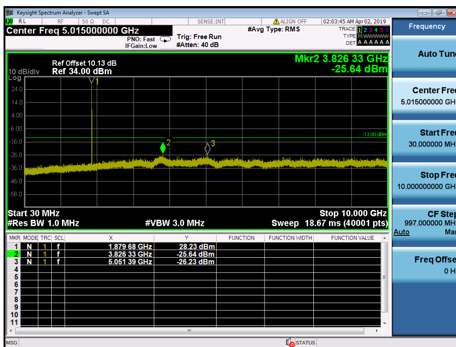
LTE Band 2 / 1.4MHz / 16QAM - RB Size/Offset (3/0) – Mid Channel
