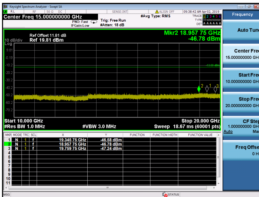
LTE Band 2 / 15MHz / 64QAM - RB Size/Offset (36/0) – High Channel
