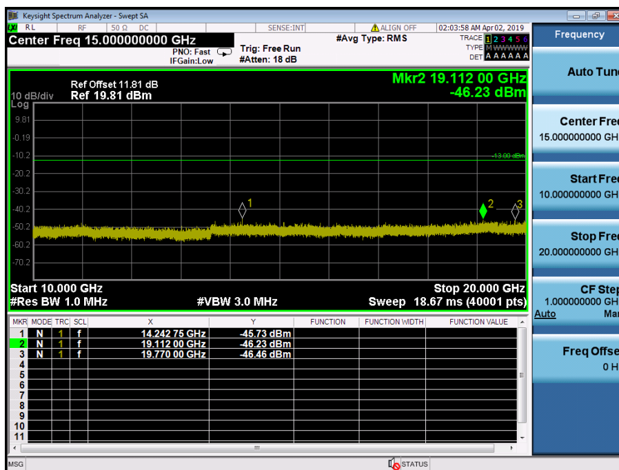
LTE Band 2 / 1.4MHz / 16QAM - RB Size/Offset (3/0) – Mid Channel
