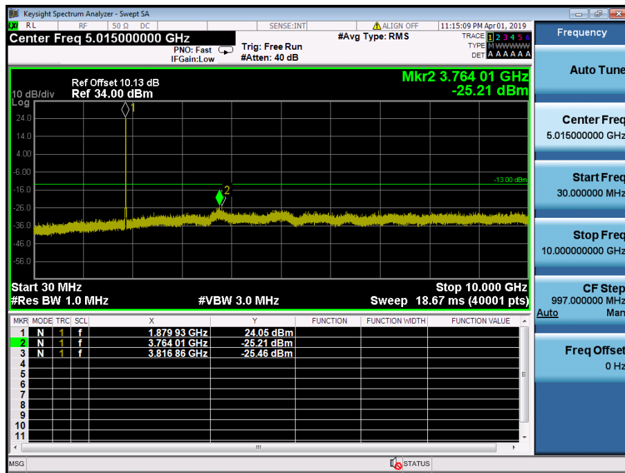
LTE Band 2 / 5MHz / QPSK - RB Size/Offset (25/0) – Mid Channel
