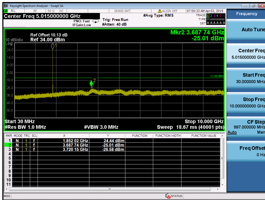
LTE Band 2 / 5MHz / 64QAM - RB Size/Offset (12/6) – Low Channel
