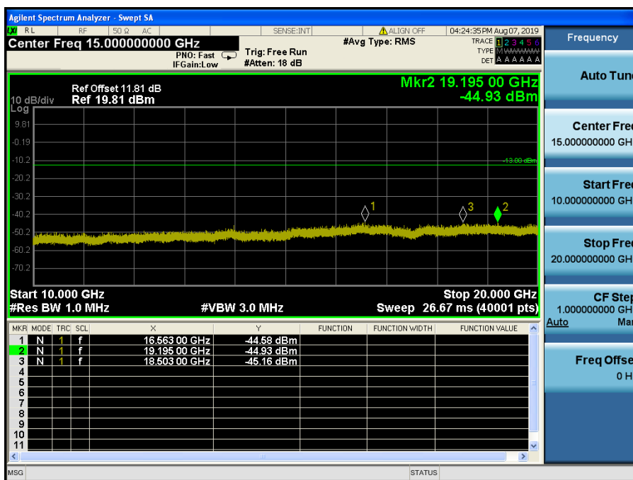
LTE Band 2 / 5MHz / 64QAM - RB Size/Offset (12/0) – Mid Channel
