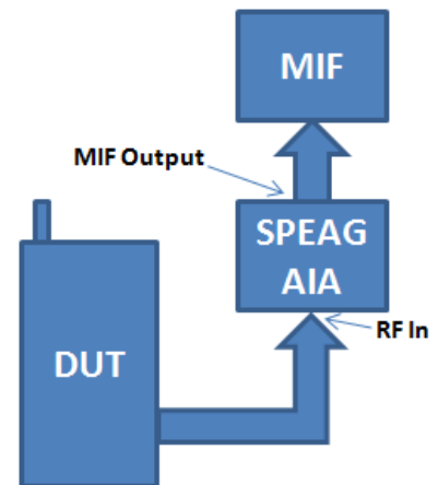
Figure 7-2 MIF Measurement Setup for unlicensed modes
