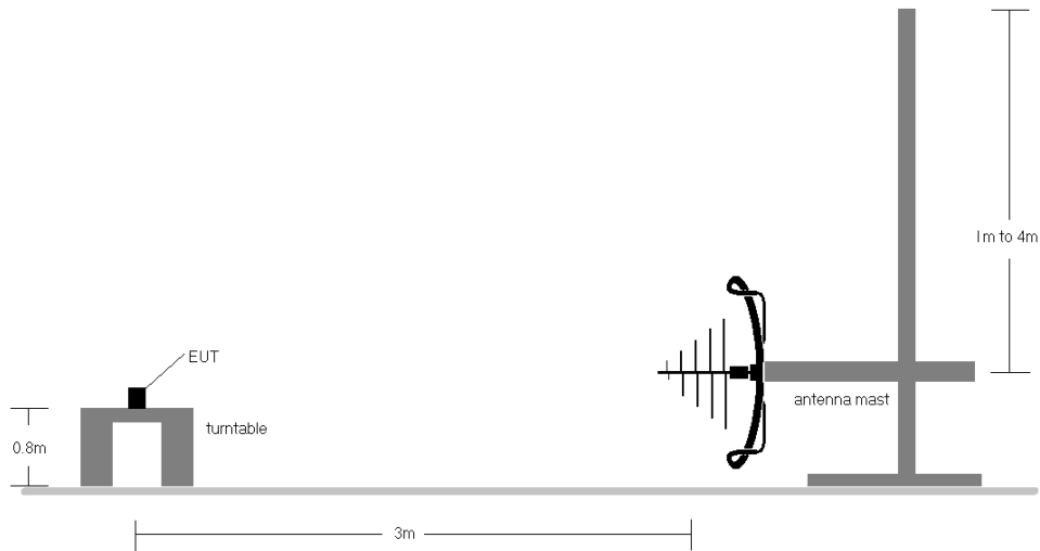
Figure 7-2. Test Instrument & Measurement Setup < 1GHz
