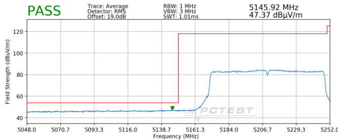
Plot 7-227. Radiated Lower Band Edge Plot MIMO (Average – UNII Band 1)
