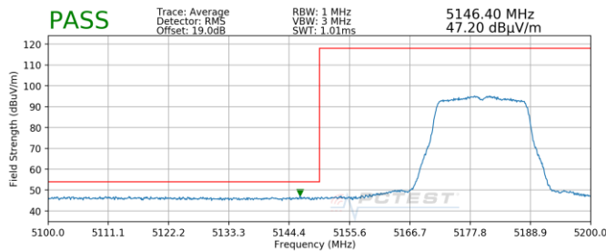
Plot 7-213. Radiated Lower Band Edge Plot MIMO (Average – UNII Band 1)
