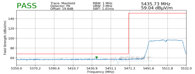
Plot 7-183. Radiated Lower Band Edge Plot SISO ANT1 (Peak – UNII Band 2C)
