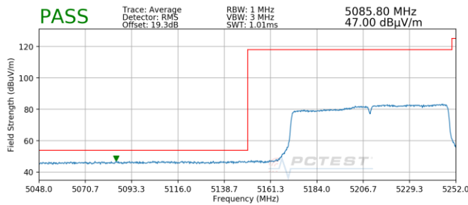
Plot 7-206. Radiated Lower Band Edge Plot SISO ANT2 (Average – UNII Band 1)
