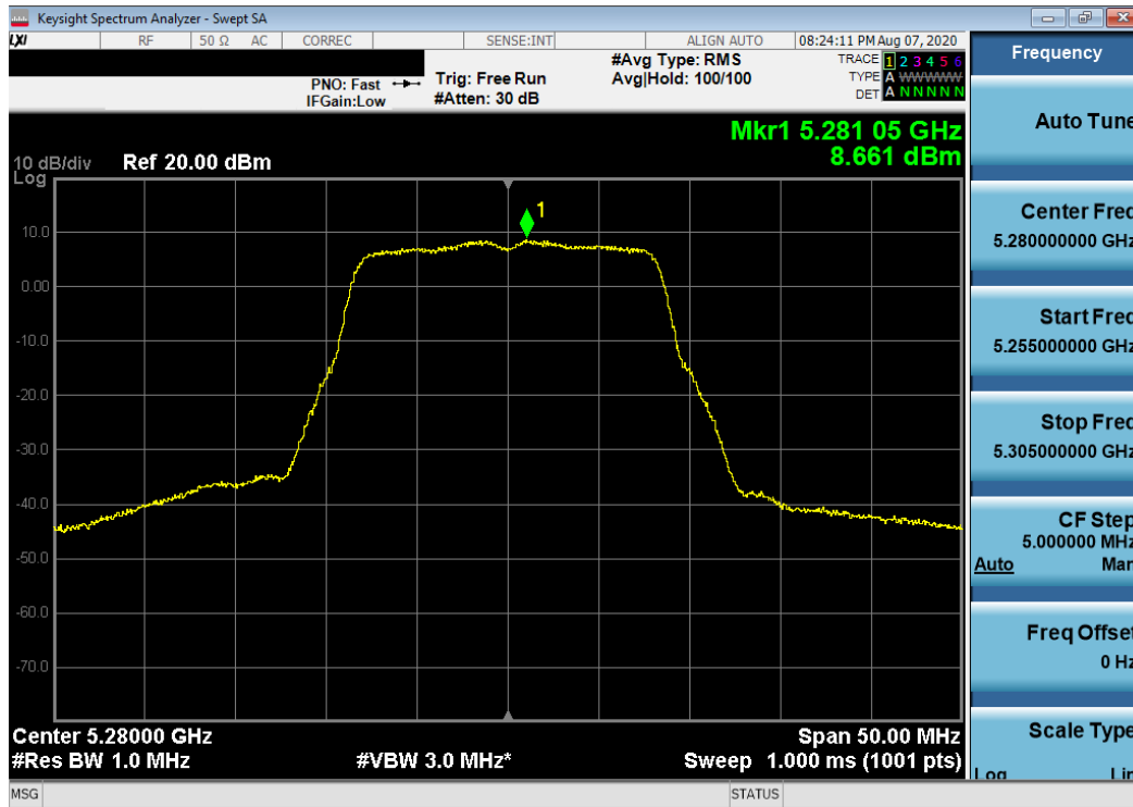
Plot 7-128. Power Spectral Density Plot SISO ANT2 (802.11a (UNII Band 2A) – Ch. 56)
