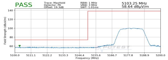
Plot 7-193. Radiated Lower Band Edge Plot SISO ANT2 (Peak – UNII Band 1)
