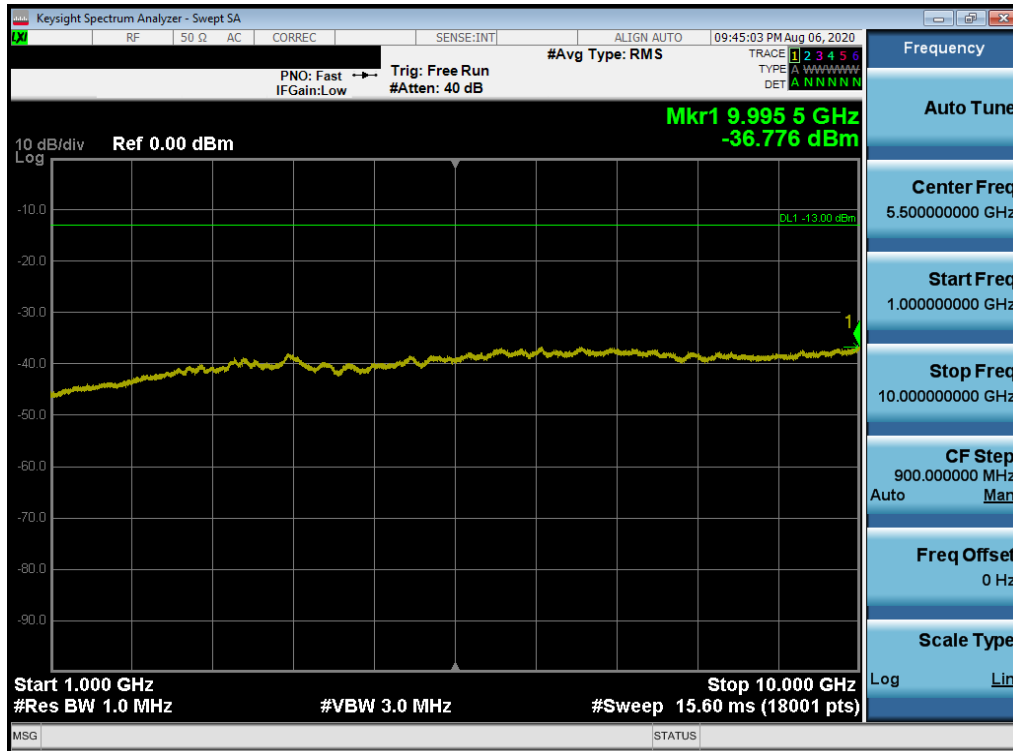
Plot 7-182. Conducted Spurious Plot (LTE Band 12/17 - 10MHz QPSK - RB Size 1, RB Offset 0 - Low Channel)
