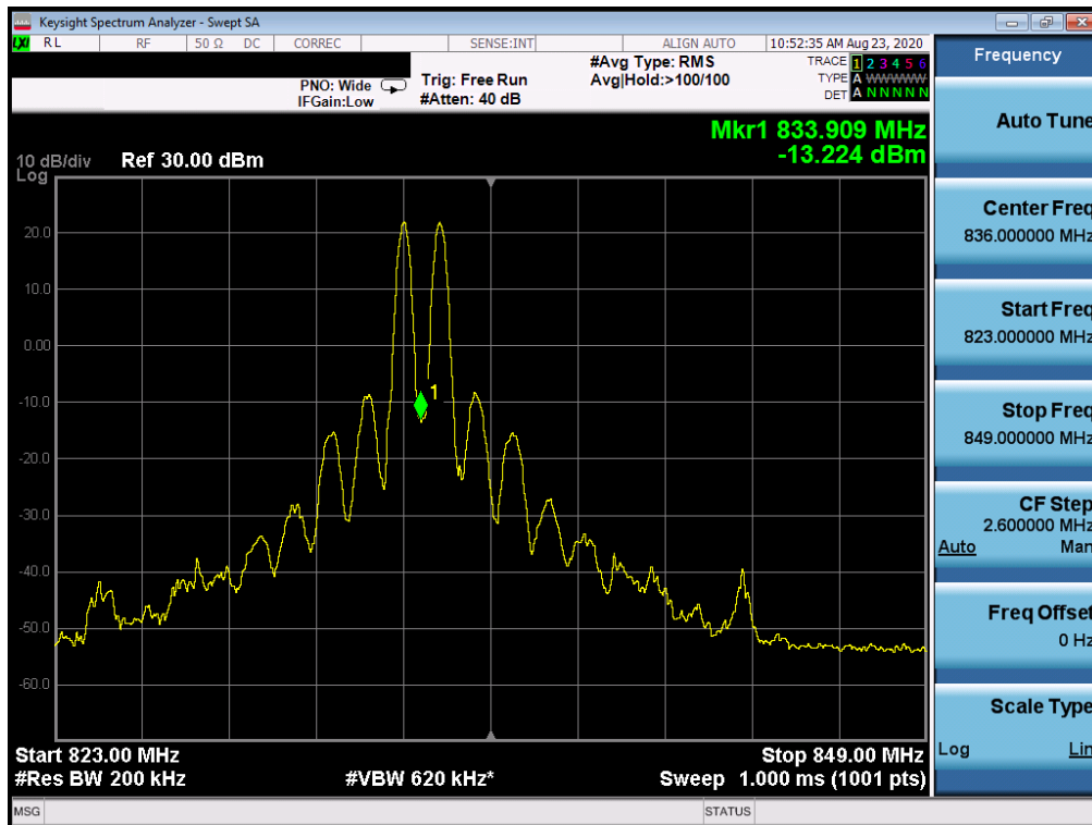
Plot 7-211. Conducted Spurious Plot (ULCA LTE Band 5 – (10 + 10)MHz QPSK – PCC 1/49 SCC 1/0 - Low Channel)
