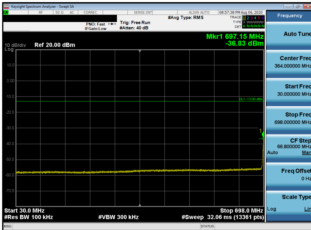
Plot 7-183. Conducted Spurious Plot (LTE Band 12/17 - 10MHz QPSK - RB Size 1, RB Offset 0 - Mid Channel)
