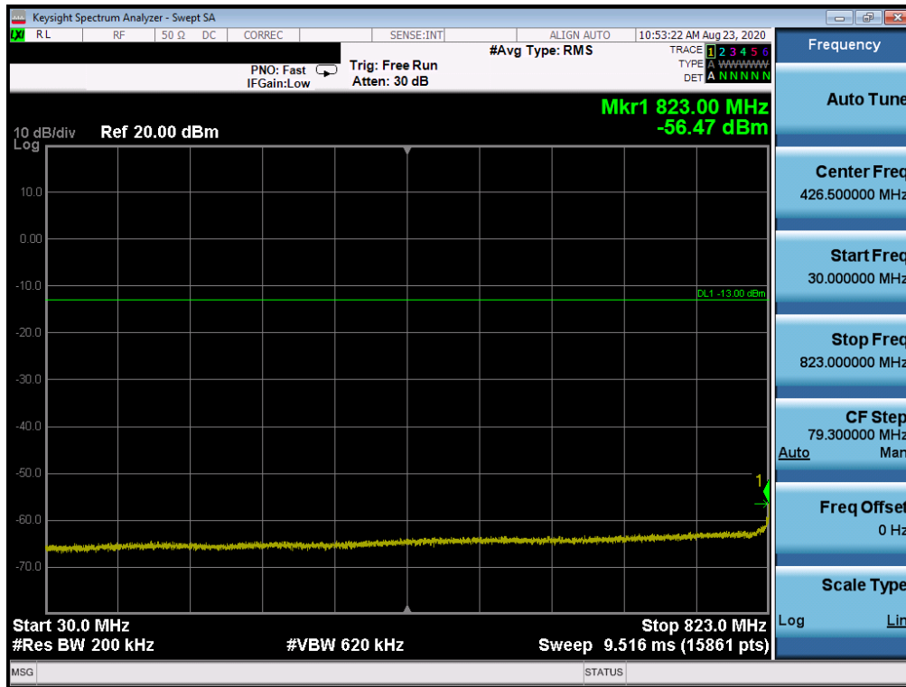
Plot 7-210. Conducted Spurious Plot (ULCA LTE Band 5 – (10 + 10)MHz QPSK – PCC 1/49 SCC 1/0 - Low Channel)
