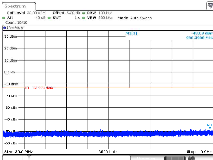
Band4-20MHz-QPSK-20050-1RB#0-Range1:30~1000MHz
