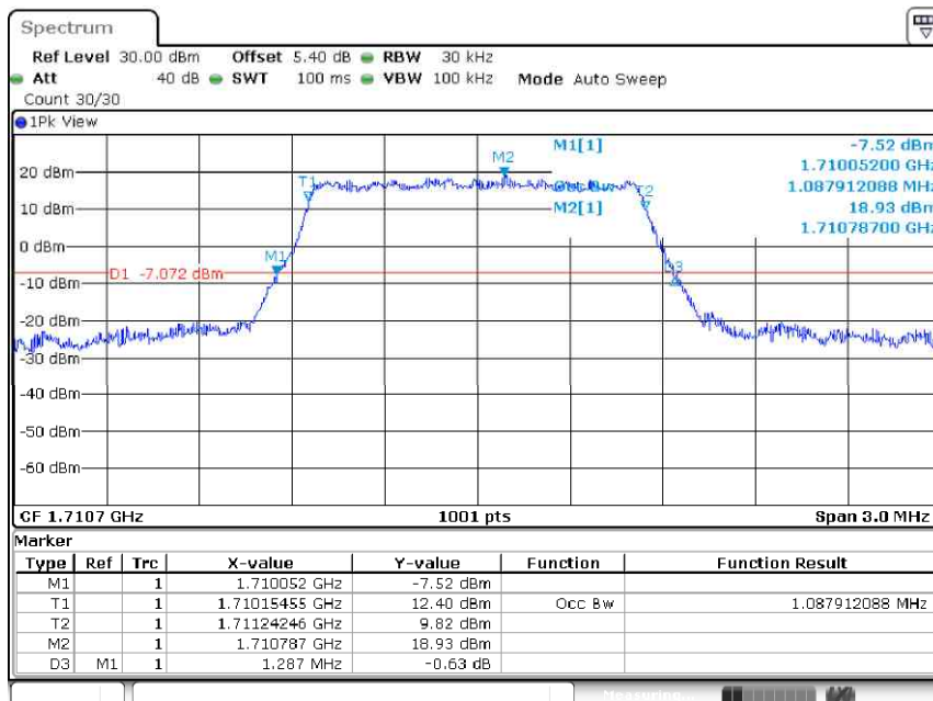
Band66-1.4MHz-QPSK-131979-6RB#0-1.088
