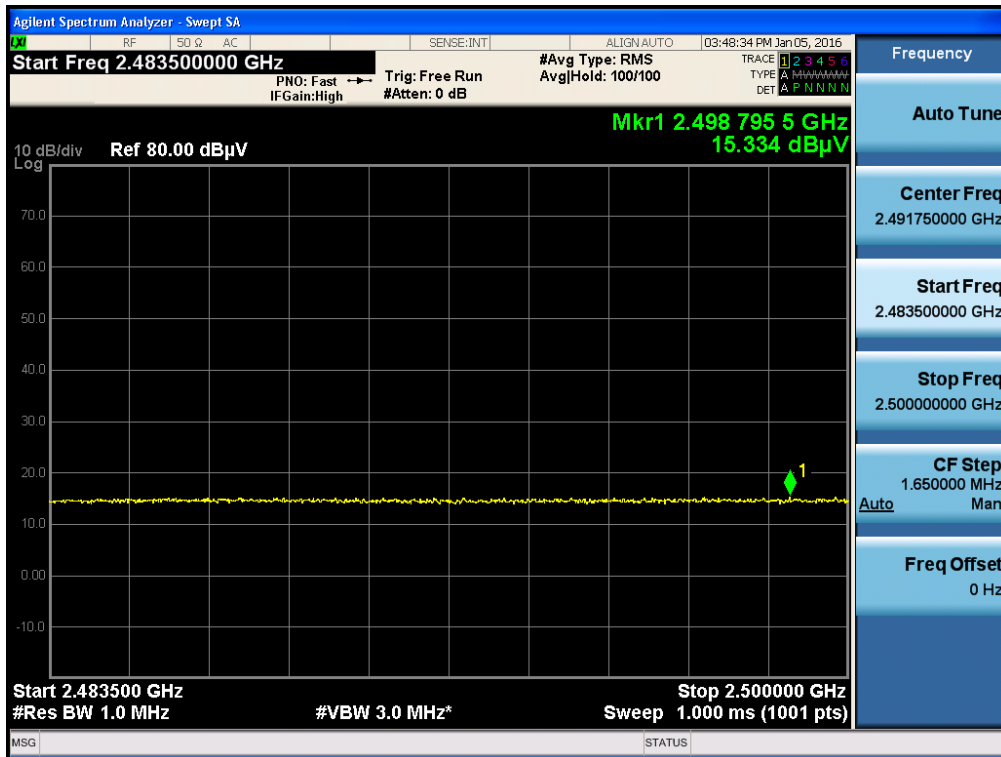
Radiated Restricted Band Edges plot – Average Reading (LE, High Ch.)
