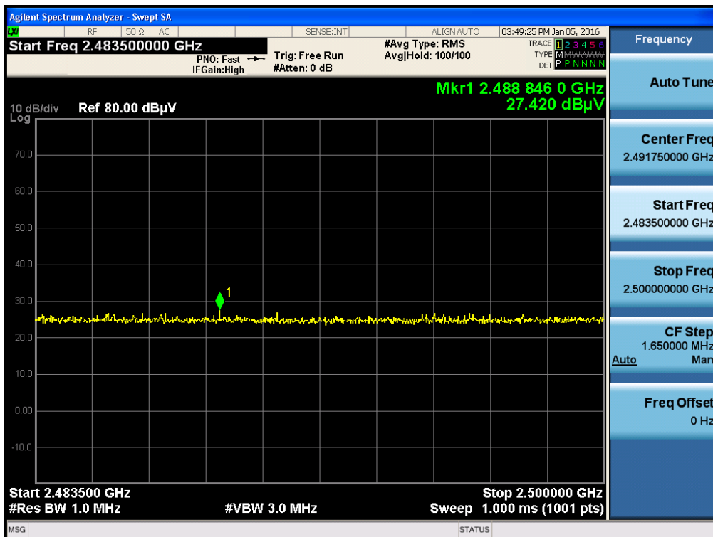
Radiated Restricted Band Edges plot – Peak Reading (LE, High Ch.)
