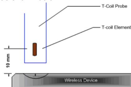
Figure 5-11 Measurement Distance
