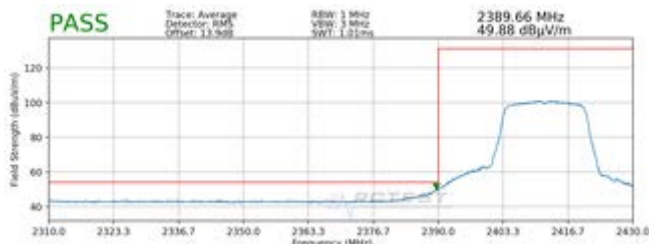
Plot 7-35. Radiated Restricted Lower Band Edge Measurement (Average)
