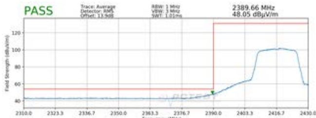
Plot 7-37. Radiated Restricted Lower Band Edge Measurement (Average)
