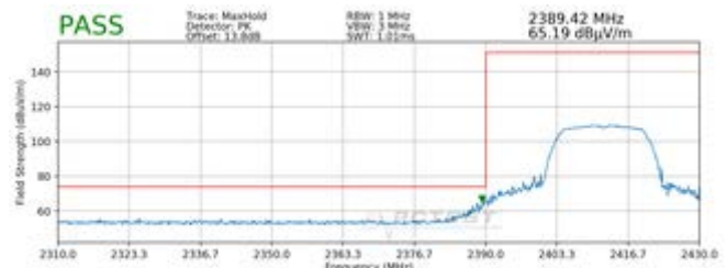
Plot 7-36. Radiated Restricted Lower Band Edge Measurement (Peak)
