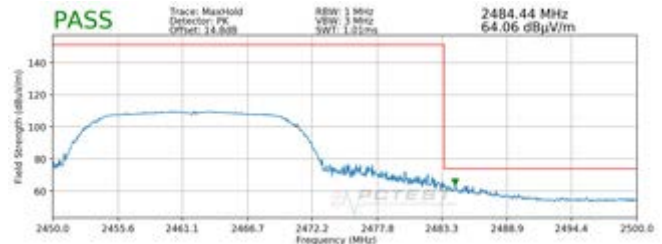
Plot 7-42. Radiated Restricted Upper Band Edge Measurement (Peak)
