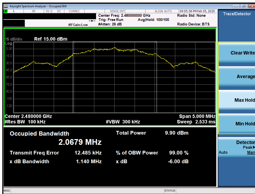
Plot 7-12. 6dB Bandwidth Plot (Bluetooth (LE), 2Mbps – Ch. 39)
