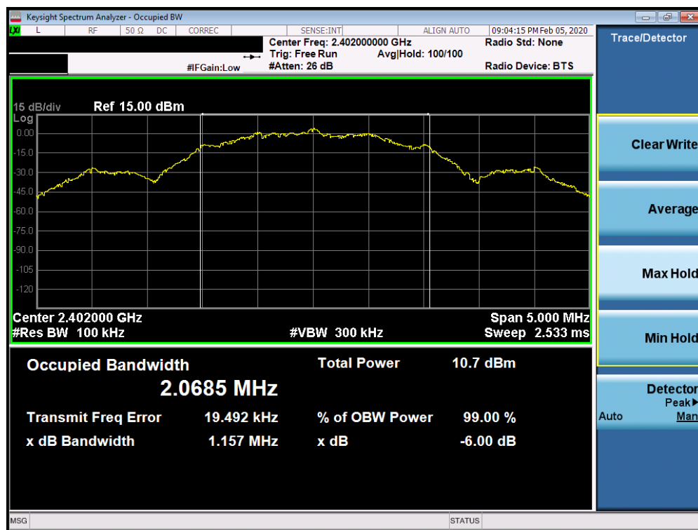
Plot 7-10. 6dB Bandwidth Plot (Bluetooth (LE), 2Mbps – Ch. 0)
