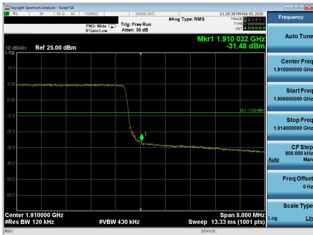
Plot 7-184. Upper Band Edge Plot (Band 2 - 10.0MHz QPSK - Full RB Configuration)
