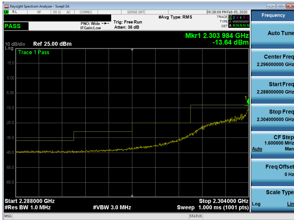
Plot 7-195. Lower Extended Band Edge Plot (Band 30 - 5.0MHz QPSK - Full RB Configuration)
