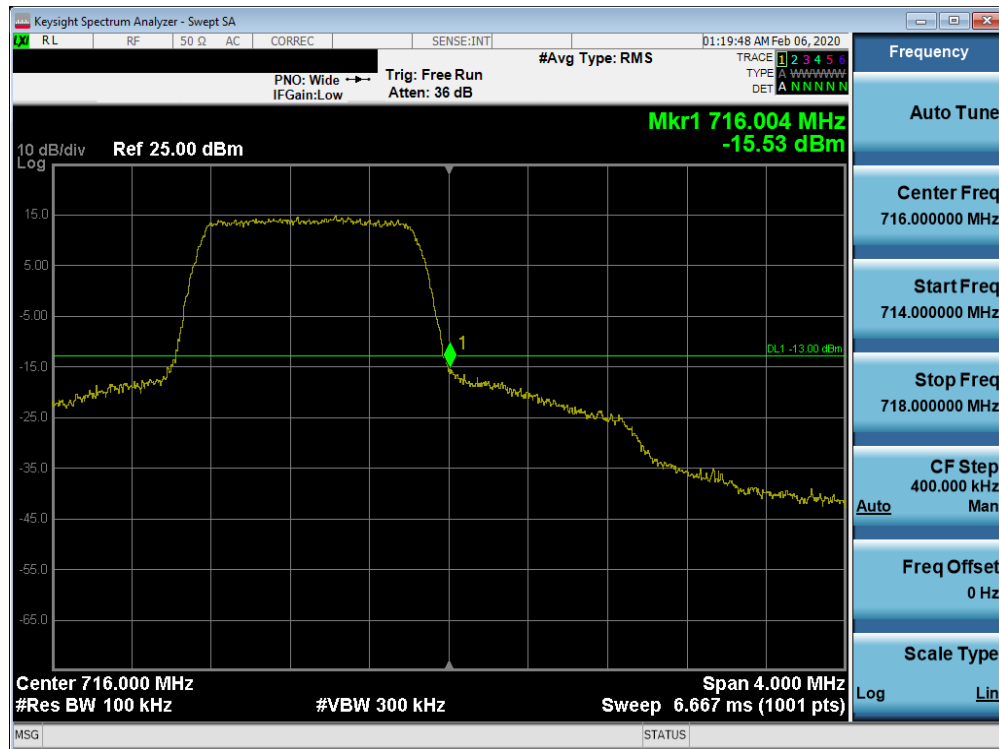
Plot 7-109. Upper Band Edge Plot (Band 12 - 1.4MHz QPSK - Full RB Configuration)
