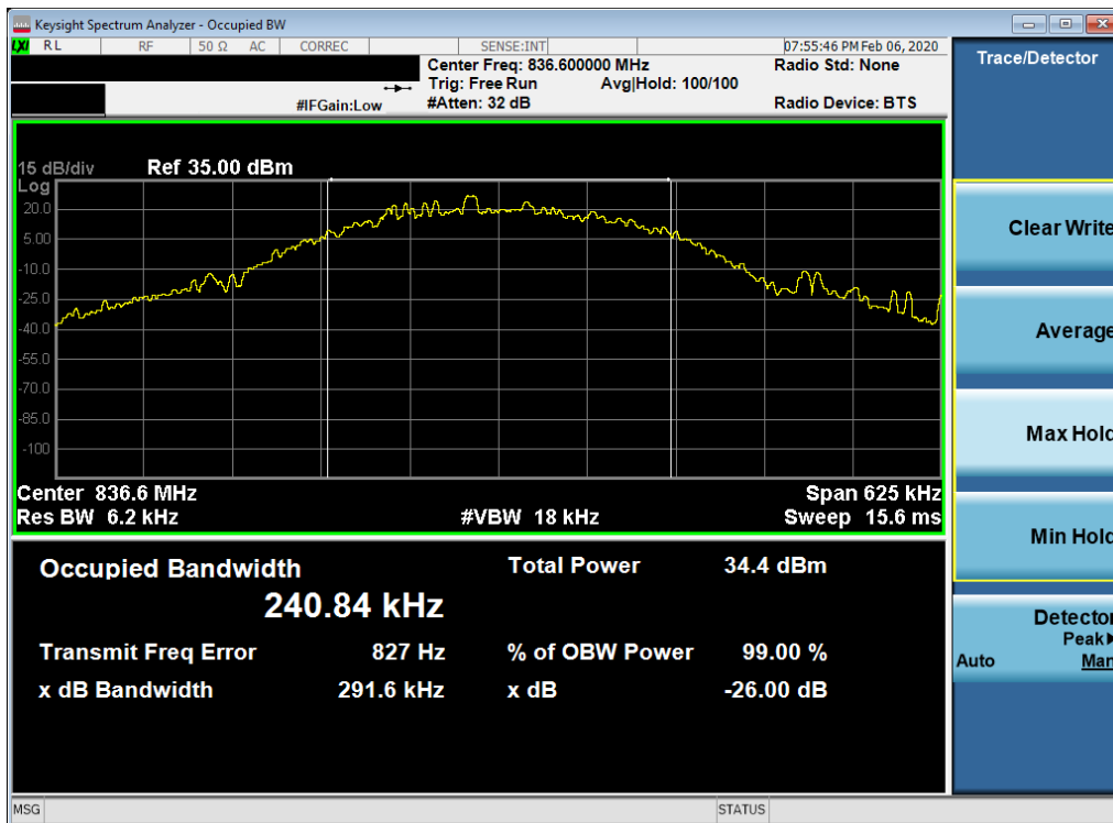
Plot 7-2. Occupied Bandwidth Plot (EDGE850 Mode)
