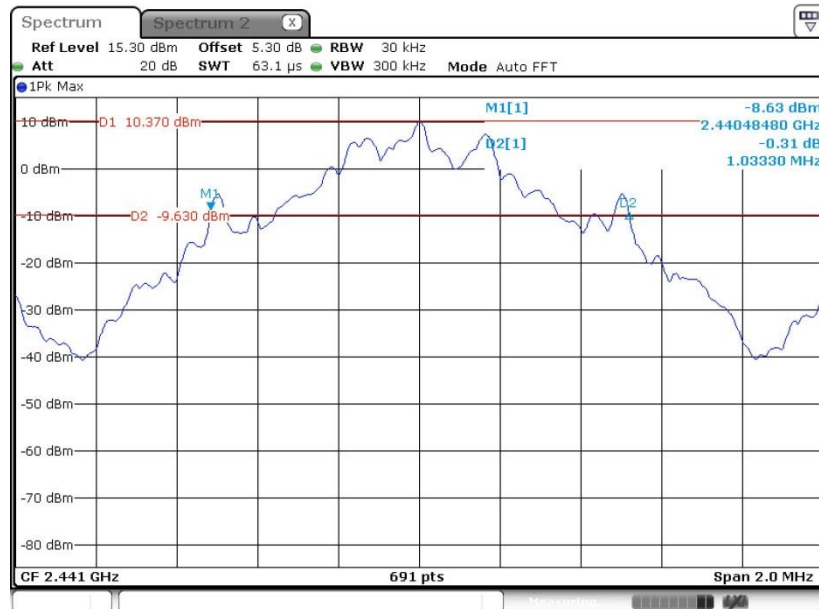
20 dB Bandwidth Plot on Channel 39
