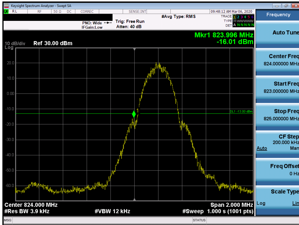
Plot 7-9. Band Edge Plot (Cellular GSM Mode – Low Channel)
