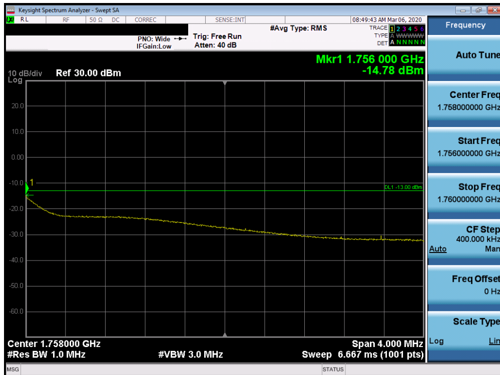
Plot 7-9. 4MHz Span Plot (AWS WCDMA Mode – High Channel)
