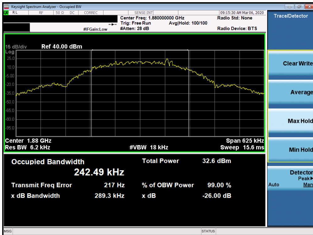
Plot 7-5. Occupied Bandwidth Plot (EDGE1900 Mode)
