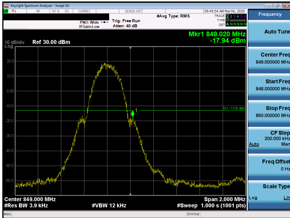
Plot 7-9. Band Edge Plot (Cellular GSM Mode – High Channel)
