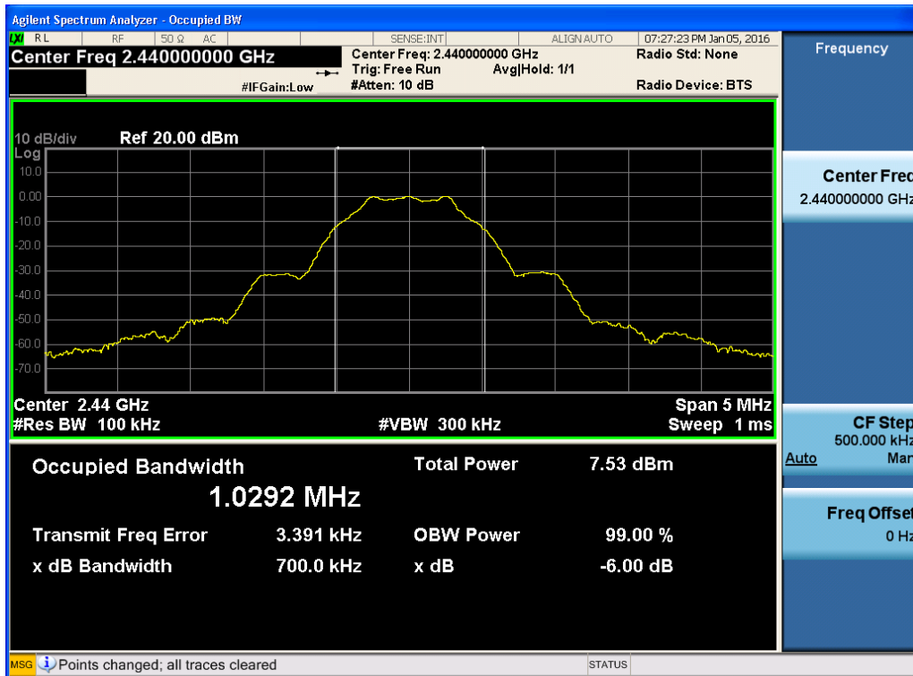
6dB Bandwidth plot (Mid-CH 19)
