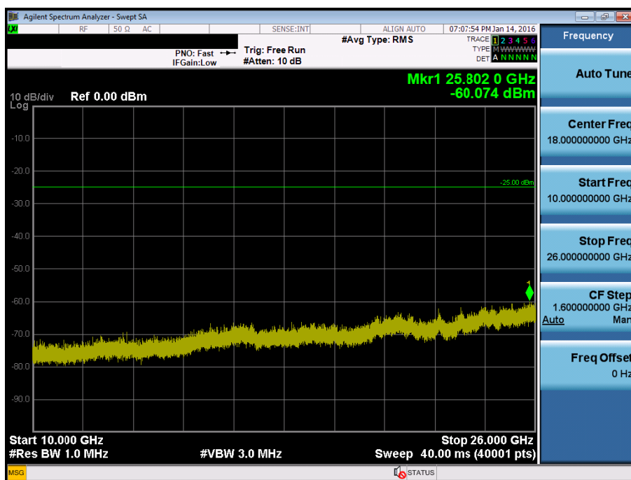
BAND7. Conducted Spurious Plot 2 (5MHz Ch.21425 QPSK RB 1, Offset 0)
