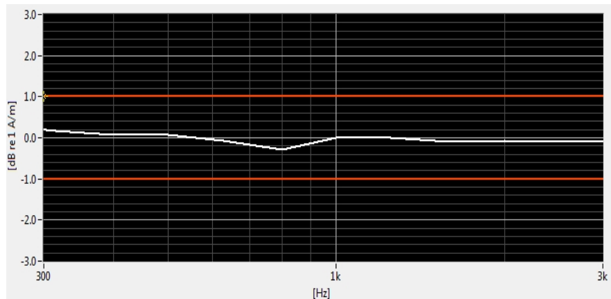
Figure 7-4 Helmholtz Coil Validation for Frequency Response
