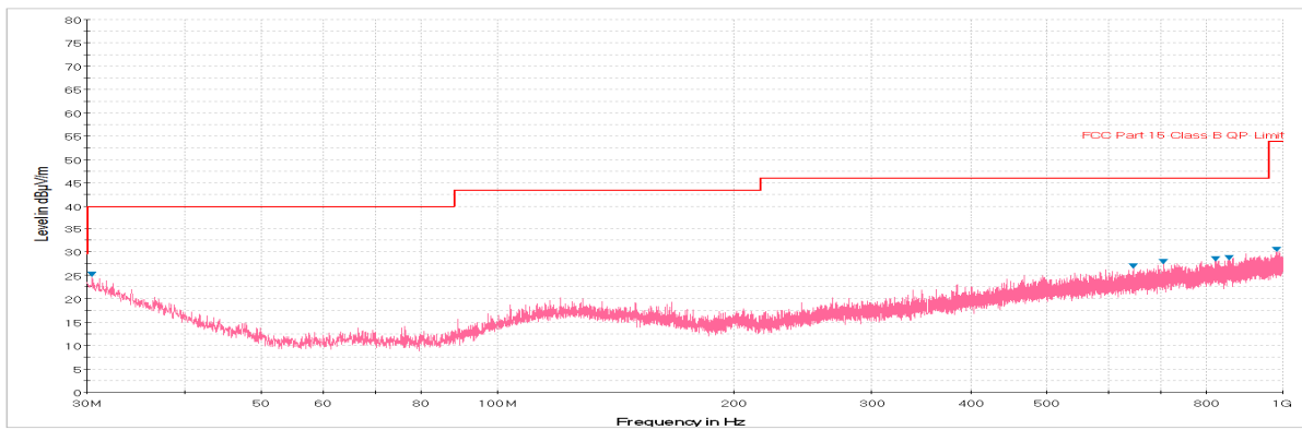
Plot 7-60. Radiated Spurious Plot below 1GHz (Pol. V)
