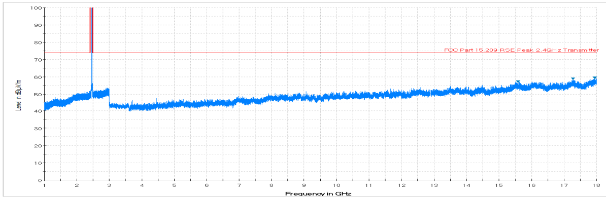
Plot 7-44. Radiated Spurious Plot above 1GHz (802.11b – Ch. 11, Ant. Pol. V)
