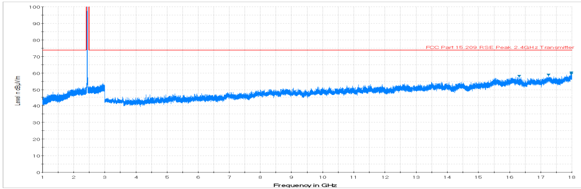
Plot 7-42. Radiated Spurious Plot above 1GHz (802.11b – Ch. 6, Ant. Pol. V)
