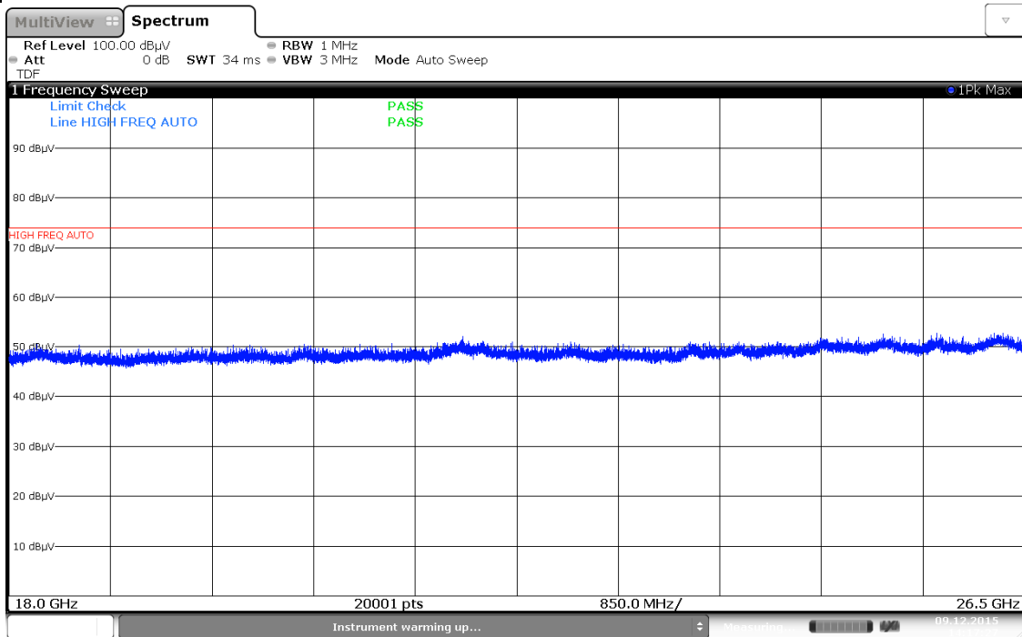
Plot 7-45. Radiated Spurious Plot above 18GHz (Pol. H)
