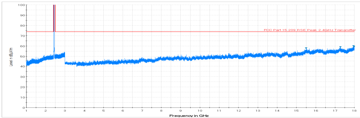
Plot 7-41. Radiated Spurious Plot above 1GHz (802.11b – Ch. 6, Ant. Pol. H)
