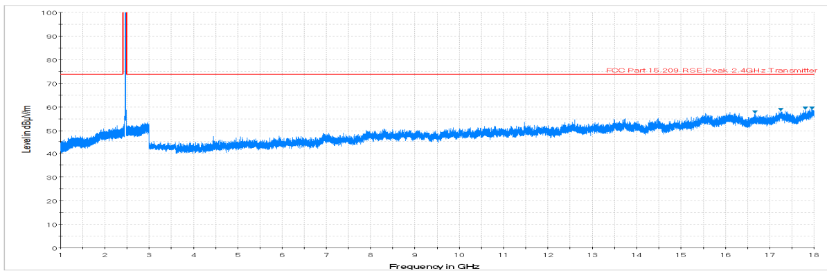
Plot 7-43. Radiated Spurious Plot above 1GHz (802.11b – Ch. 11, Ant. Pol. H)
