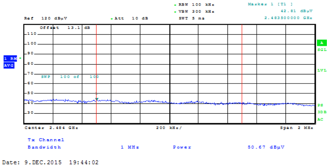
Plot 7-57. Radiated Restricted Upper Band Edge Measurement (Average)
