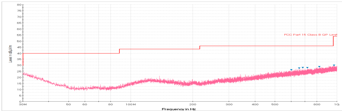
Plot 7-59. Radiated Spurious Plot below 1GHz (Pol. H)
