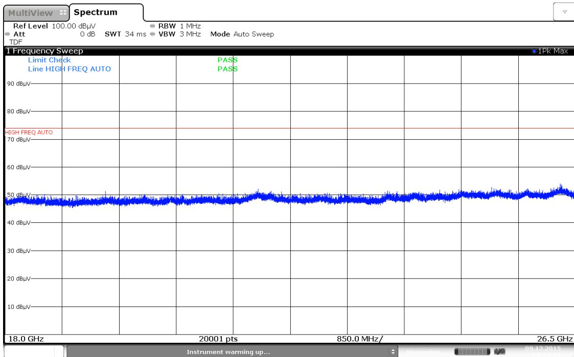
Plot 7-46. Radiated Spurious Plot above 18GHz (Pol. V)
