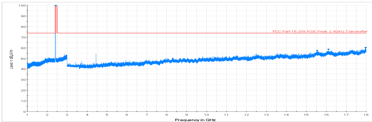
Plot 7-40. Radiated Spurious Plot above 1GHz (802.11b – Ch. 1, Ant. Pol. V)
