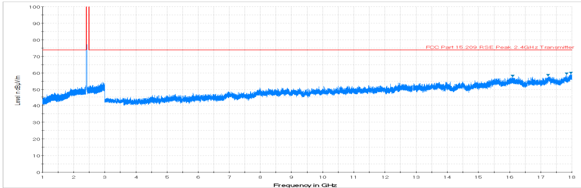
Plot 7-39. Radiated Spurious Plot above 1GHz (802.11b – Ch. 1, Ant. Pol. H)
