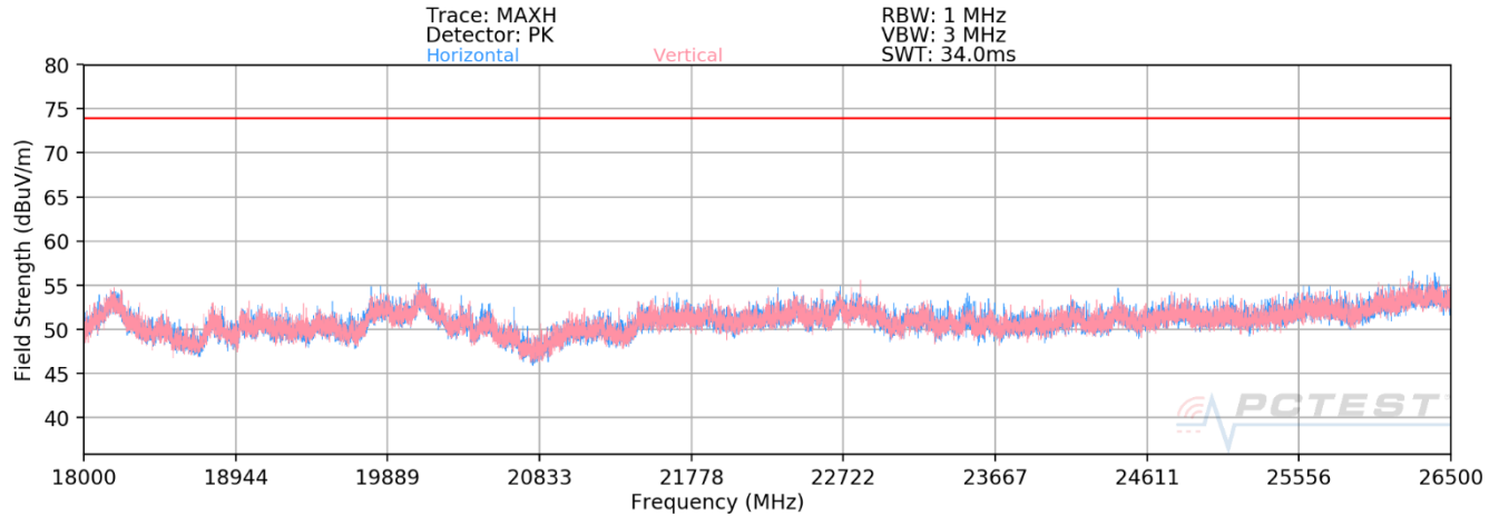
Plot 7-45. Radiated Spurious Plot above 18GHz
