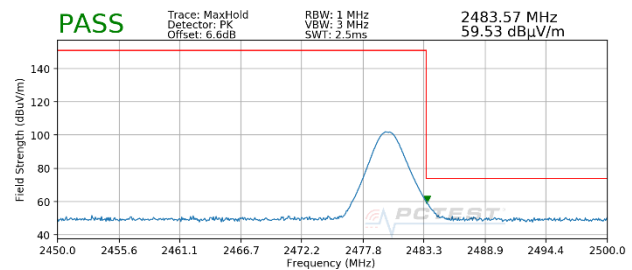
Plot 7-47. Radiated Restricted Upper Band Edge Measurement (Peak)
