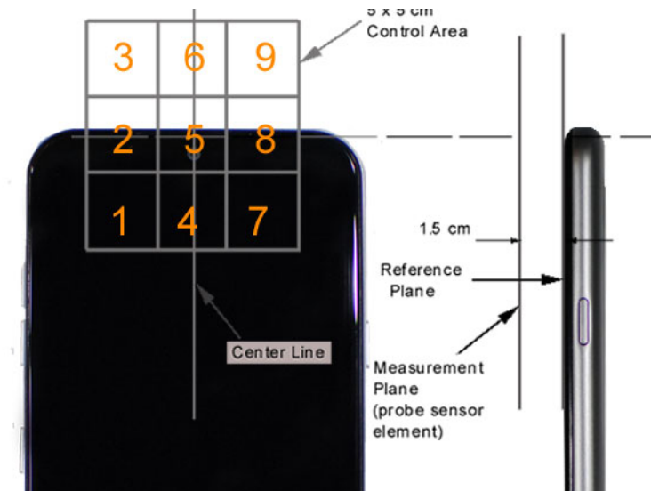
Figure 17-3 5x5 Scan grid above WD (Acoustic centered scan area pictured)
