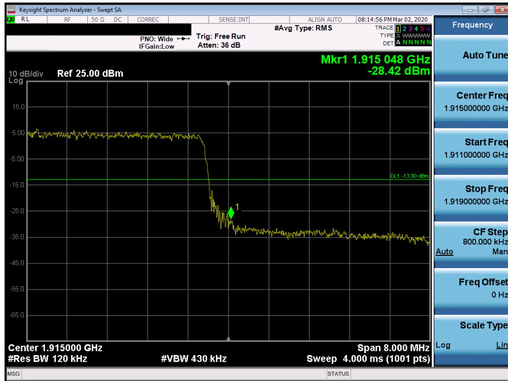
Plot 7-211. Upper Band Edge Plot (Band 25 - 10.0MHz QPSK - Full RB Configuration)
