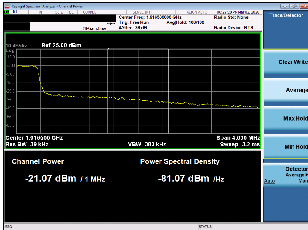
Plot 7-200. Upper Extended Band Edge Plot (Band 25 - 3.0MHz QPSK - Full RB Configuration)
