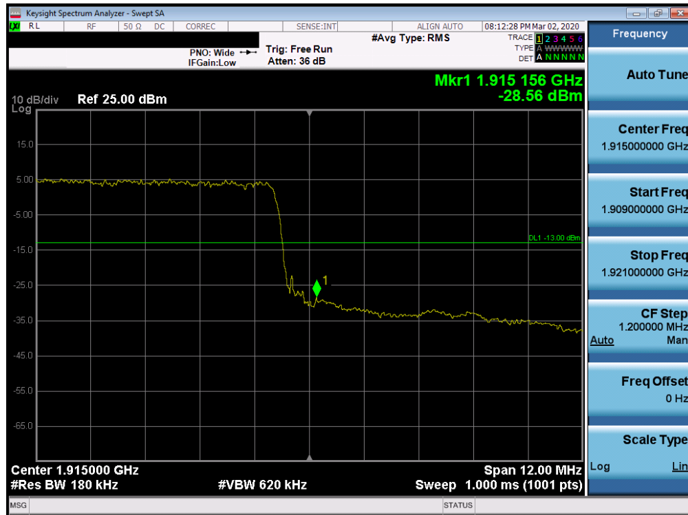
Plot 7-217. Upper Band Edge Plot (Band 25 - 15.0MHz QPSK - Full RB Configuration)
