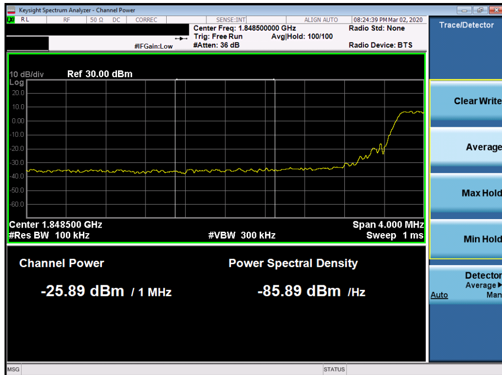
Plot 7-202. Lower Extended Band Edge Plot (Band 25/2 - 5.0MHz QPSK - Full RB Configuration)
