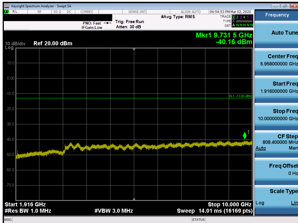
Plot 7-116. Conducted Spurious Plot (Band 25/2 - 20.0MHz QPSK - RB Size 1, RB Offset 0 - High Channel)
