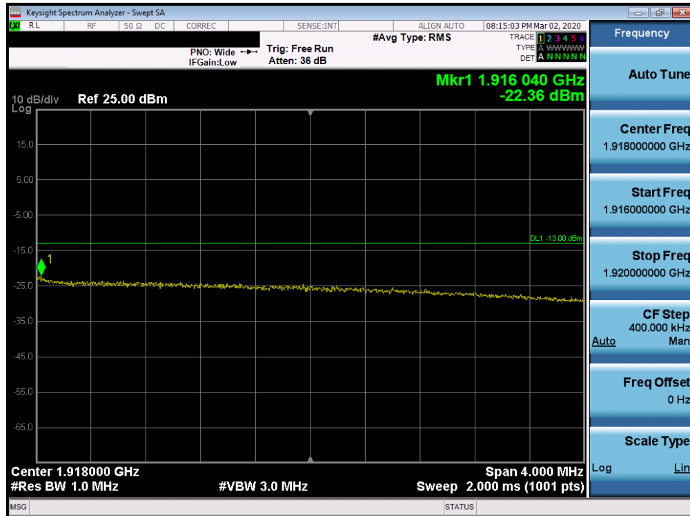
Plot 7-212. Upper Extended Band Edge Plot (Band 25 - 10.0MHz QPSK - Full RB Configuration)
