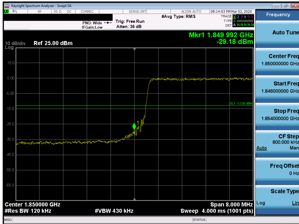
Plot 7-207. Lower Band Edge Plot (Band 25/2 - 10.0MHz QPSK - Full RB Configuration)
