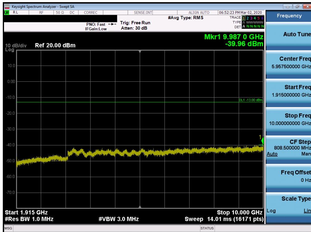
Plot 7-110. Conducted Spurious Plot (Band 25/2 - 20.0MHz QPSK - RB Size 1, RB Offset 0 - Low Channel)
