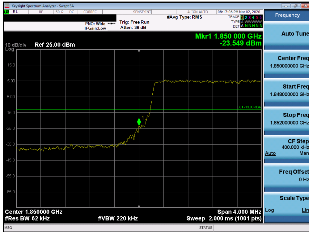
Plot 7-201. Lower Band Edge Plot (Band 25/2 - 5.0MHz QPSK - Full RB Configuration)
