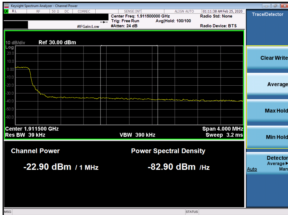
Plot 7-204. Upper Extended Band Edge Plot (Band 2 - 5.0MHz QPSK - Full RB Configuration)
