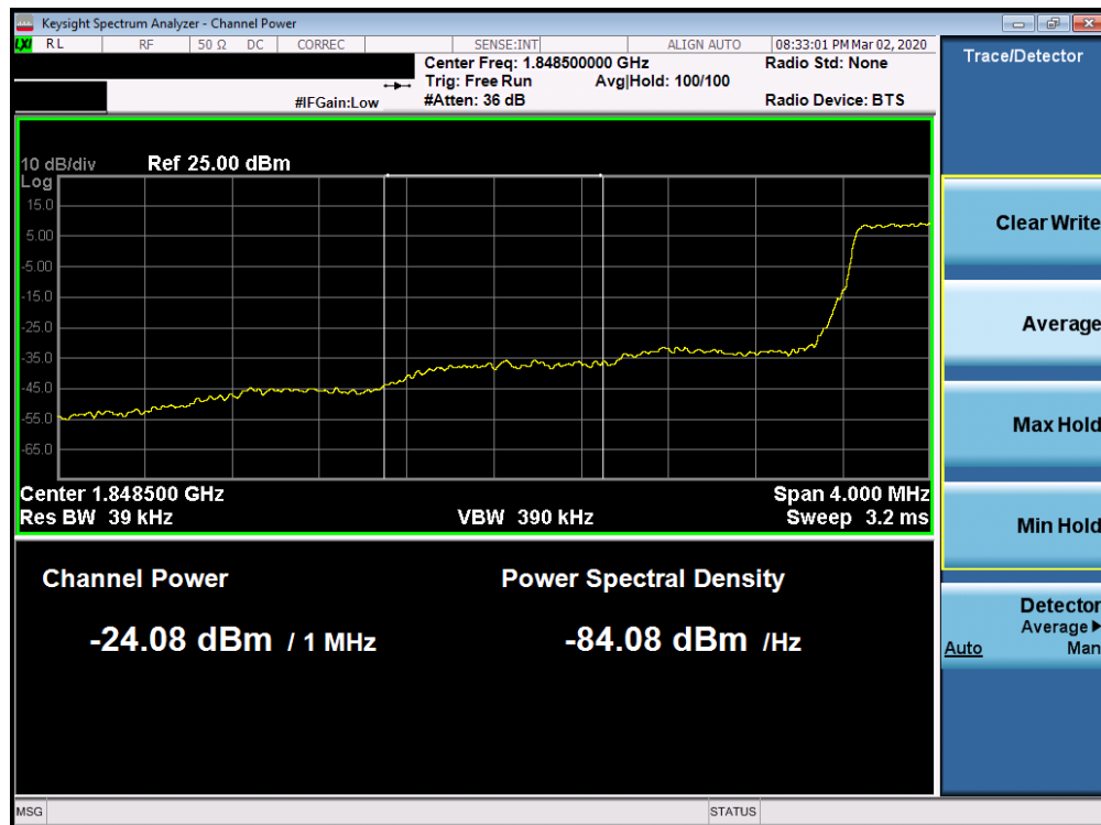
Plot 7-190. Lower Extended Band Edge Plot (Band 25/2 - 1.4MHz QPSK - Full RB Configuration)
