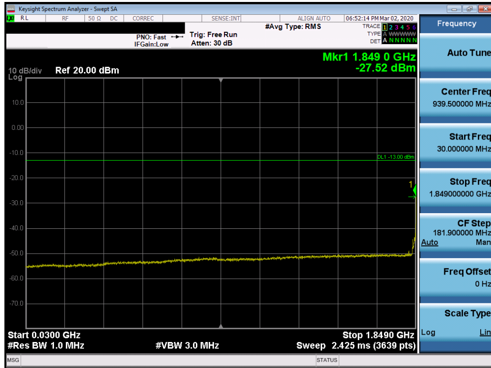
Plot 7-109. Conducted Spurious Plot (Band 25/2 - 20.0MHz QPSK - RB Size 1, RB Offset 0 - Low Channel)
