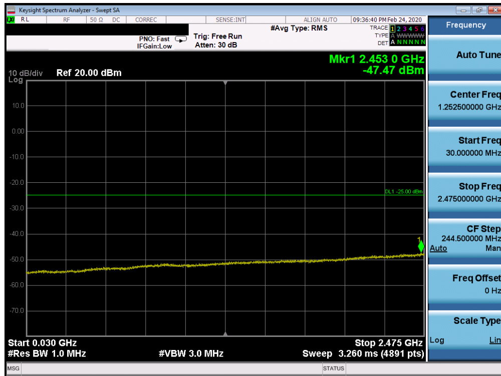
Plot 7-118. Conducted Spurious Plot (Band 7 - 20.0MHz QPSK - RB Size 1, RB Offset 0 - Low Channel)
