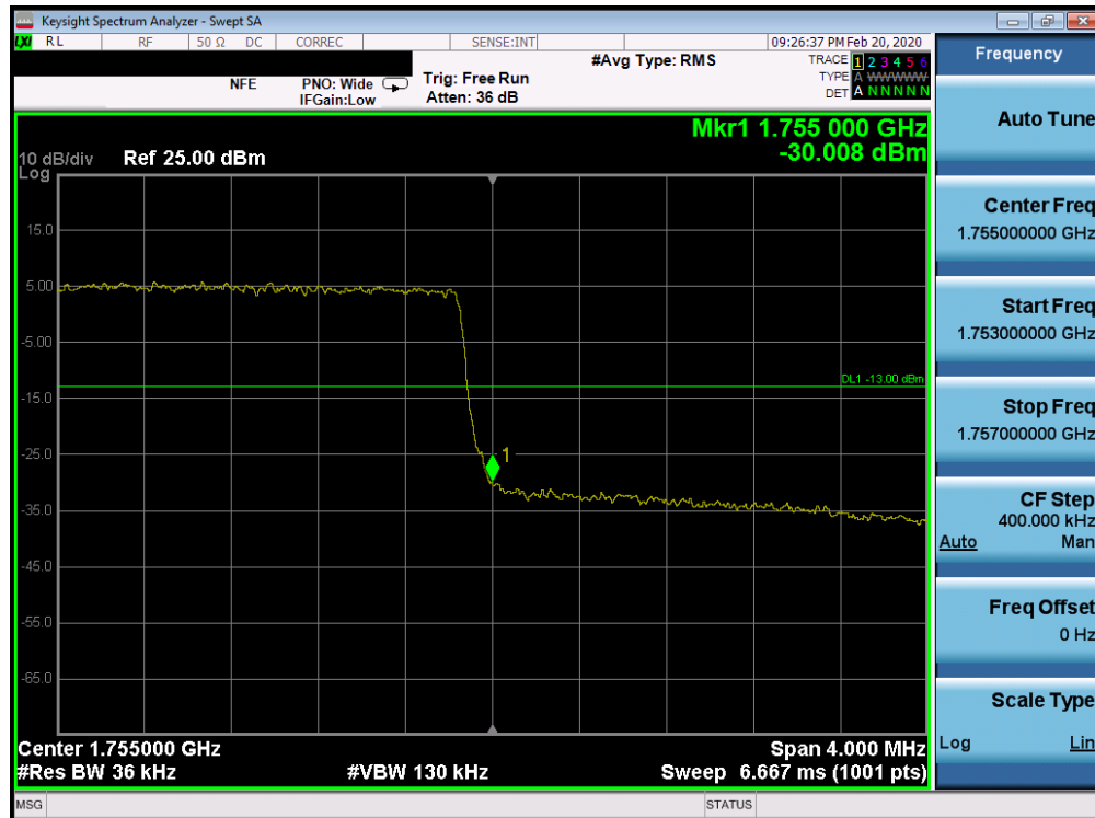
Plot 7-161. Upper Band Edge Plot (Band 4 - 3.0MHz QPSK - Full RB Configuration)
