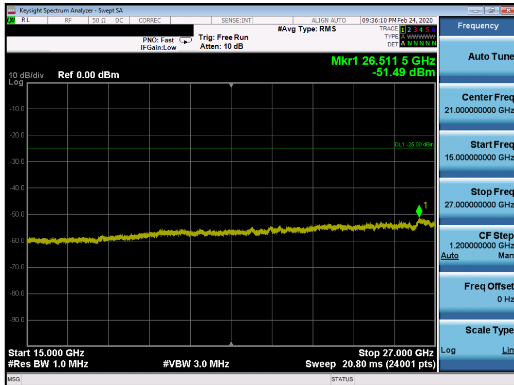
Plot 7-123. Conducted Spurious Plot (Band 7 - 20.0MHz QPSK - RB Size 1, RB Offset 0 - Mid Channel)
