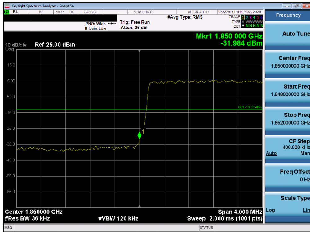
Plot 7-195. Lower Band Edge Plot (Band 25/2 - 3.0MHz QPSK - Full RB Configuration)
