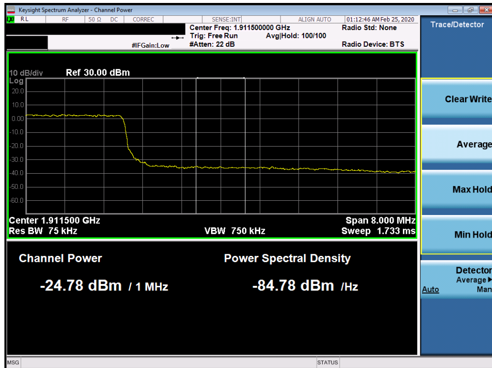
Plot 7-210. Upper Extended Band Edge Plot (Band 2 - 10.0MHz QPSK - Full RB Configuration)
