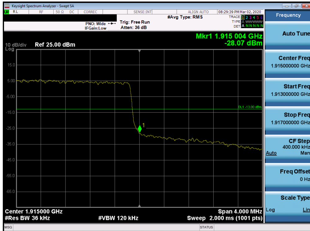
Plot 7-199. Upper Band Edge Plot (Band 25 - 3.0MHz QPSK - Full RB Configuration)
