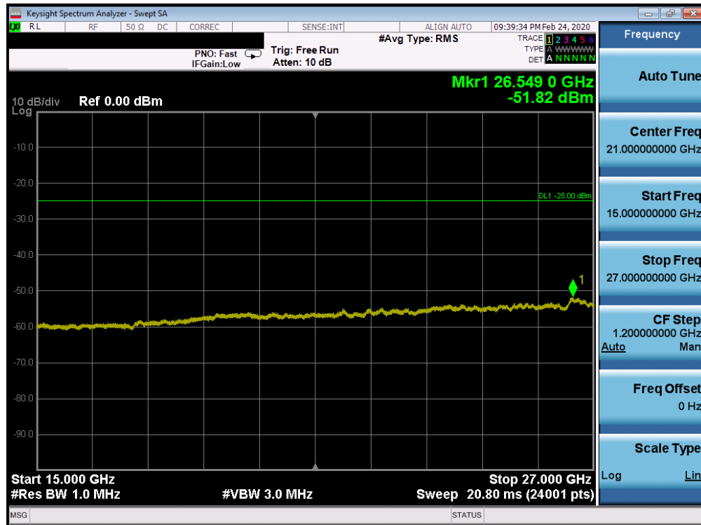
Plot 7-126. Conducted Spurious Plot (Band 7 - 20.0MHz QPSK - RB Size 1, RB Offset 0 - High Channel)
