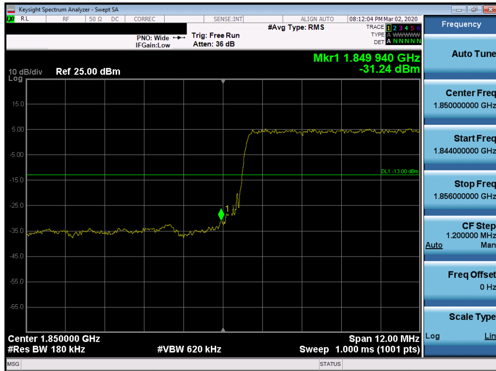
Plot 7-213. Lower Band Edge Plot (Band 25/2 - 15.0MHz QPSK - Full RB Configuration)
