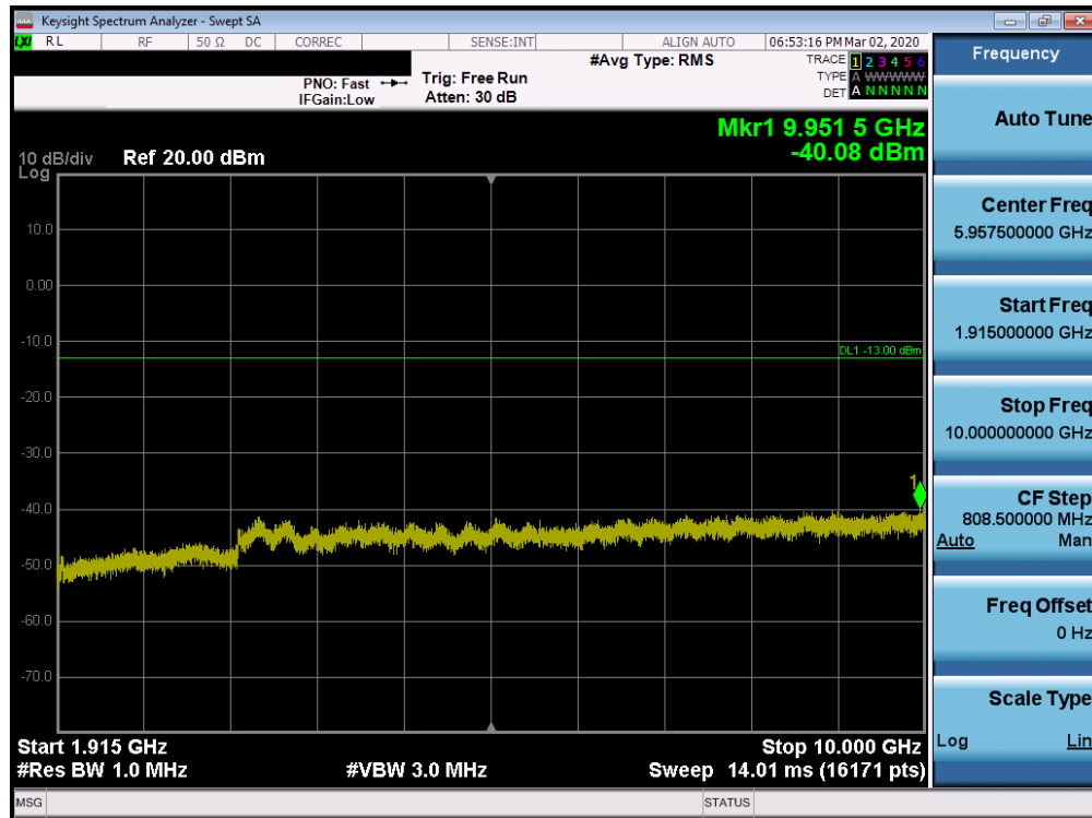
Plot 7-113. Conducted Spurious Plot (Band 25/2 - 20.0MHz QPSK - RB Size 1, RB Offset 0 - Mid Channel)
