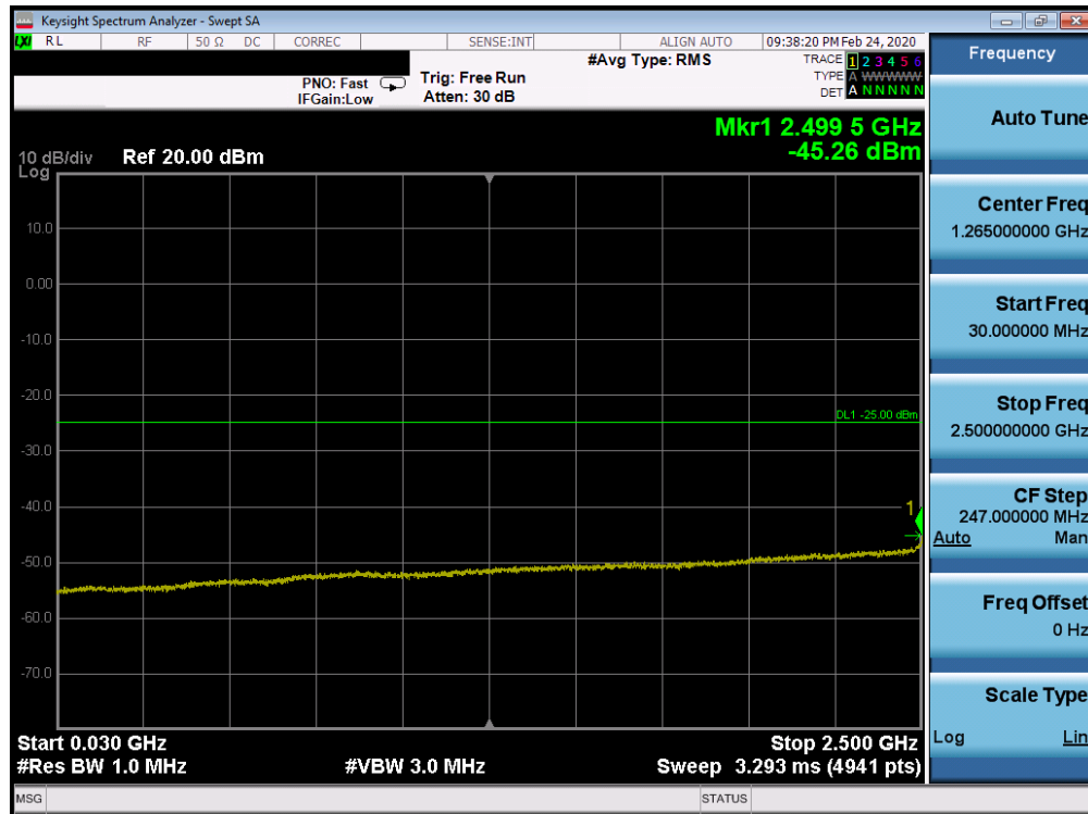
Plot 7-124. Conducted Spurious Plot (Band 7 - 20.0MHz QPSK - RB Size 1, RB Offset 0 - High Channel)
