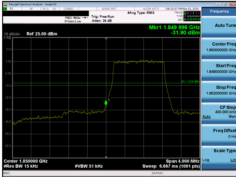
Plot 7-189. Lower Band Edge Plot (Band 25/2 - 1.4MHz QPSK - Full RB Configuration)
