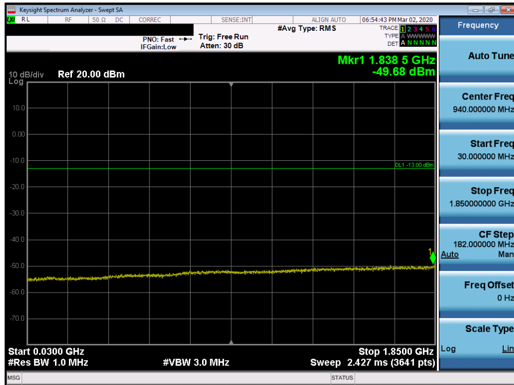
Plot 7-115. Conducted Spurious Plot (Band 25/2 - 20.0MHz QPSK - RB Size 1, RB Offset 0 - High Channel)
