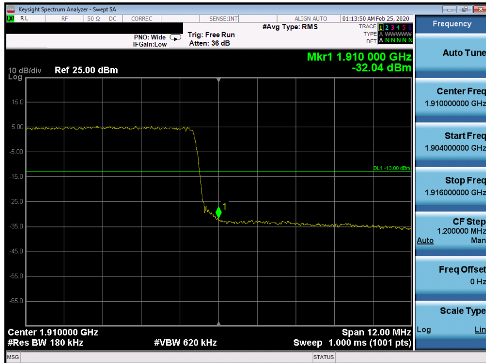
Plot 7-215. Upper Band Edge Plot (Band 2 - 15.0MHz QPSK - Full RB Configuration)
