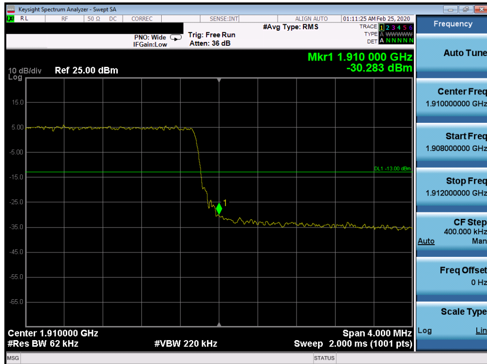
Plot 7-203. Upper Band Edge Plot (Band 2 - 5.0MHz QPSK - Full RB Configuration)
