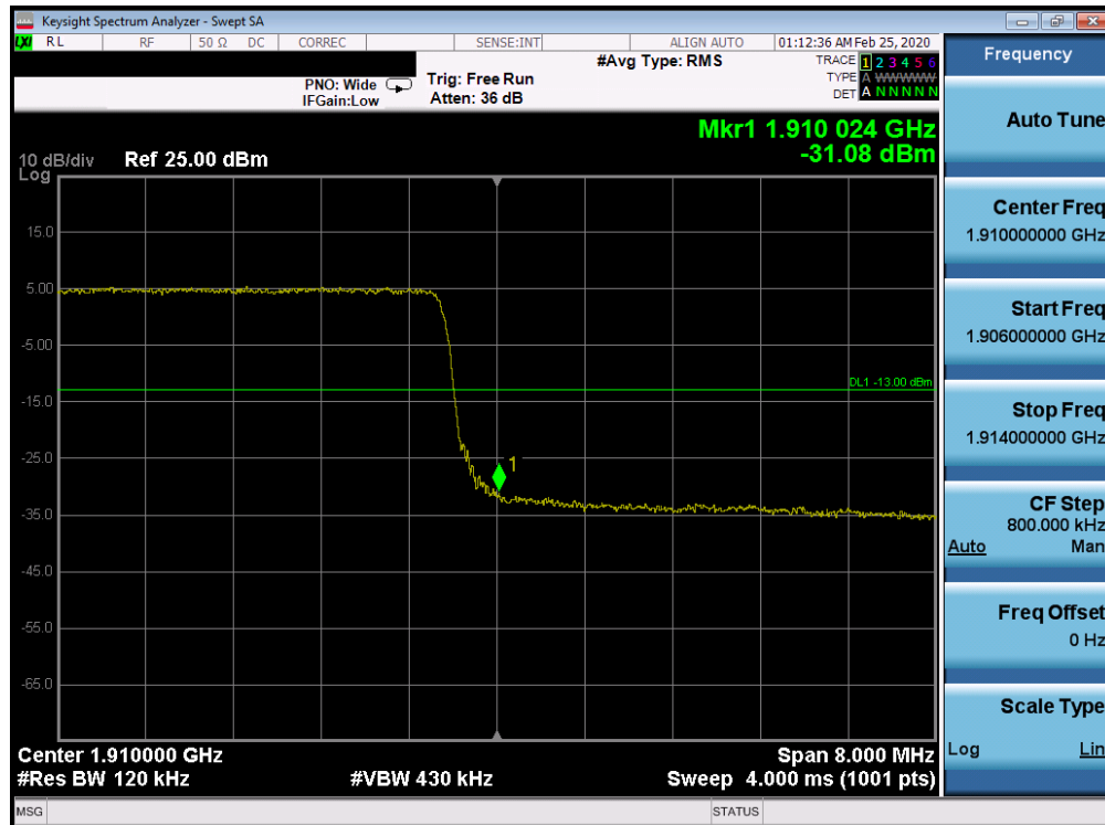
Plot 7-209. Upper Band Edge Plot (Band 2 - 10.0MHz QPSK - Full RB Configuration)
