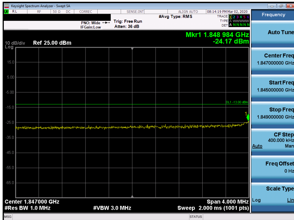
Plot 7-208. Lower Extended Band Edge Plot (Band 25/2 - 10.0MHz QPSK - Full RB Configuration)
