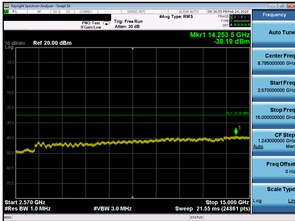
Plot 7-119. Conducted Spurious Plot (Band 7 - 20.0MHz QPSK - RB Size 1, RB Offset 0 - Low Channel)
