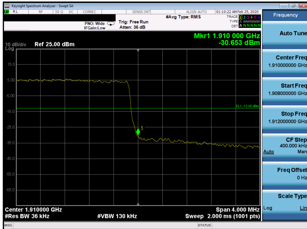
Plot 7-197. Upper Band Edge Plot (Band 2 - 3.0MHz QPSK - Full RB Configuration)
