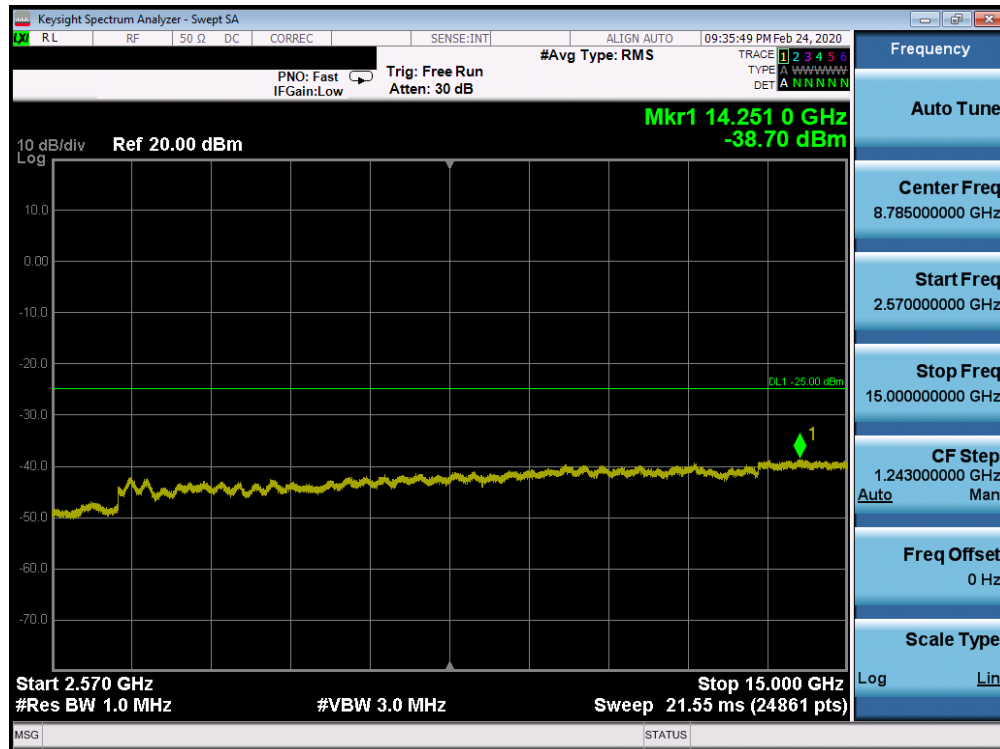
Plot 7-122. Conducted Spurious Plot (Band 7 - 20.0MHz QPSK - RB Size 1, RB Offset 0 - Mid Channel)
