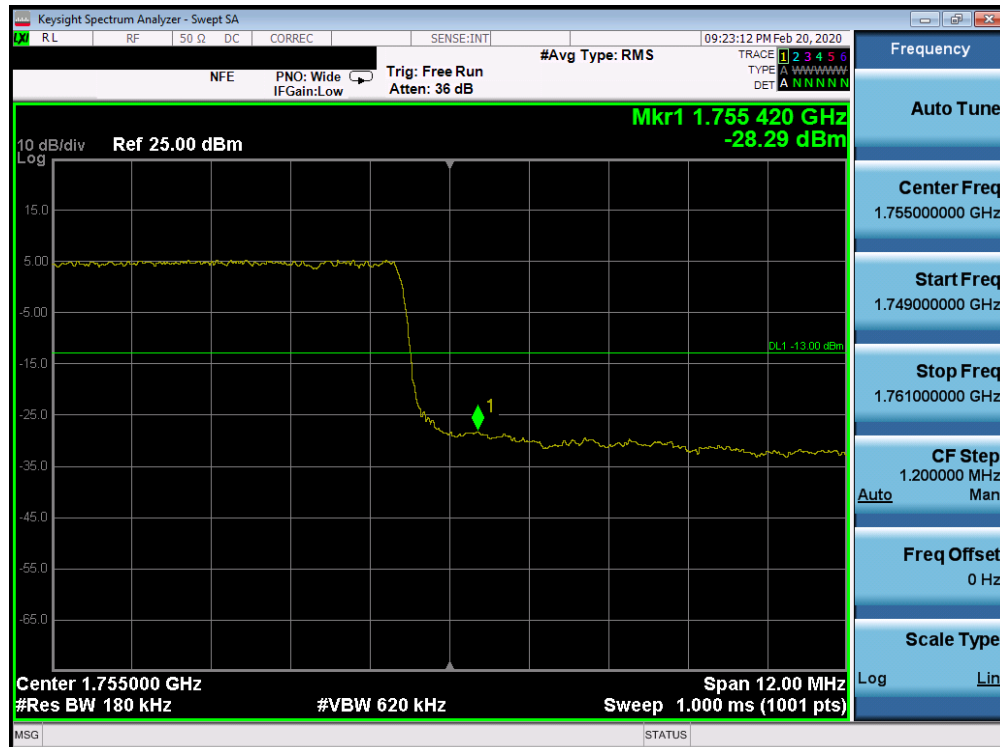
Plot 7-179. Upper Band Edge Plot (Band 4 - 15.0MHz QPSK - Full RB Configuration)
