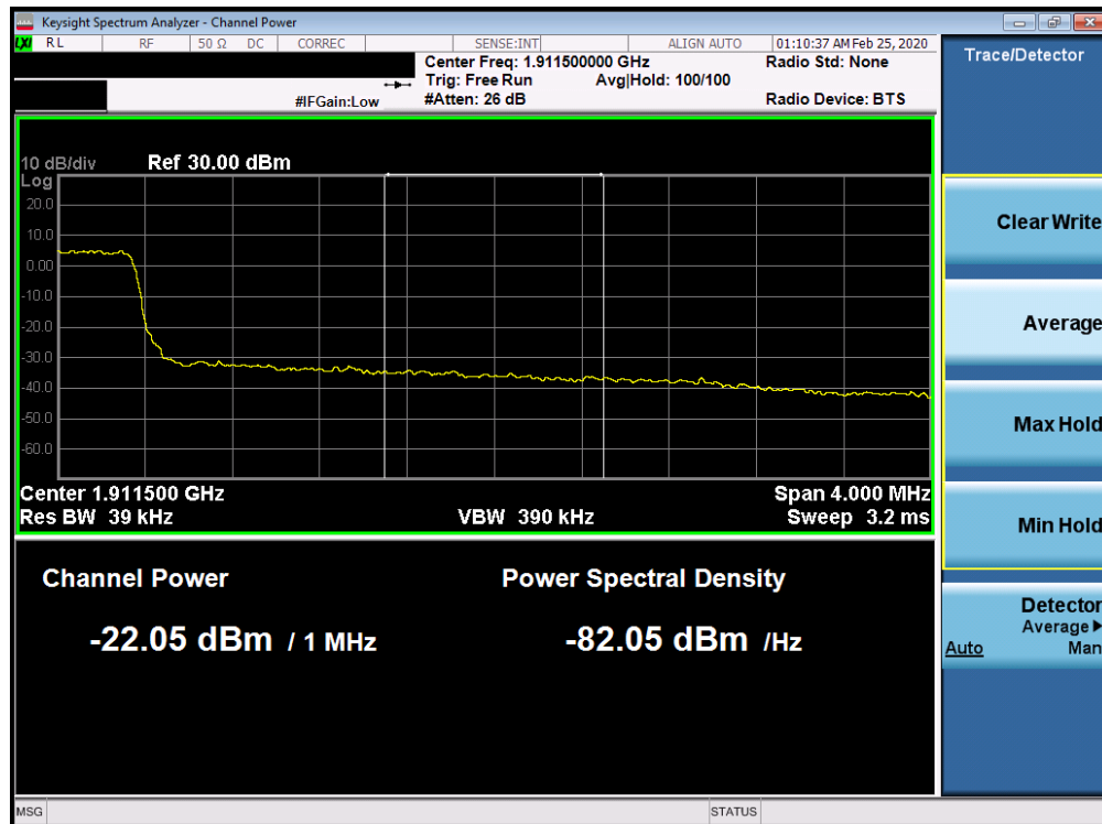
Plot 7-198. Upper Extended Band Edge Plot (Band 2 - 3.0MHz QPSK - Full RB Configuration)
