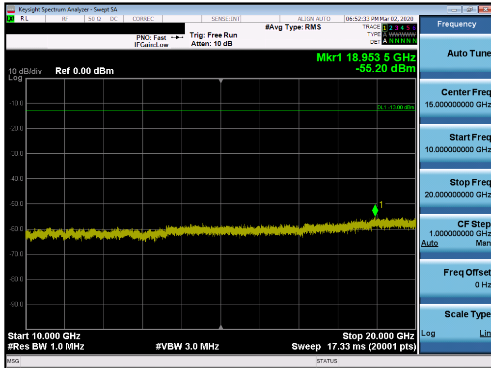
Plot 7-111. Conducted Spurious Plot (Band 25/2 - 20.0MHz QPSK - RB Size 1, RB Offset 0 - Low Channel)
