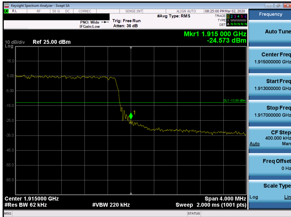
Plot 7-205. Upper Band Edge Plot (Band 25 - 5.0MHz QPSK - Full RB Configuration)
