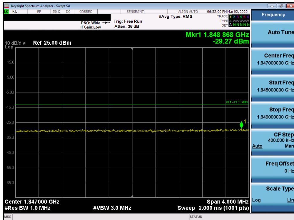
Plot 7-220. Lower Extended Band Edge Plot (Band 25/2 - 20.0MHz QPSK - Full RB Configuration)
