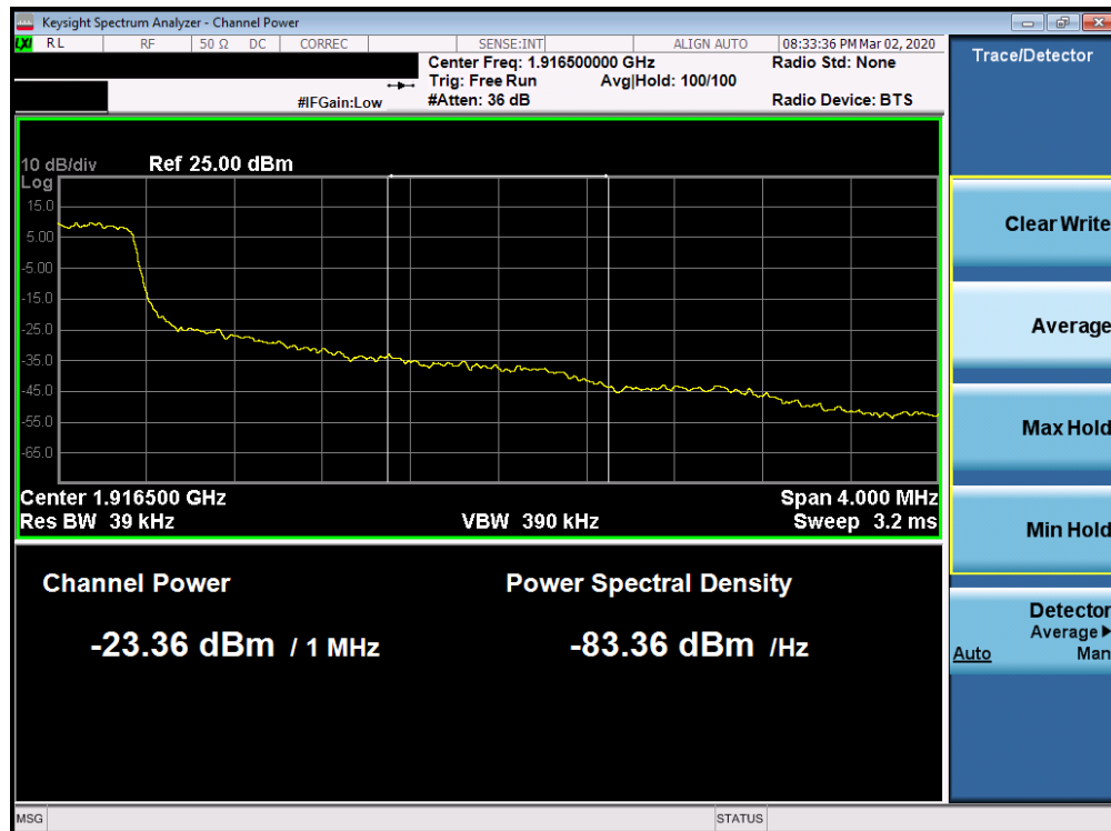
Plot 7-194. Upper Extended Band Edge Plot (Band 25 - 1.4MHz QPSK - Full RB Configuration)
