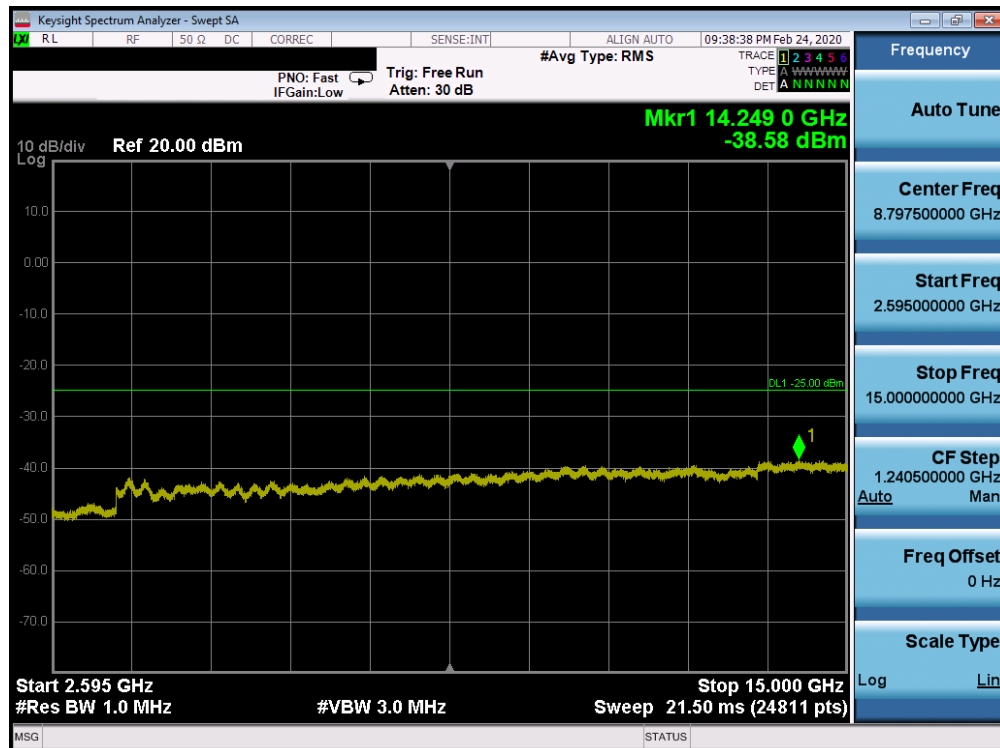
Plot 7-125. Conducted Spurious Plot (Band 7 - 20.0MHz QPSK - RB Size 1, RB Offset 0 - High Channel)
