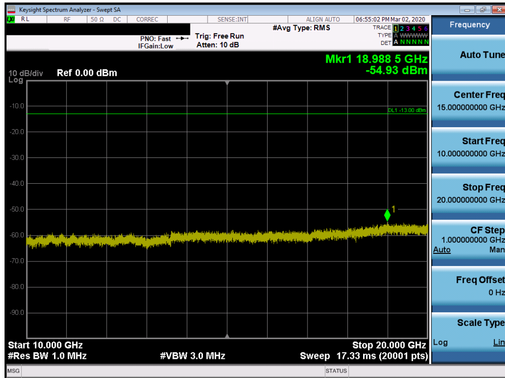
Plot 7-117. Conducted Spurious Plot (Band 25/2 - 20.0MHz QPSK - RB Size 1, RB Offset 0 - High Channel)
