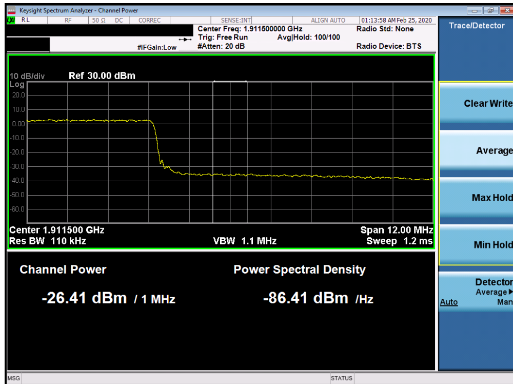
Plot 7-216. Upper Extended Band Edge Plot (Band 2 - 15.0MHz QPSK - Full RB Configuration)
