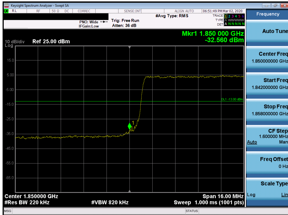
Plot 7-219. Lower Band Edge Plot (Band 25/2 - 20.0MHz QPSK - Full RB Configuration)
