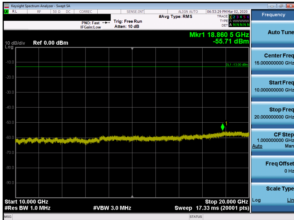
Plot 7-114. Conducted Spurious Plot (Band 25/2 - 20.0MHz QPSK - RB Size 1, RB Offset 0 - Mid Channel)
