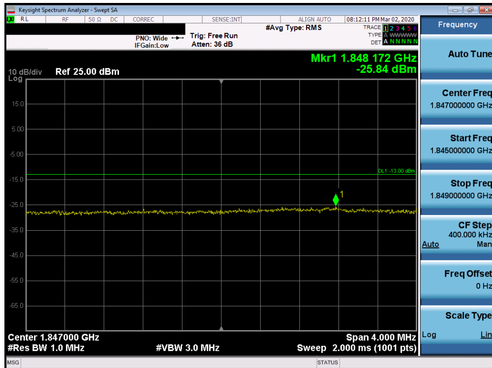
Plot 7-214. Lower Extended Band Edge Plot (Band 25/2 - 15.0MHz QPSK - Full RB Configuration)
