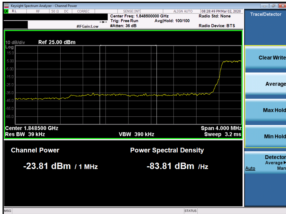
Plot 7-196. Lower Extended Band Edge Plot (Band 25/2 - 3.0MHz QPSK - Full RB Configuration)
