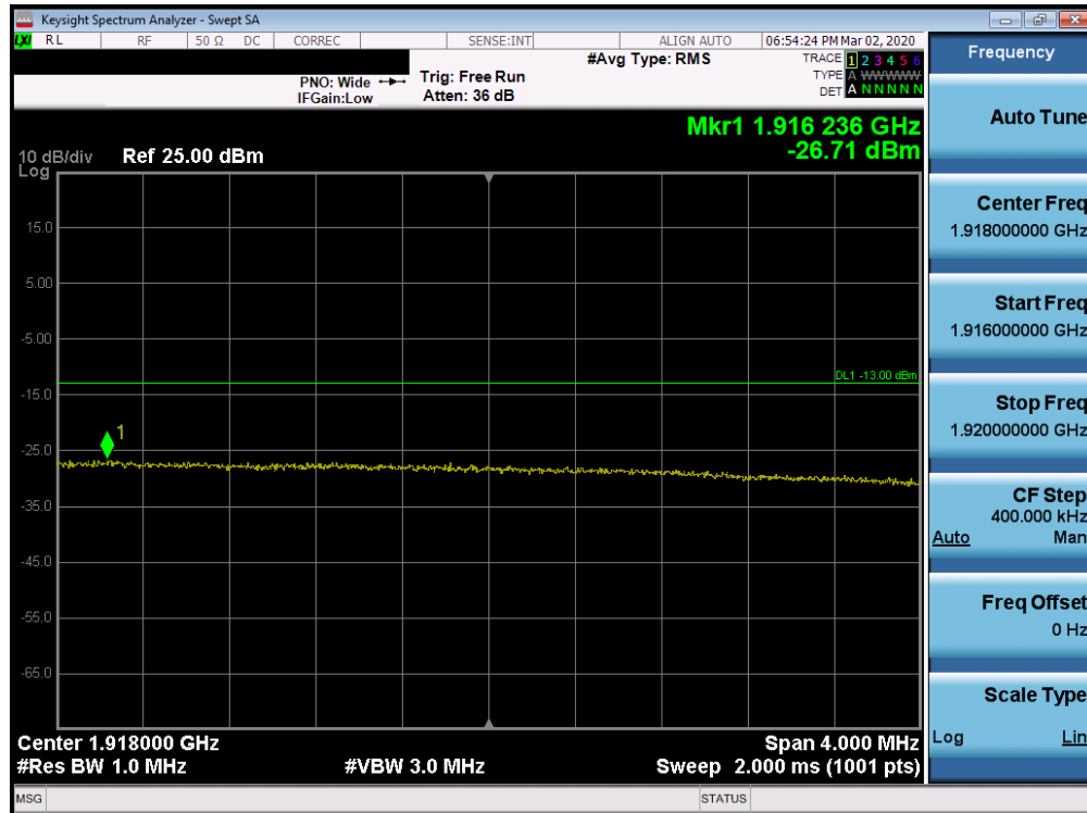
Plot 7-224. Upper Extended Band Edge Plot (Band 25 - 20.0MHz QPSK - Full RB Configuration)
