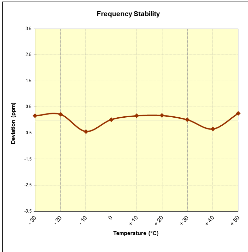
Figure 7-9. Frequency Stability Graph (Cellular GPRS Mode – Ch. 190)
