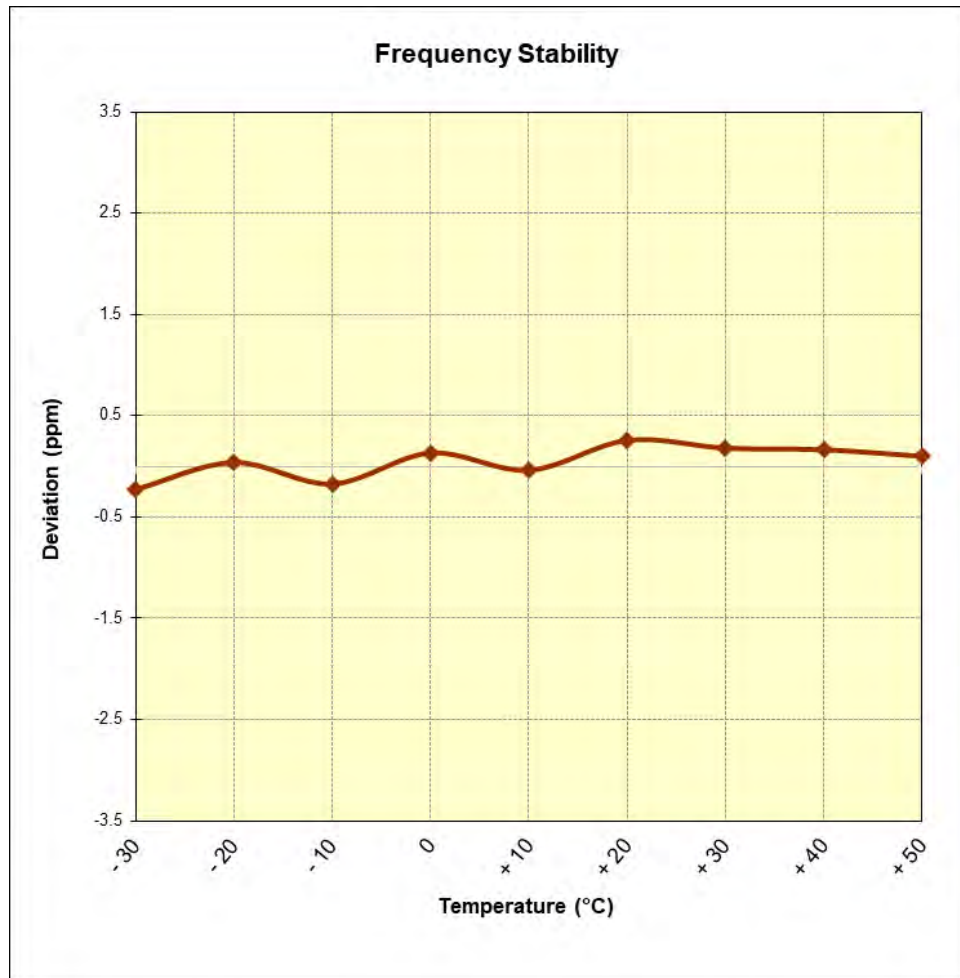
Figure 7-11. Frequency Stability Graph (Cellular WCDMA Mode – Ch. 4183)
