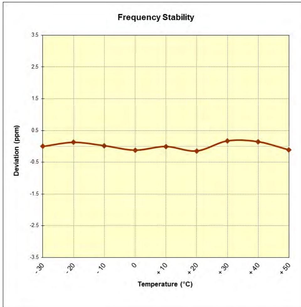
Figure 7-14. Frequency Stability Graph (PCS CDMA Mode – Ch. 600)
