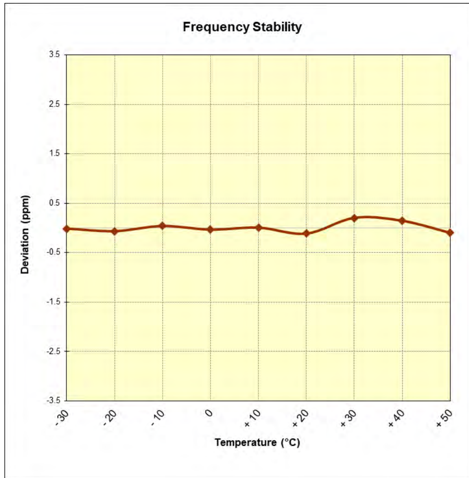
Figure 7-12. Frequency Stability Graph (AWS WCDMA Mode – Ch. 1413)
