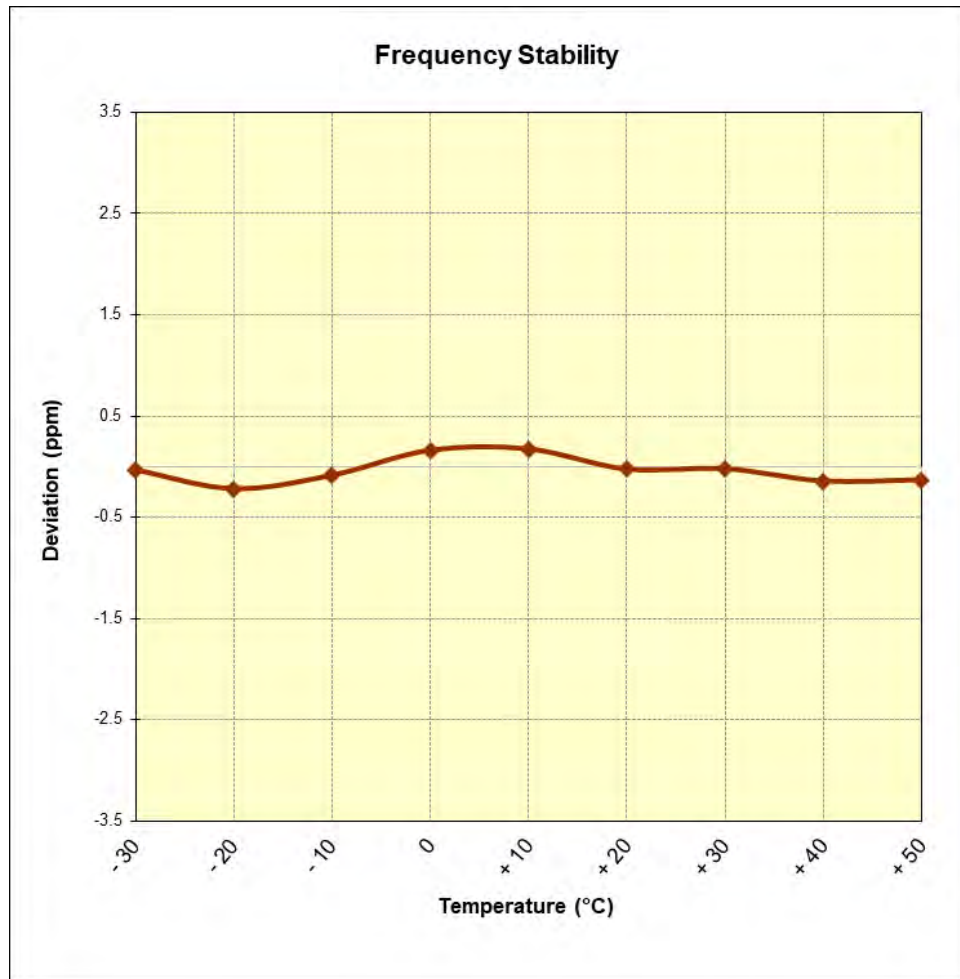
Figure 7-15. Frequency Stability Graph (PCS WCDMA Mode – Ch. 9400)
