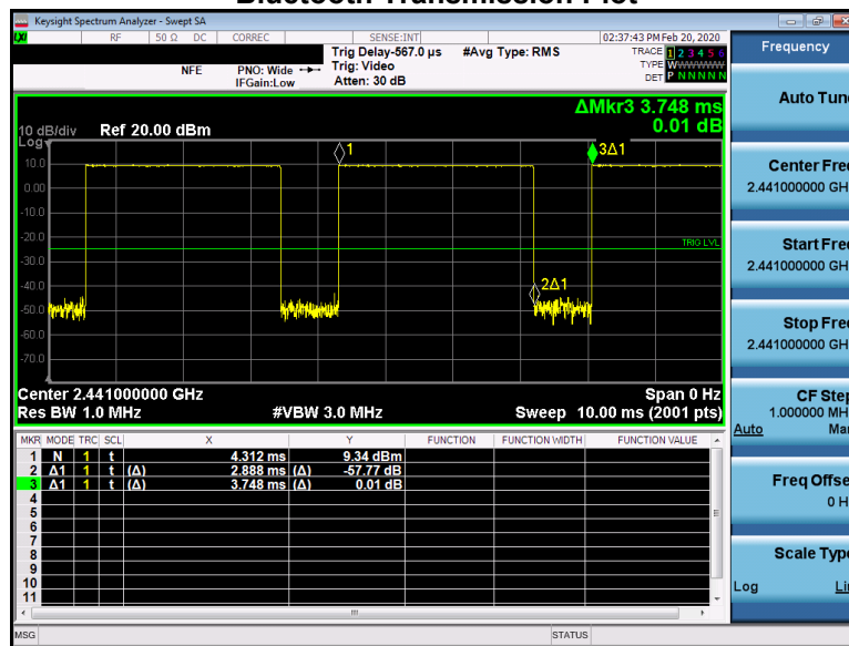
Figure 9-5 Bluetooth Transmission Plot
