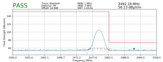
Plot 7-6. Radiated Restricted Upper Band Edge Measurement (Peak)
