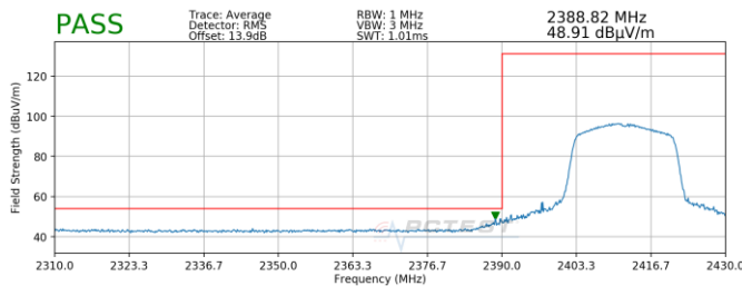
Plot 7-5. Radiated Restricted Lower Band Edge Measurement (Average)
