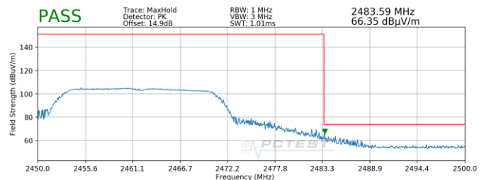
Plot 7-12. Radiated Restricted Upper Band Edge Measurement (Peak)
