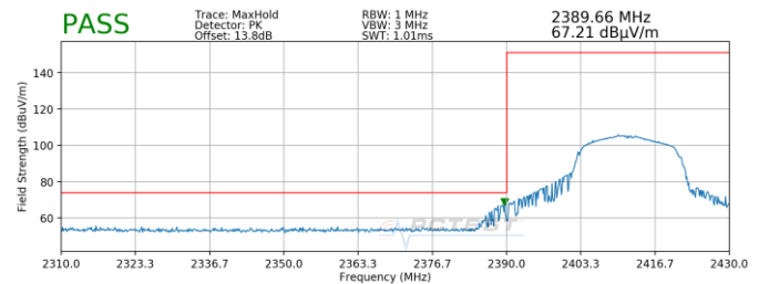
Plot 7-6. Radiated Restricted Lower Band Edge Measurement (Peak)
