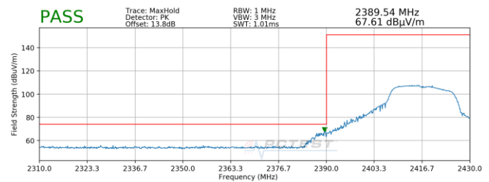
Plot 7-8. Radiated Restricted Lower Band Edge Measurement (Peak)
