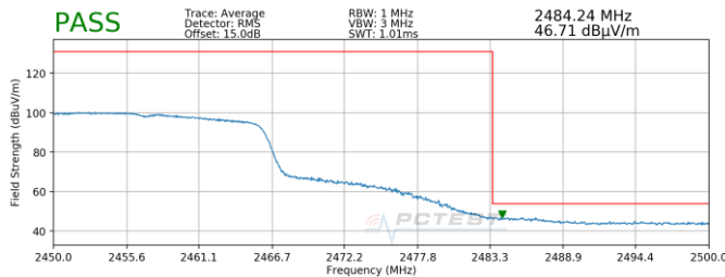
Plot 7-9. Radiated Restricted Upper Band Edge Measurement (Average)
