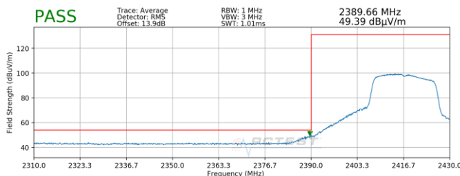
Plot 7-7. Radiated Restricted Lower Band Edge Measurement (Average)
