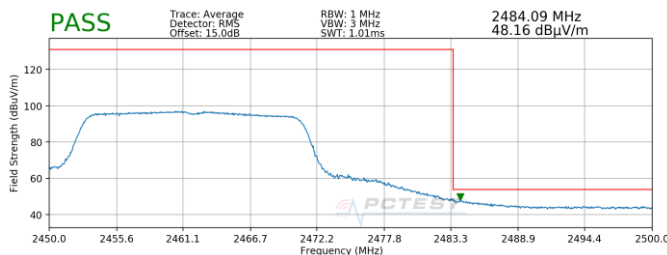
Plot 7-11. Radiated Restricted Upper Band Edge Measurement (Average)
