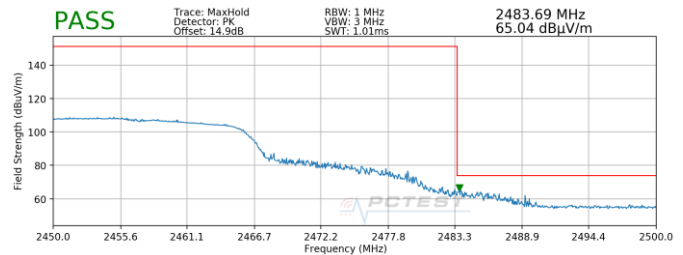
Plot 7-10. Radiated Restricted Upper Band Edge Measurement (Peak)
