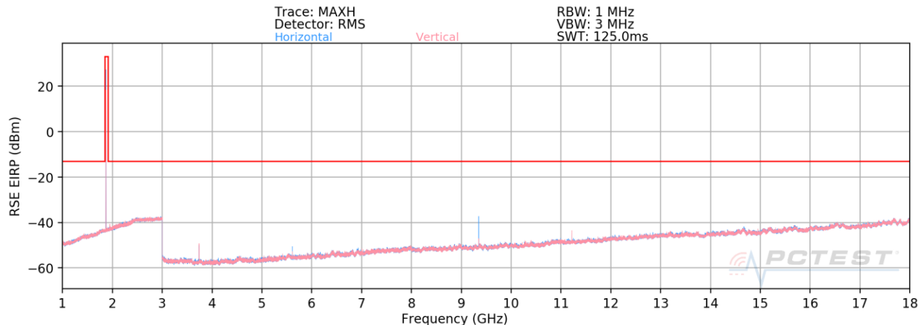
Plot 7-4. Radiated Spurious Plot above 1GHz (PCS GPRS Mode)
