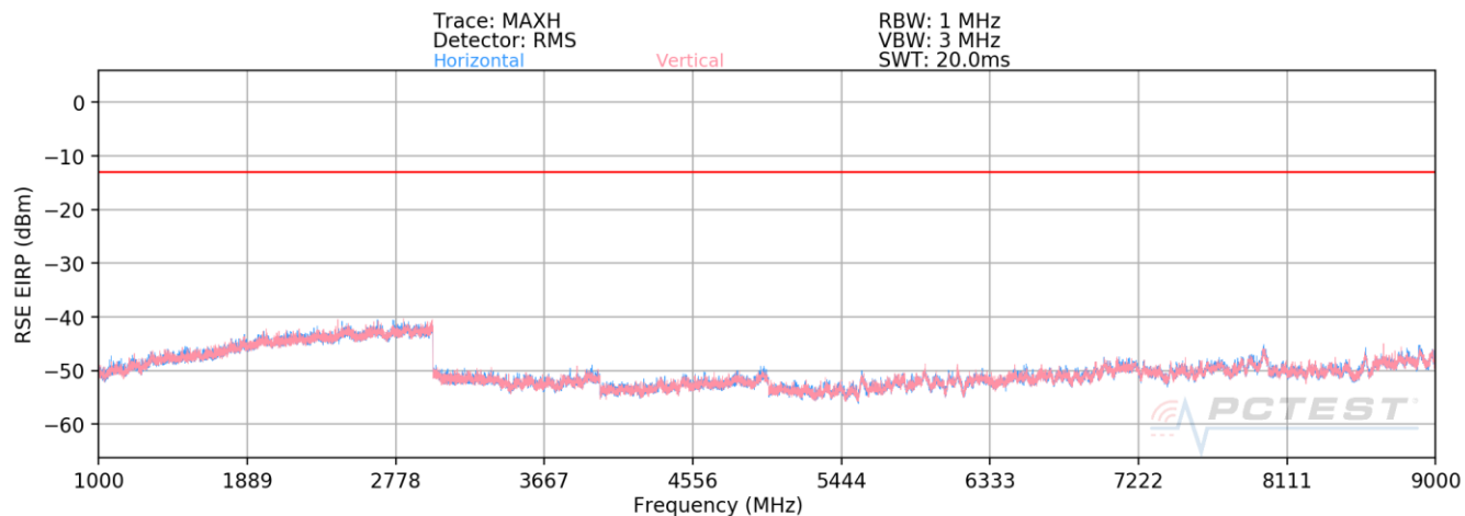
Plot 7-2. Radiated Spurious Plot above 1GHz (Cellular WCDMA Mode)
