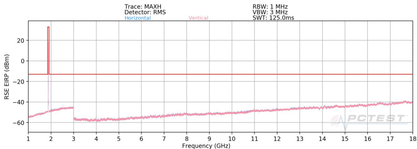
Plot 7-5. Radiated Spurious Plot above 1GHz (PCS WCDMA Mode)
