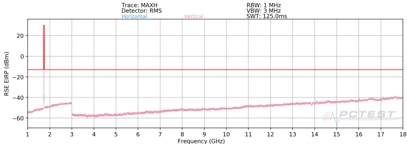
Plot 7-3. Radiated Spurious Plot above 1GHz (AWS WCDMA Mode)
