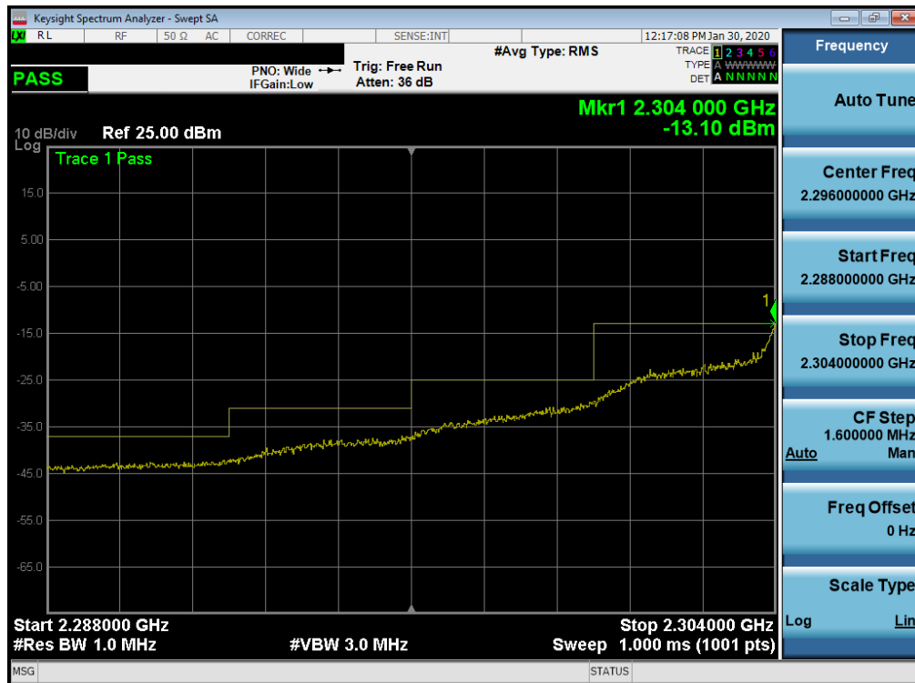
Plot 7-149. Lower Extended Band Edge Plot (Band 30 - 5.0MHz QPSK - Full RB Configuration)
