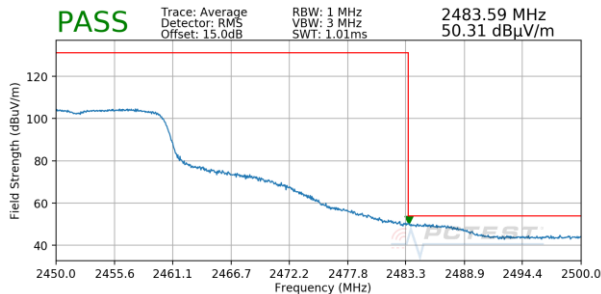
Plot 7-41. Radiated Restricted Upper Band Edge Measurement (Average)
