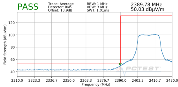
Plot 7-35. Radiated Restricted Lower Band Edge Measurement (Average)
