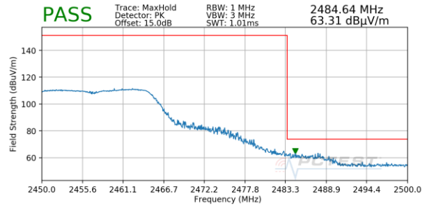
Plot 7-44. Radiated Restricted Upper Band Edge Measurement (Peak)
