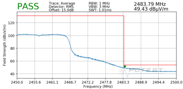
Plot 7-43. Radiated Restricted Upper Band Edge Measurement (Average)
