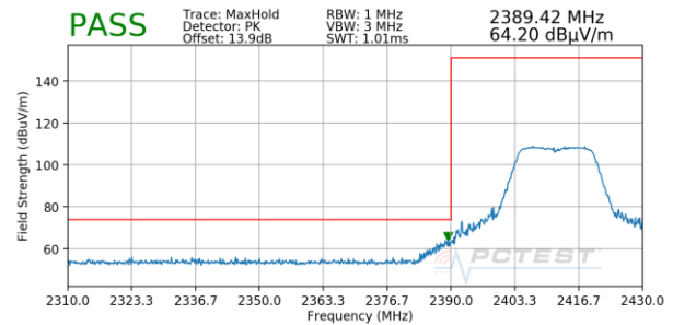
Plot 7-36. Radiated Restricted Lower Band Edge Measurement (Peak)
