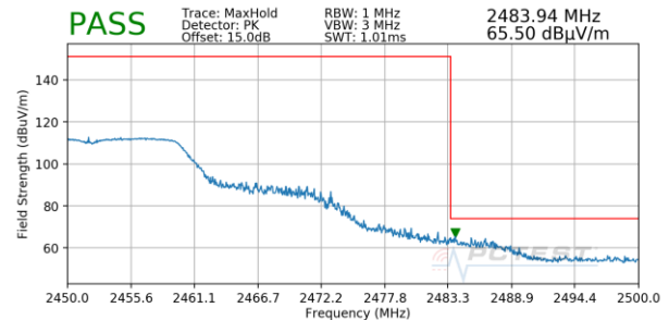
Plot 7-42. Radiated Restricted Upper Band Edge Measurement (Peak)
