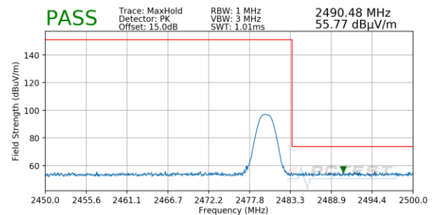
Plot 7-19. Radiated Restricted Upper Band Edge Measurement (Peak)
