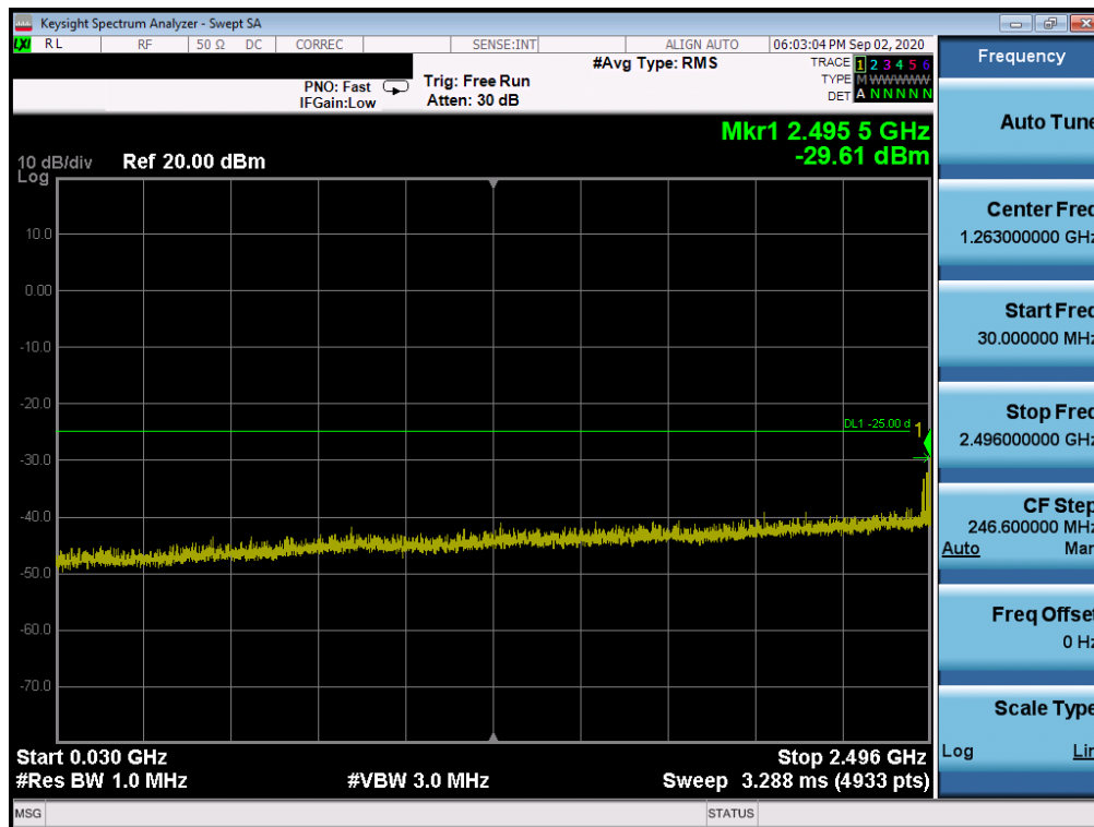
Plot 7-16. Conducted Spurious Plot (LTE Band 41(PC2) - 20MHz QPSK - RB Size 1, RB Offset 0 - Mid Channel)
