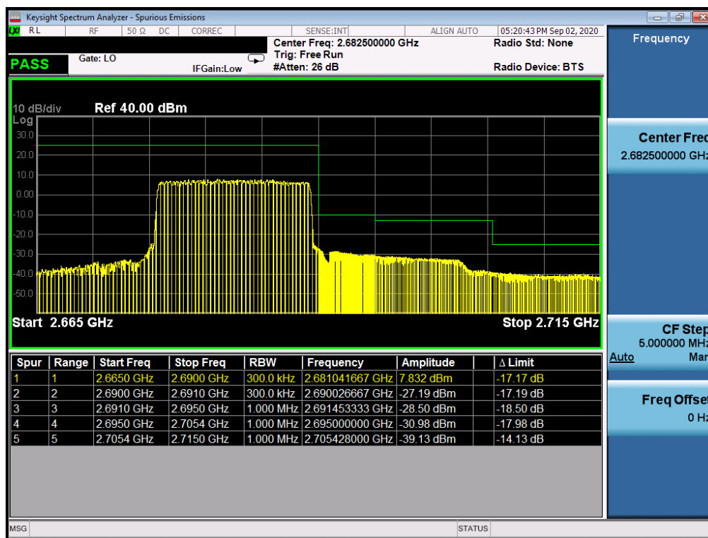
Plot 7-25. Upper ACP Plot (LTE Band 41(PC2) - 15MHz QPSK - Full RB Configuration)
