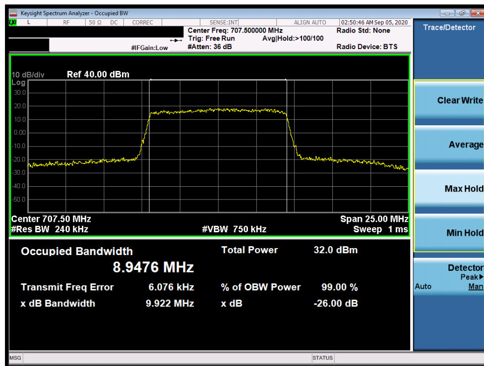
Plot 7-14. Occupied Bandwidth Plot (LTE Band 12 - 10MHz 16-QAM - Full RB Configuration)
