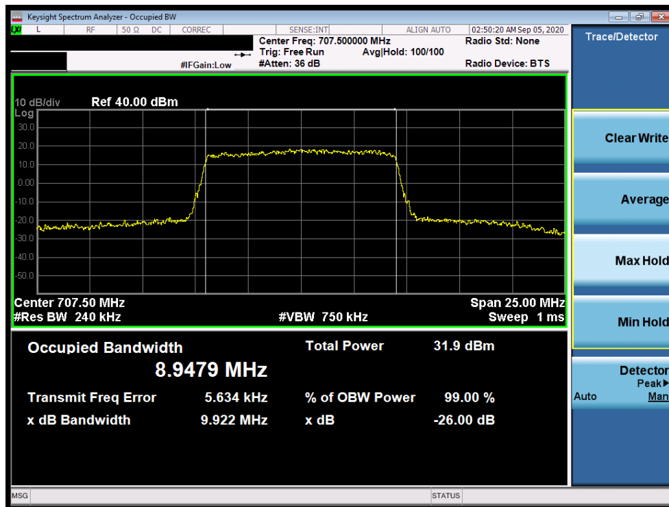
Plot 7-13. Occupied Bandwidth Plot (LTE Band 12 - 10MHz QPSK - Full RB Configuration)
