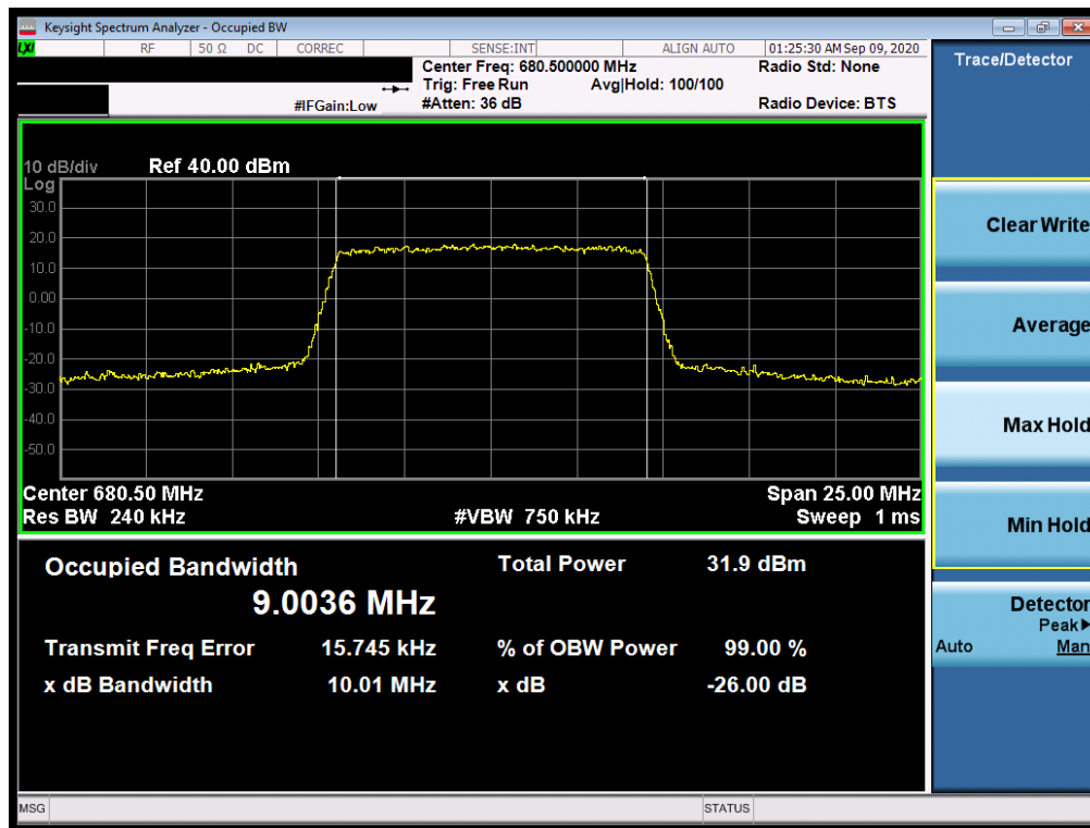
Plot 7-7. Occupied Bandwidth Plot (LTE Band 71 - 10MHz QPSK - Full RB Configuration)
