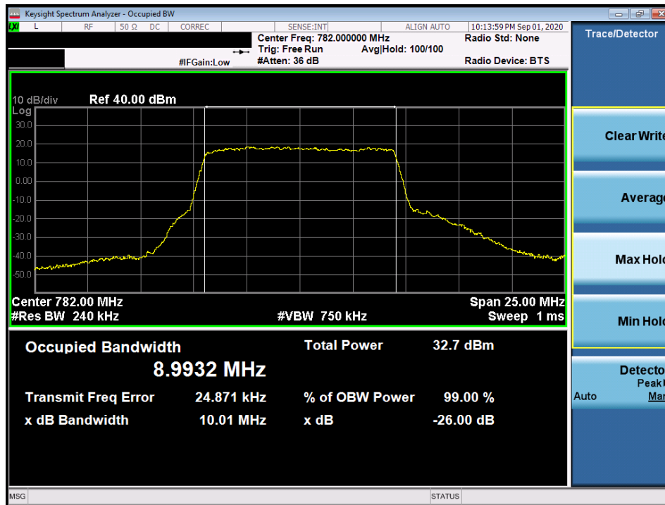
Plot 7-25. Occupied Bandwidth Plot (LTE Band 13 - 10MHz QPSK - Full RB Configuration)
