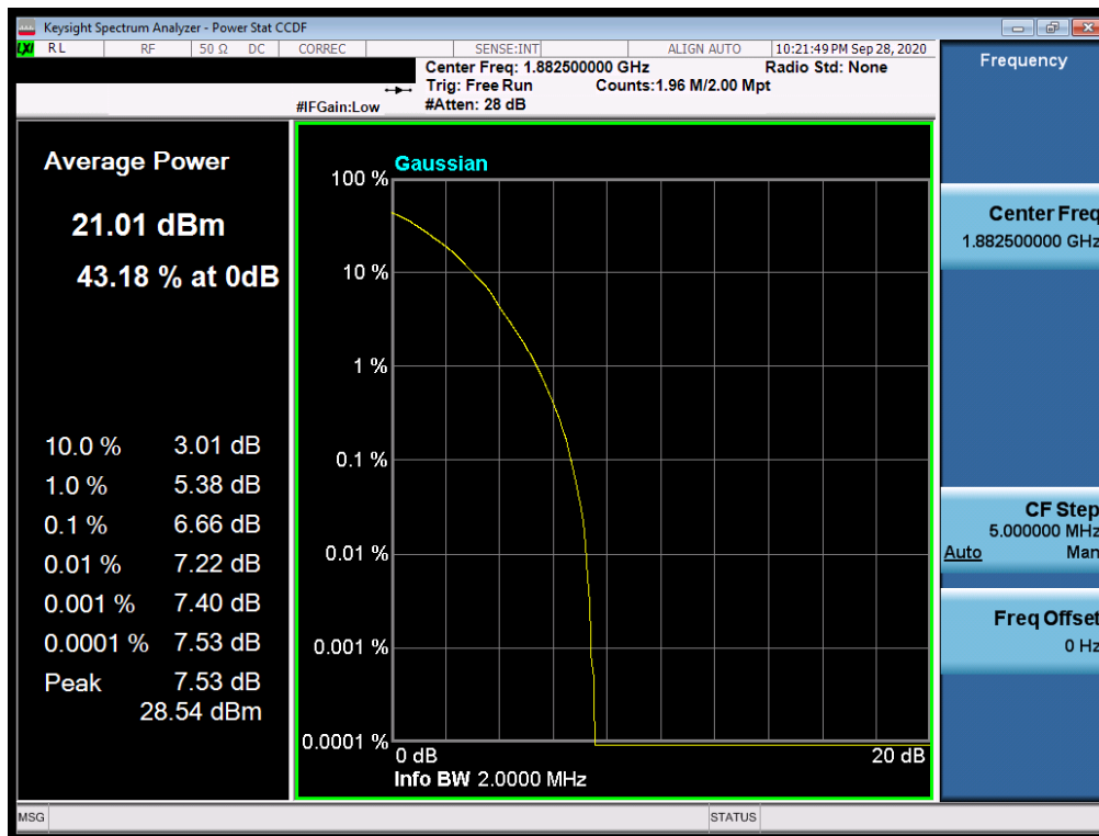
Plot 7-116. PAR Plot (LTE Band 25/2 - 1.4MHz 64-QAM - Full RB Configuration)
