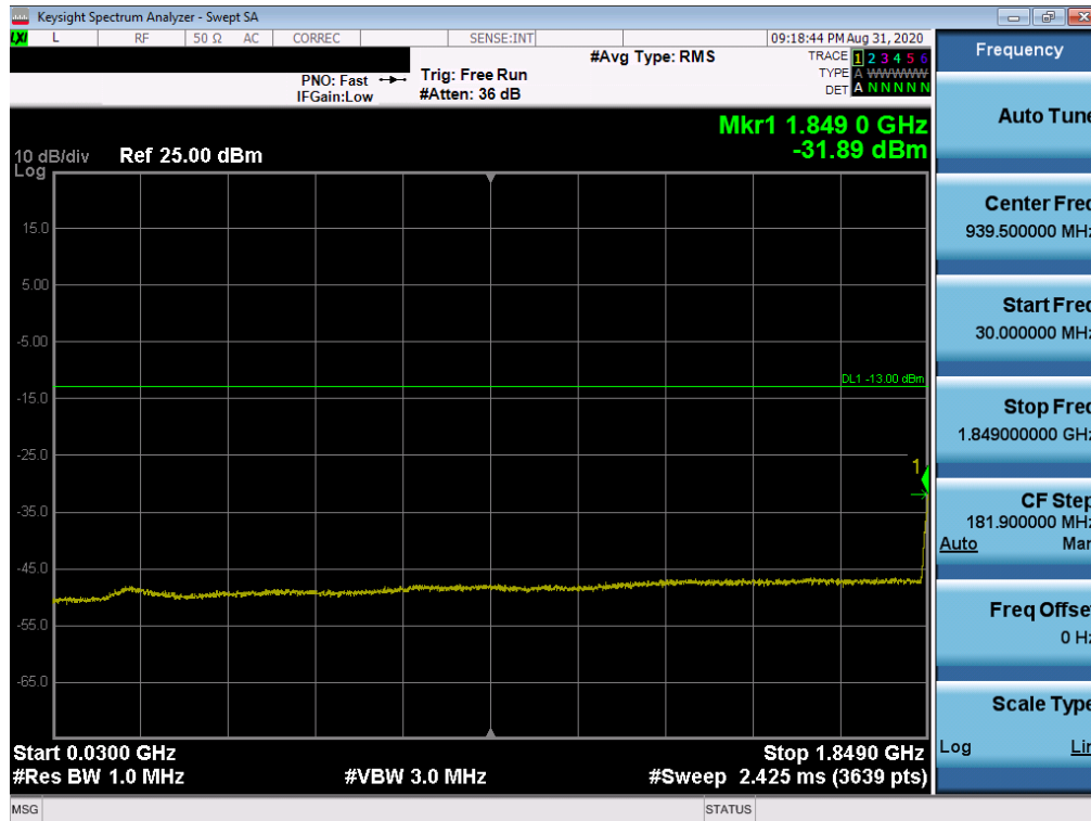
Plot 7-22. Conducted Spurious Plot (LTE Band 25/2 - 20MHz QPSK - RB Size 1, RB Offset 0 - Low Channel)
