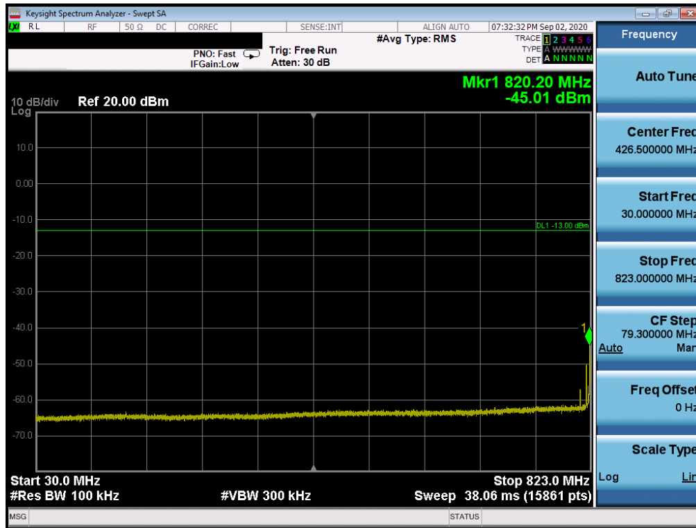
Plot 7-19. Conducted Spurious Plot (LTE Band 26/5 - 10MHz QPSK - RB Size 1, RB Offset 0 - Low Channel)
