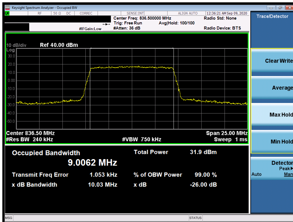
Plot 7-4. Occupied Bandwidth Plot (LTE Band 26/5 - 10MHz QPSK - Full RB Configuration)
