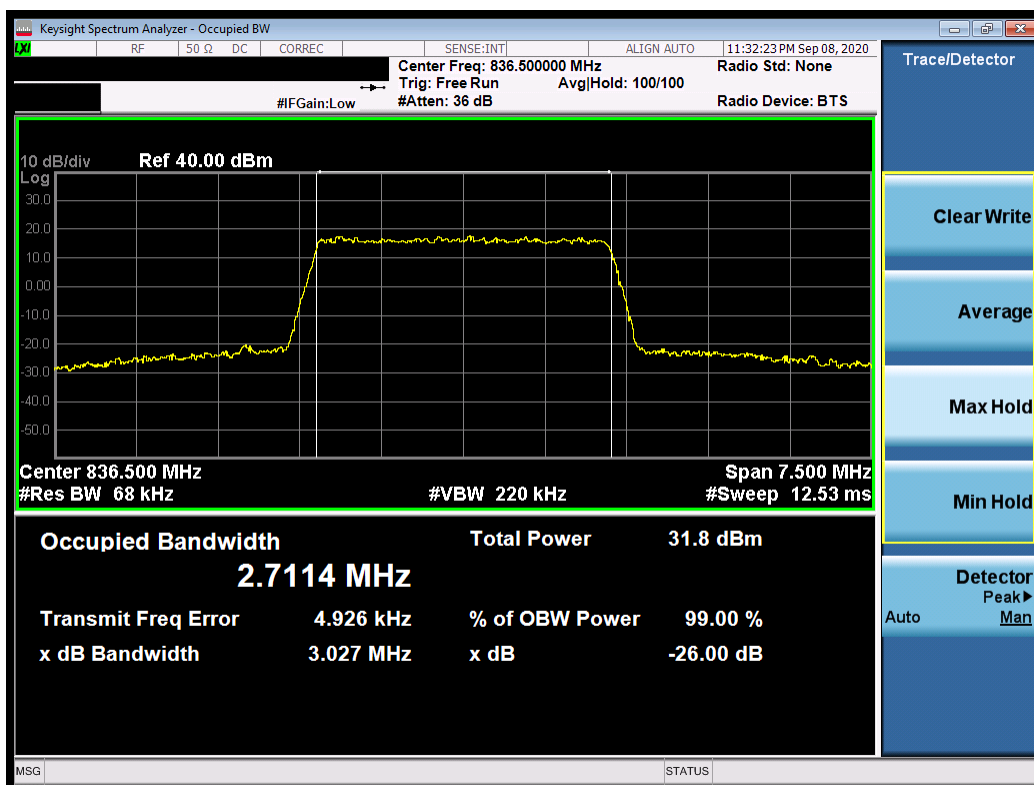
Plot 7-10. Occupied Bandwidth Plot (LTE Band 26/5 - 3MHz QPSK - Full RB Configuration)
