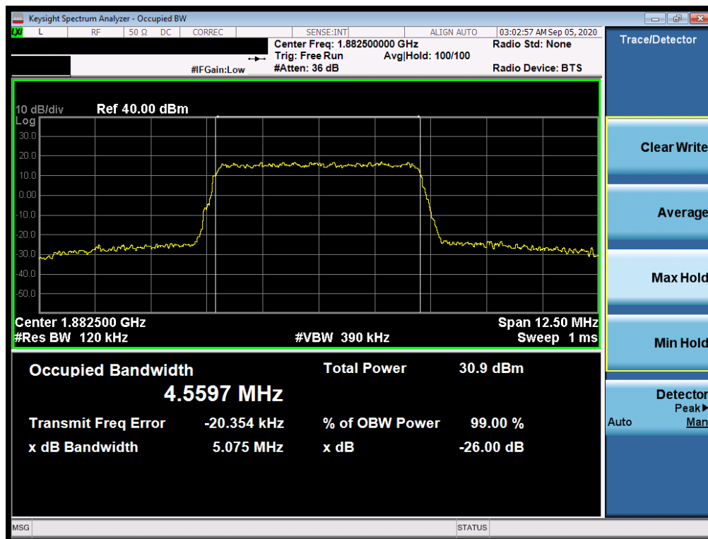
Plot 7-11. Occupied Bandwidth Plot (LTE Band 25/2 - 5MHz 16-QAM - Full RB Configuration)
