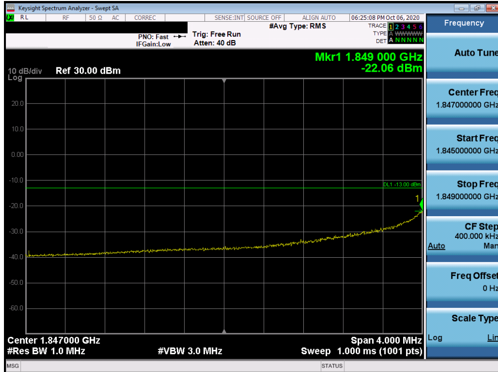
Plot 7-33. Extended Lower Band Edge Plot (CDMA PCS – Ch. 25)
