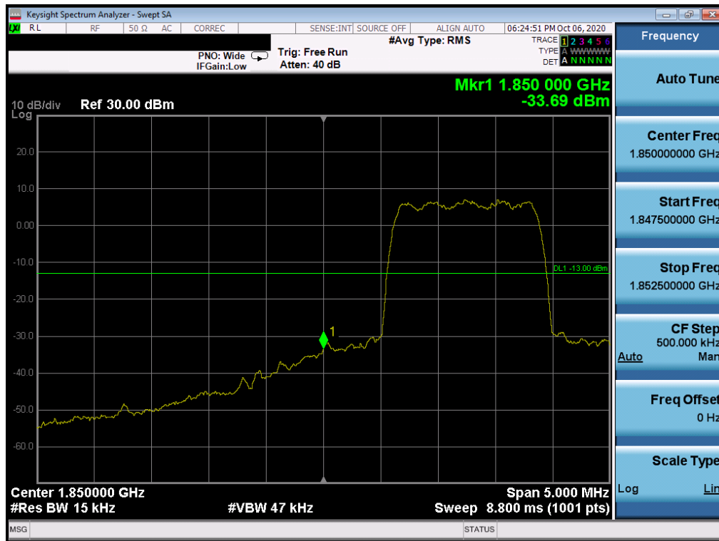
Plot 7-32. Lower Band Edge Plot (CDMA PCS – Ch. 25)
